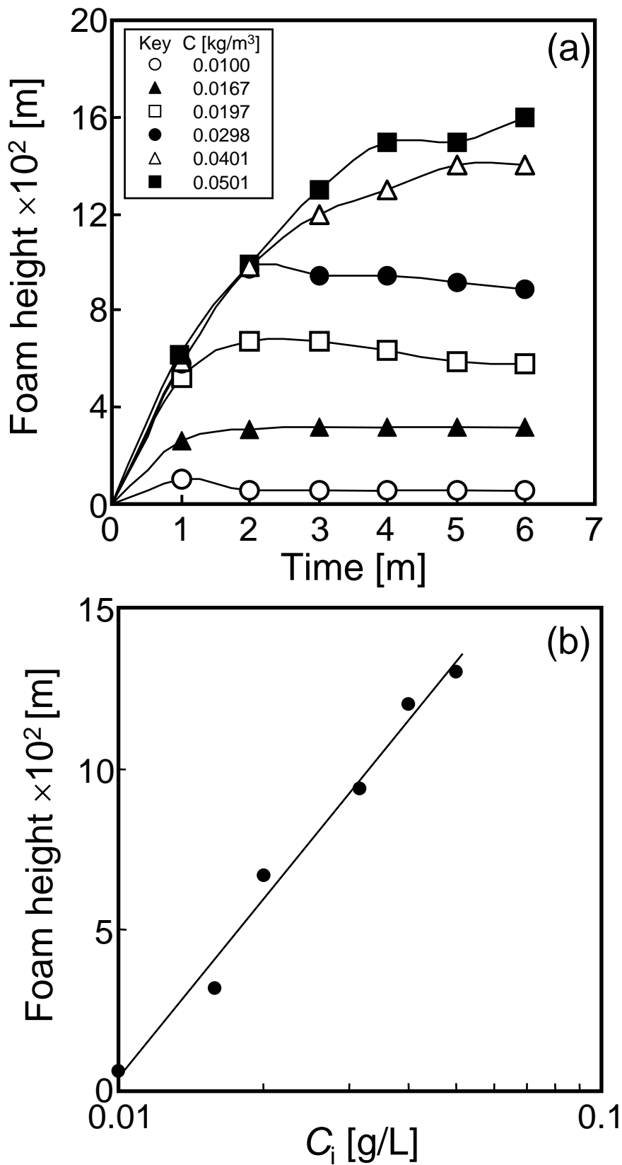
Fig. 6. (a) Change in foam height within the column for ovalbumin in foaming ability experiments at pH 4.6. (b) Variation of foam height at 3 min after aeration with the initial concentration of OA solution. The solid line is calculated by the least squares regression.
