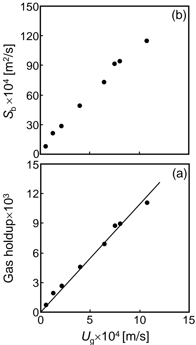
Fig. 4. (a) Change in gas holdup with superficial gas velocity, U_g . The solid line was calculated by a least square regression. (b) Variation of bubble surface area production rate, S_b , with superficial gas velocity, U_g . The values were calculated from Eq. (2).
