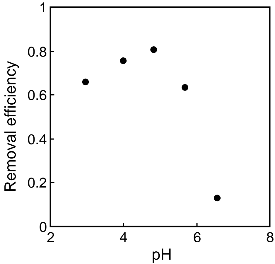
Fig. 2. Influence of pH on removal efficiency of ovalbumin (OA) by batch wise foam separation. The initial concentration of OA was 3.68 \times 10^{-2} \text{ kg/m}^3 and superficial gas velocity is 5.37 \times 10^{-4} \text{ m/s} .
