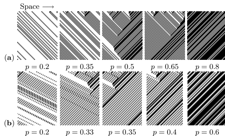
Fig. 1. Typical orbits of traffic models. Initial distribution of “1” is denoted by p . (a) ECA184. (b) EBCA1
