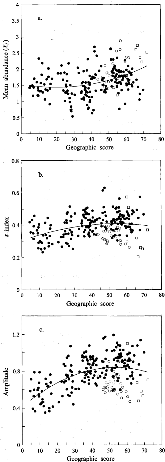
Fig. 5. The relationship between three statistics of population dynamics and geographic score. (a) mean abundance ( \bar{X}_t ), (b) temporal variability ( s -index) and (c) amplitude. Solid circle: 186 populations for Groups 2, 3, 4, 5, 6, 7, 8, 9 and 10; open circle: 31 populations for Group 1; open square: 8 populations for Group 11.
