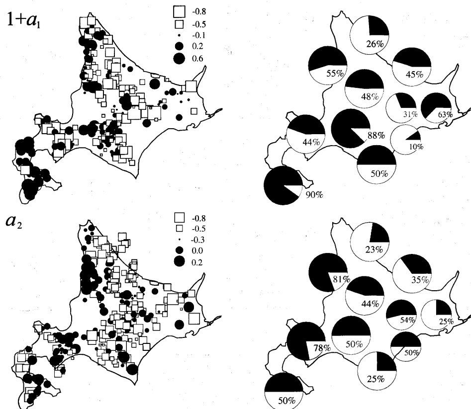
Fig. 7. First order ( (1+a_1) ; upper-left) and second order ( a_2 ; lower-left) autoregressive coefficients of the 225 time series plotted at their spatial co-ordinates. Positive estimates are represented by filled circles, negative estimates are represented by open squares. The size of the symbol is proportional to the absolute value of the estimate. The pie-charts represent the proportion (percentage) of time series in each group having higher values than the grand average (upper-right: (1+a_1) , grand average = -0.13 ; lower-right: a_2 , grand average = -0.29 ).
