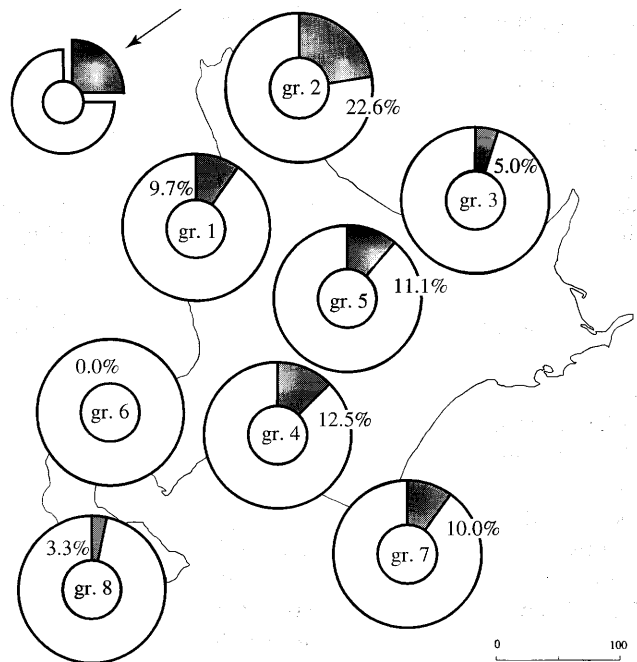
Fig. 6. Proportion of delayed density-dependent populations for each group. Groups 9, 10 and 11 were omitted because of the short length of these time series.
