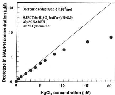
Fig. 6. Relationship between HgCl_2 concentration and decrease in NADPH concentration.
