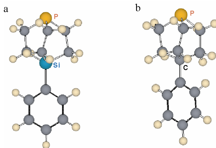
Figure 4. Optimized structures of Ph-SMAP (C-P-C angle 99.7°), (a) and 13 (C-P-C angle 96.2°), (b).
