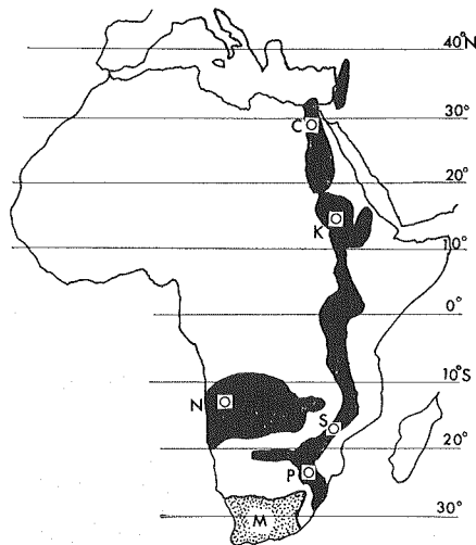
Fig. 3. Distribution of Salix safsaf and the site of collection
