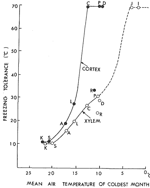
Fig. 4. Freezing tolerance of primitive willow associated with winter cold of their native habitats.
