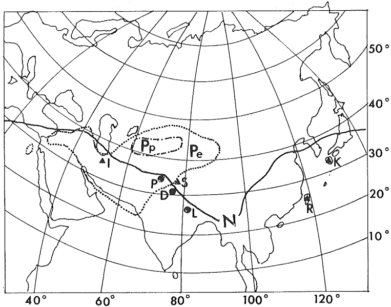
Fig. 2. Distribution of Salix subgen. Protitea in Asia and Central Asia.
