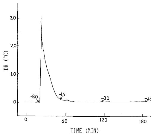
Fig. 5. DTA profile of winter twig piece of Salix tetrasperma from Dehra Dun
