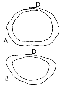
Fig. 1. Comparison of bud scale of willows (4)
