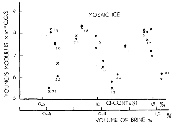
Fig. 11. Relation between Young's modulus of sea ice and chlorine content at -15^{\circ}\text{C} (mosaic ice).
