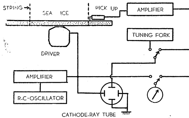
Fig. 2. Block diagram of Young's modulus meter.
