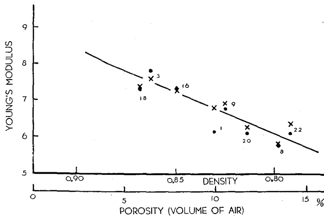
Fig. 14. Relation between Young's modulus and density at -15^{\circ}\text{C} (granular ice).
