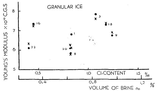
Fig. 12. Relation between Young's modulus of sea ice and chlorine content at -15^{\circ}\text{C} (granular ice).
