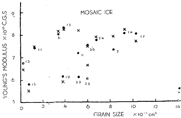
Fig. 9. Relation between Young's modulus of sea ice at -15^{\circ}\text{C} and grain size (mosaic ice).
