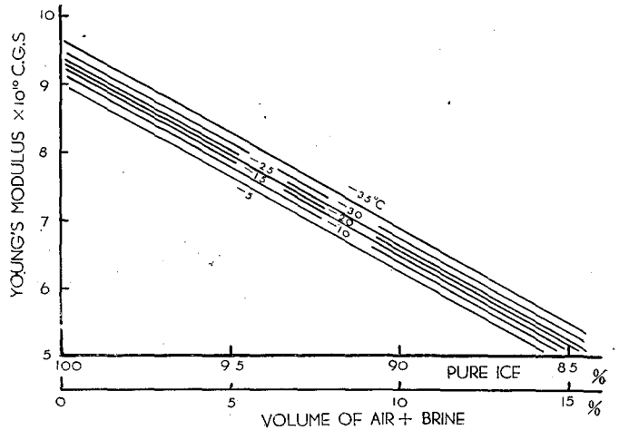
Fig. 19. Relation between Young's modulus of sea ice and volume of pure ice at various temperatures (mosaic ice).
