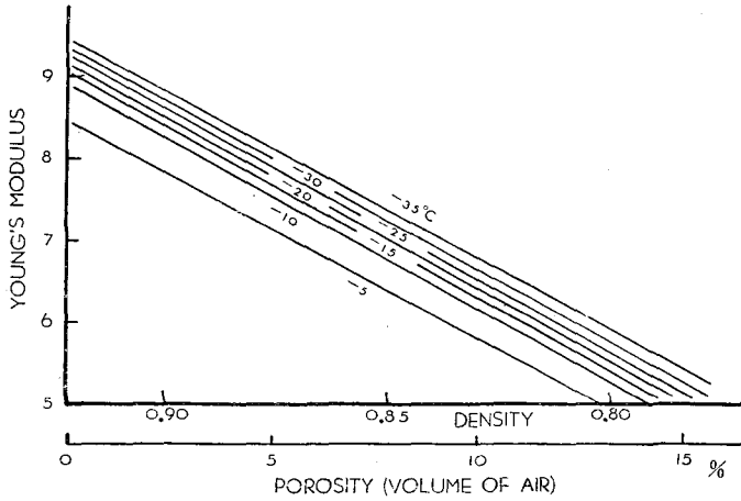
Fig. 15. Relation between Young's modulus of sea ice and density at various temperatures (mosaic ice).
