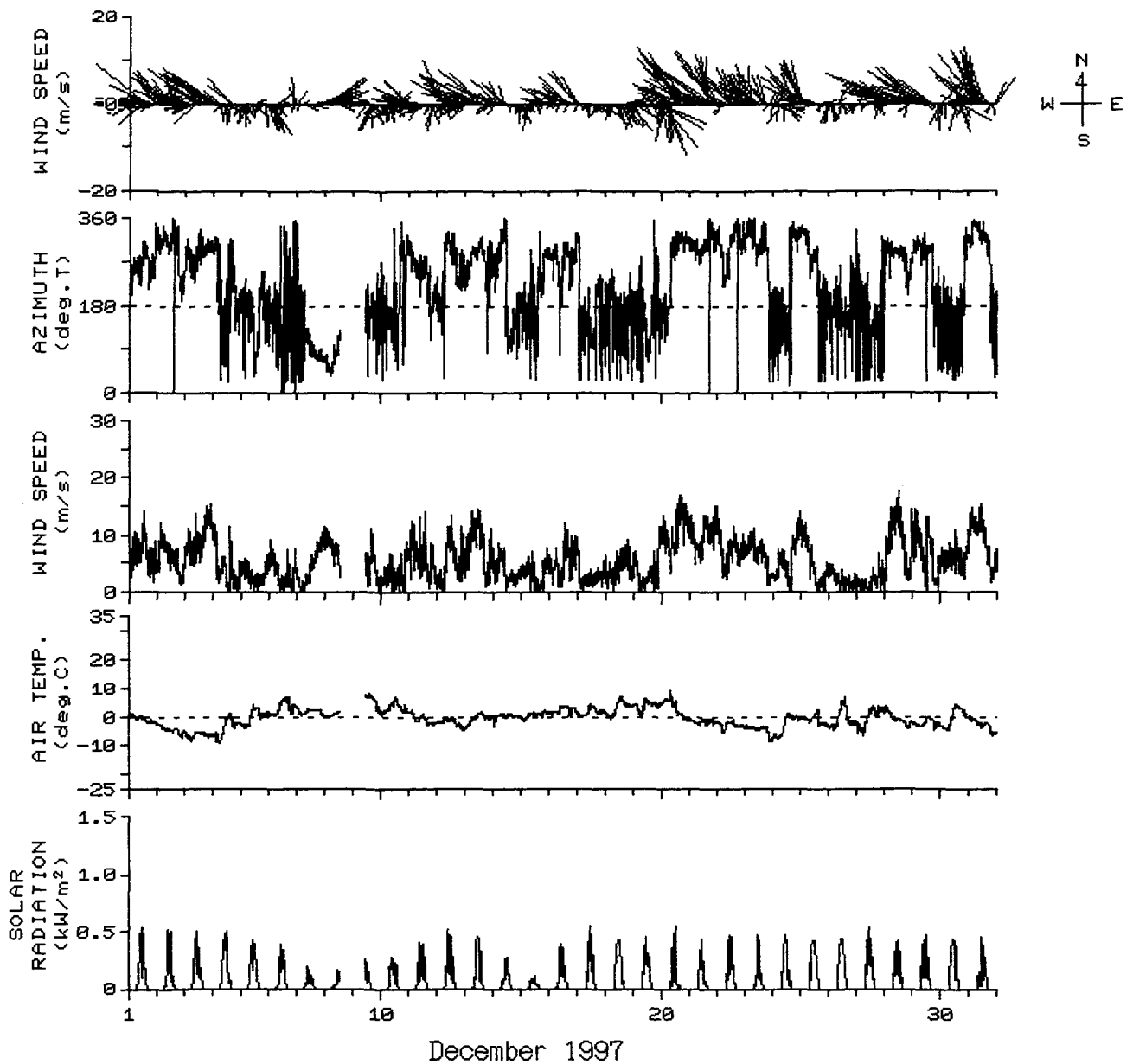
Fig. 3 Wind speed and azimuth, air temperature and solar radiation obtained during the period between December 1997 and November 1998 at Kimuaneppu.
