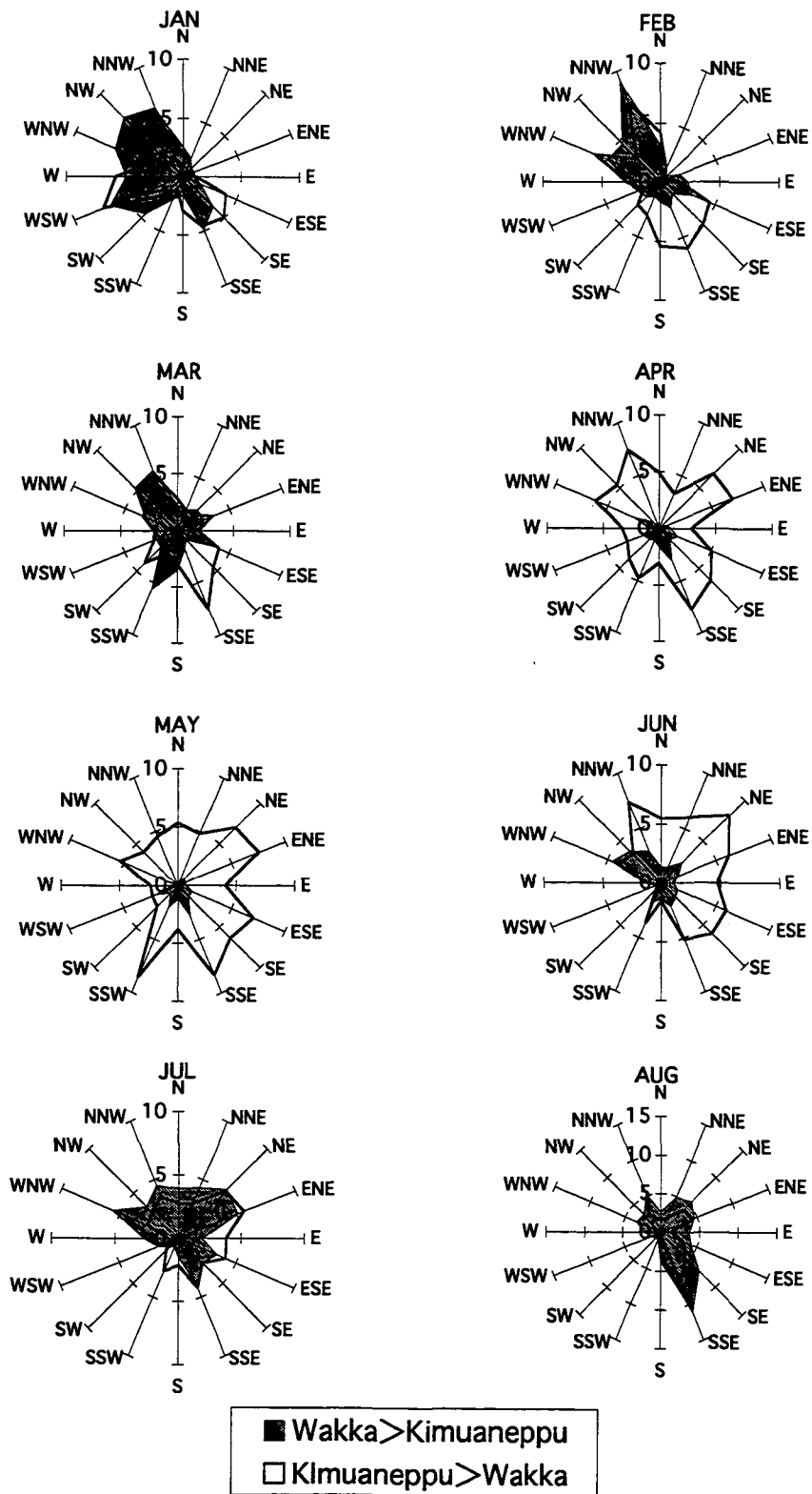
Fig. 5 Monthly wind direction dependency of frequency of the higher air temperature at Wakka (solid line) and the higher air temperature at Kimuanepu (broken line) integrated for the period from 1995 to 1998. The wind direction is the one observed at Wakka.
