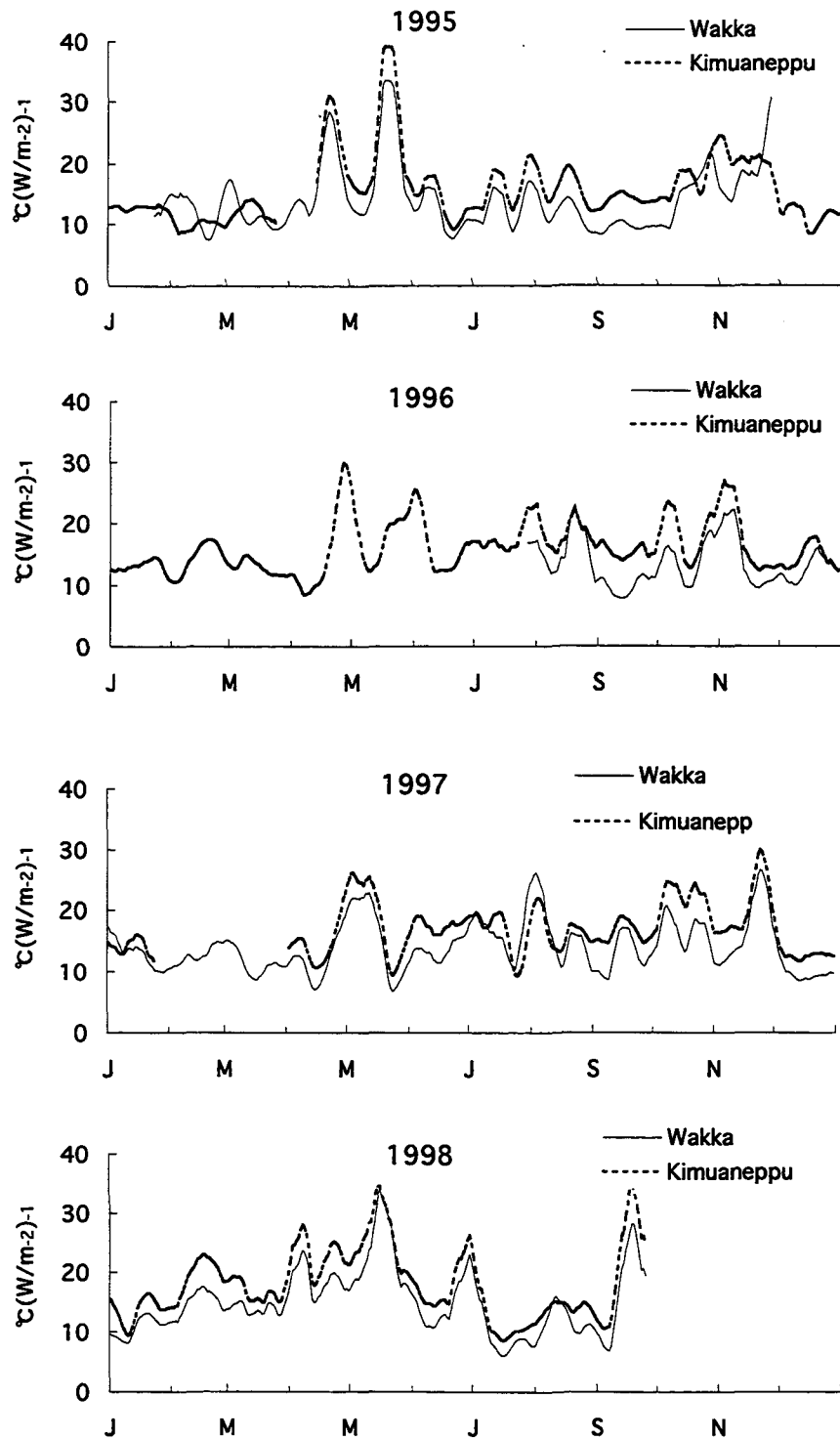
Fig. 6 Time series climatic sensitivity of at Wakka (solid line) and Kimuaneppu (broken line) for the years from 1995 to 1998.
