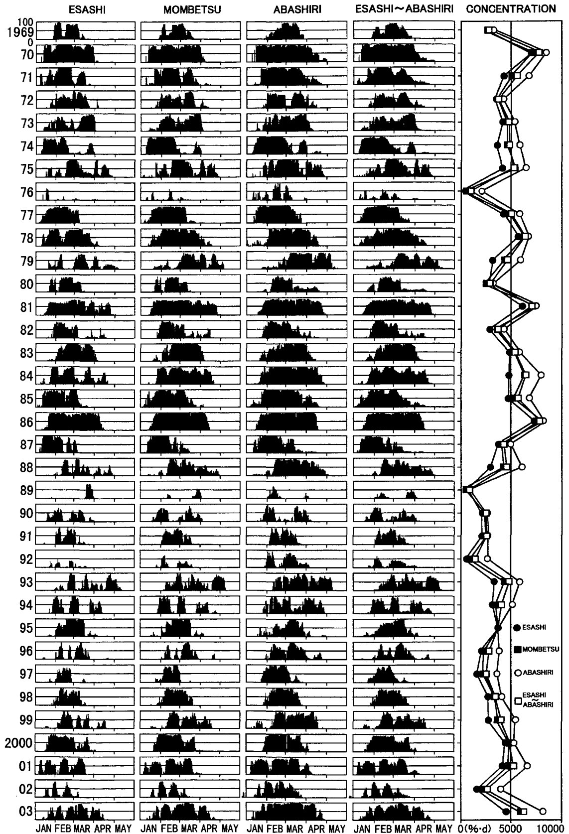
Fig. 2 Daily ice concentrations within about 50-km radar coverage from the coastline during the period from 1969 through 2003.
