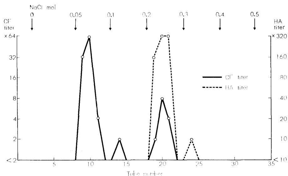
FIGURE 2 Fractionation of ICH soluble antigens on DEAE cellulose column chromatograph—CF titer was measured with anti-virus particle serum D-20
