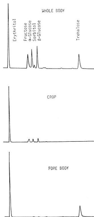
Fig. 1. Gas-liquid chromatograms of sugar contents in the overwintering adults of Ceratina flavipes . Crop and fore body from the same bee
