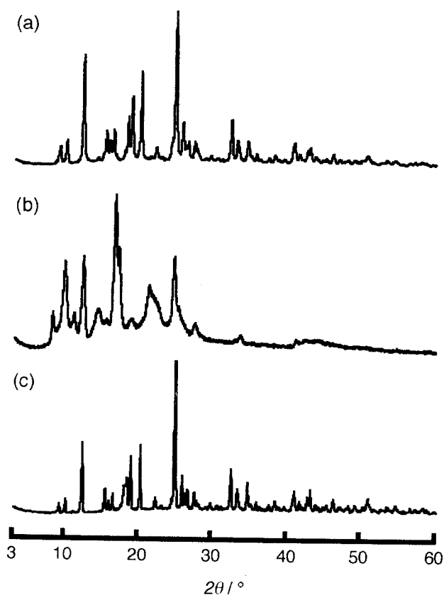
Figure V.14. XRPD patterns of (a) pure V-9·2H 2 O , (b) solid obtained by immersing V-9·2H 2 O in a H 2 O solution containing the 4,4'-bpy ligand and excess amount of NH 4 PF 6 , and (c) solid obtained by immersing V-10 in a H 2 O solution containing excess amount of (NH 4 ) 2 SO 4 .
