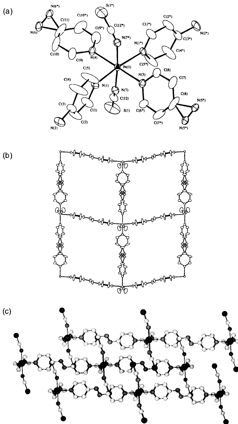
Figure I.4. (a) ORTEP drawing around a Fe(II) center of I-3 at the 30 % probability level. (b) ORTEP view of a 2-D structure of I-3 at the 30 % probability level. (c) View of a stacking form of 2-D sheets of I-3 .
