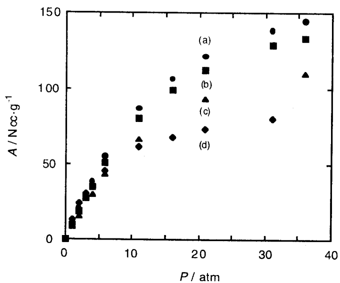
Figure IV.5. Adsorption isotherms of (a) IV-1, (b) IV-2, (c) IV-3, and (d) zeolite 5A, obtained with a CH 4 gas between 1 and 36 atm at 25 °C ( A = \text{absolute adsorption (Ncc}\cdot\text{g}^{-1}) ).
