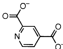
pyridine-2,4-dicarboxylate (2,4-pydc)
