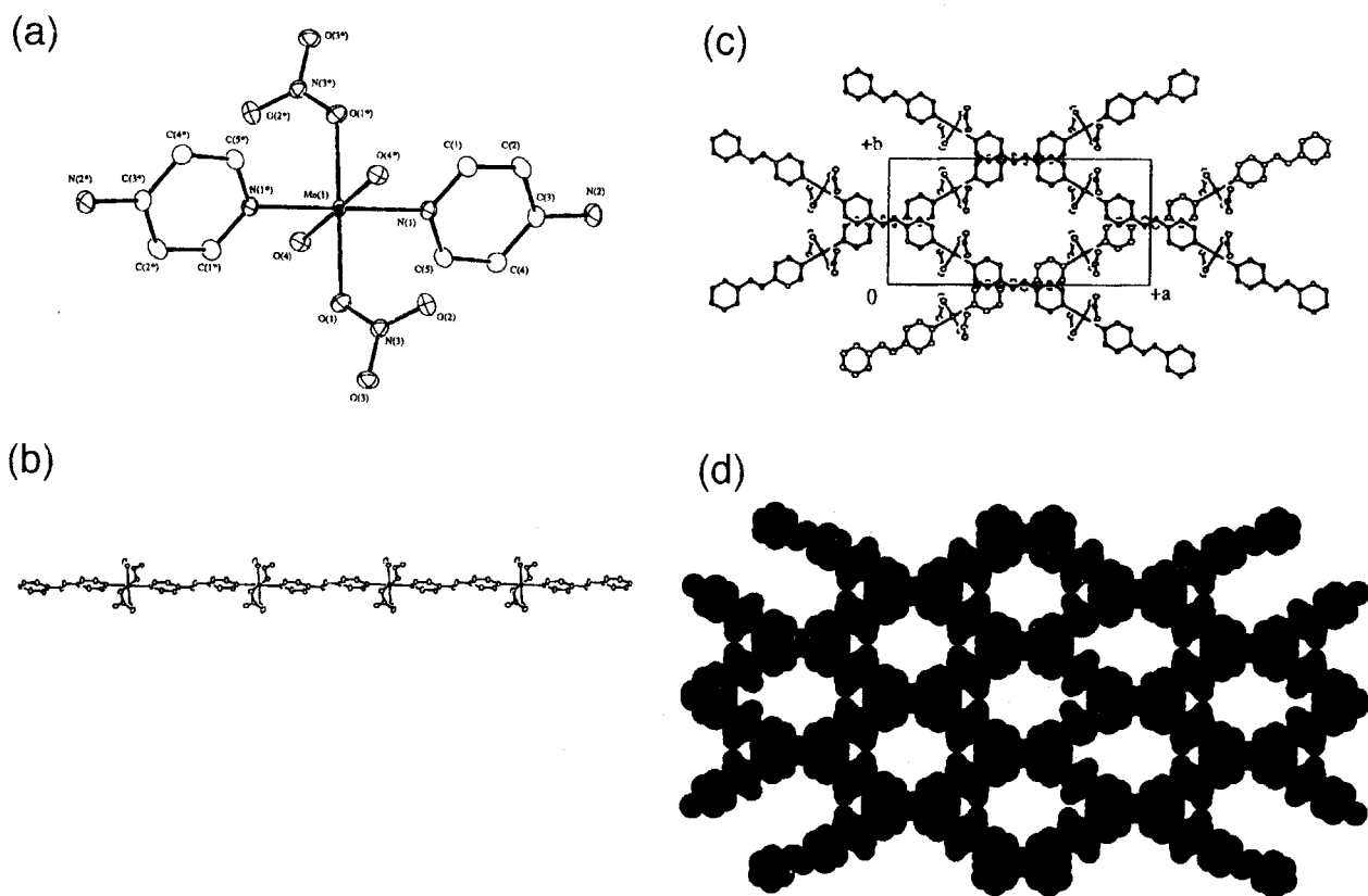
Figure VI.1 (a) ORTEP drawing around the Mn(II) center of VI-1 ·2EtOH at the 30 % probability level. In regard to all figures, the hydrogen atoms are omitted for clarity. (b) ORTEP drawing of a 1-D linear chain structure of VI-1 ·2EtOH. (c) The stacking form of [\text{Mn}(\text{NO}_3)_2(\text{azpy})(\text{H}_2\text{O})_2]_n chains of VI-1 ·2EtOH along the c -axis. (d) A space-filling model of a log-cabin structure of VI-1 ·2EtOH along the c -axis, indicating the aspect of large channel structure. The EtOH molecules are omitted for clarity.
