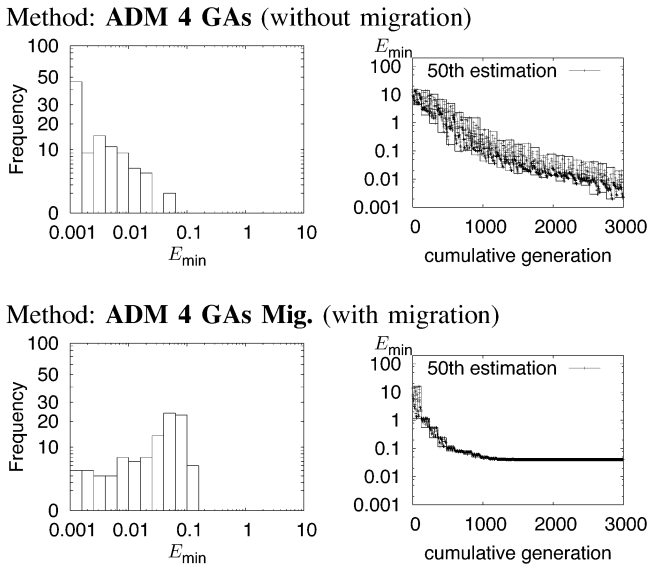
Fig. 6. Difference between cases with and without the migration strategies. Frequency histograms of final least mean square for 100 trials in the left-hand side, and typical examples of convergence profile are shown in the right-hand side. These data are computed by the ADM under “internal type condition” for “Sim-NoError.” Frequencies for which the final least mean square is smaller than the lowest level are counted into the lowest section. The rank of the convergence profiles with respect to the final least mean square is 50th in 100 trials. Each box shows the group of an adaptive range approach that contains four GAs. The label in the abscissa, i.e., “cumulative generation,” means that each generation of a single GA with short lifetime (Max. 30 generations) for the ADM is accumulated.
