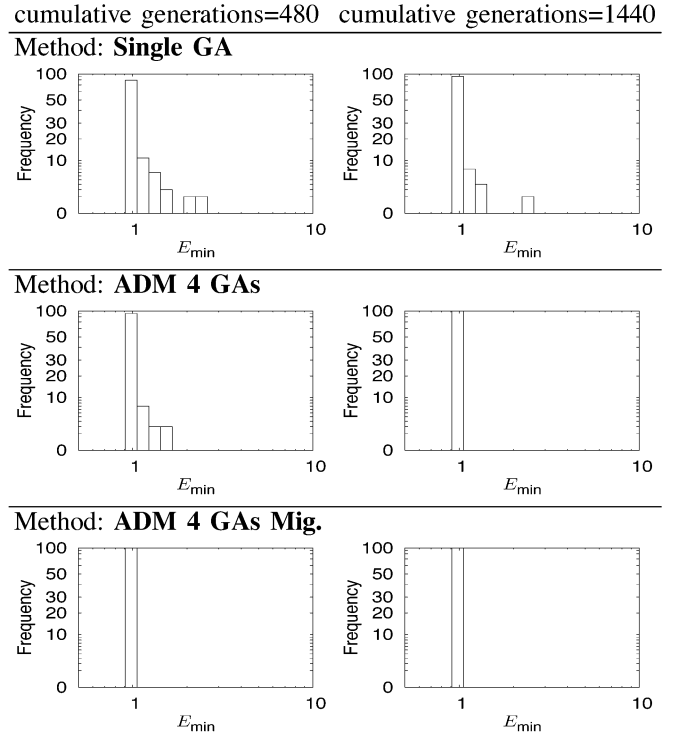
Fig. 7. Frequency histograms for “Sim-with-Error” under “internal type condition,” when the cumulative generations are 480 and 1440.
