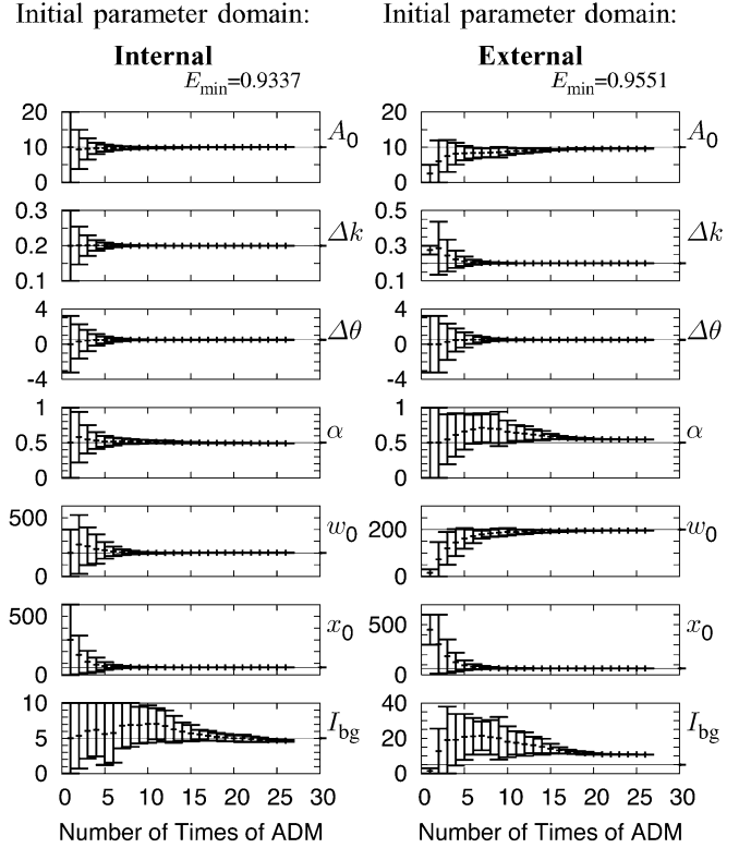
Fig. 9. Convergence of parameter domains for “internal” and “external” data. Input measurement data is “Sim-With-Error,” and ADM is “ADM 4 GAs.” The results are taken from the 50th rank in 100 trials. The bars at each iteration indicate the domain of parameters. Iteration means the number of times to apply the adaptive domain algorithm. The horizontal solid line in each figure shows the parameter assumed initially.
