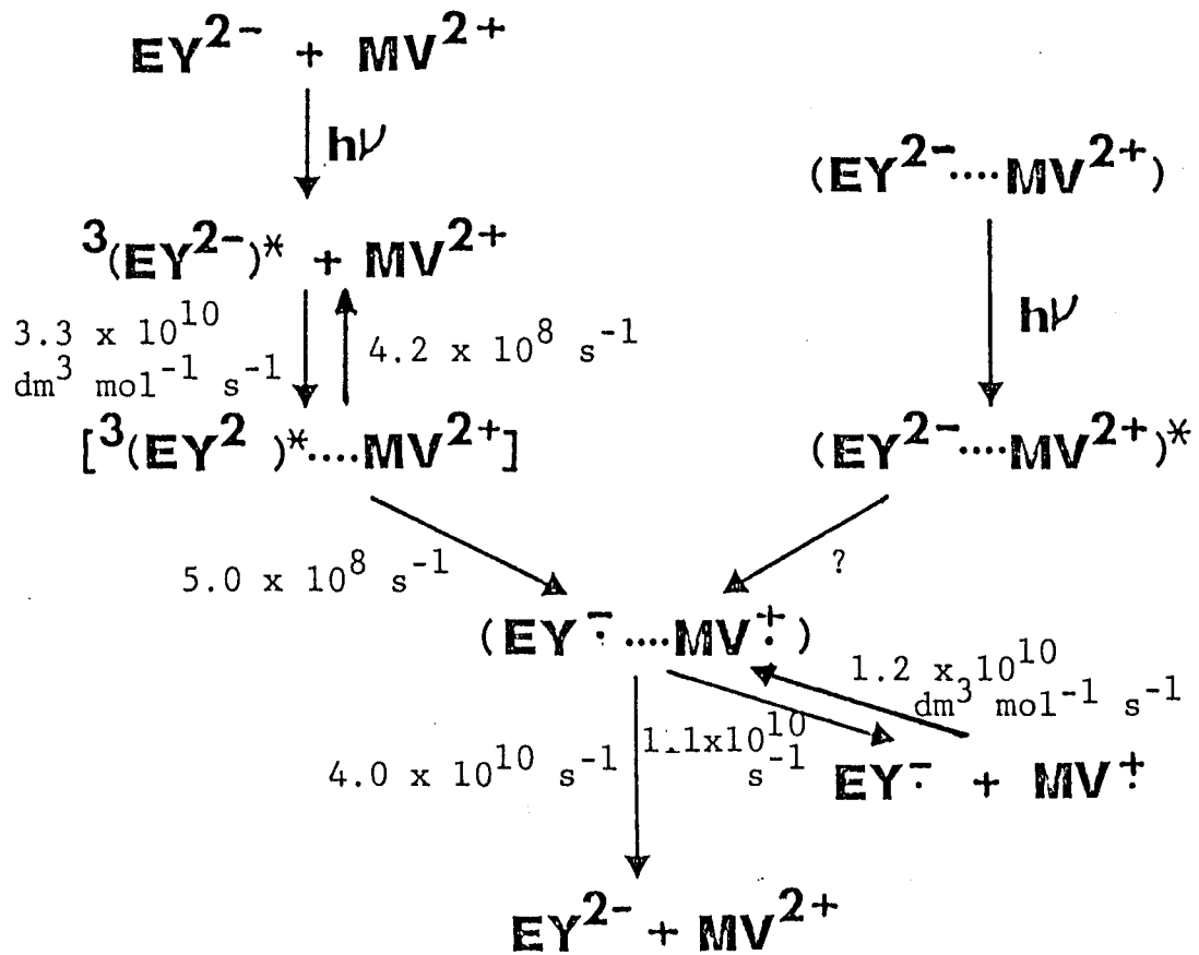
Figure 22. Summary of the rate constants for EY^{2-} - MV^{2+} system.
