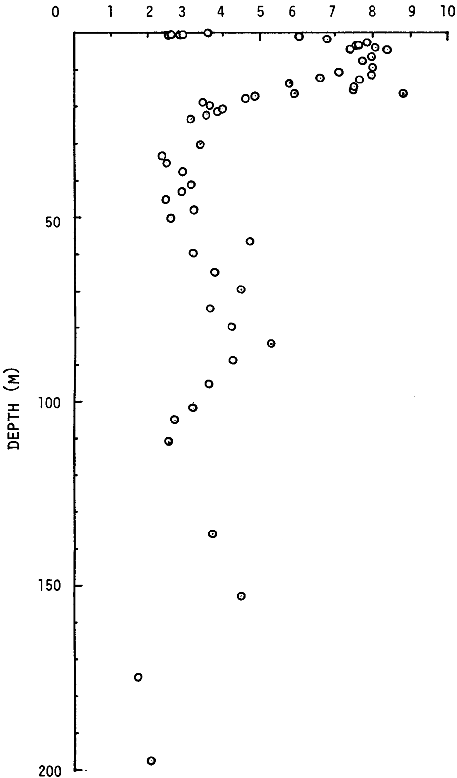
Fig. 6 Vertical profile of humic compounds in a 200 m core of Lake Biwa.
