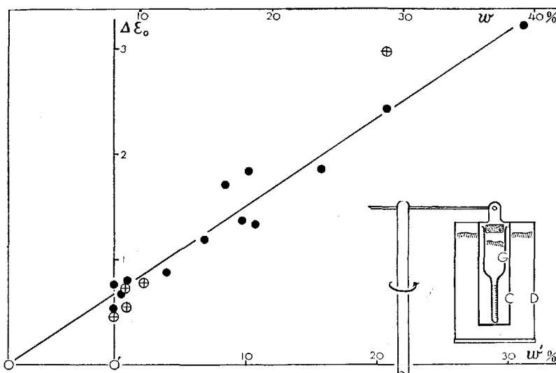
Fig. 17 \Delta\epsilon_0 (the change in the optical dielectric constant accompanying the freezing of wet snow) versus w (the free water content of the wet snow). \Delta\epsilon_0 was determined under the condition that the wet snow had density 0.5 \text{ gr/cm}^3 within the electric condenser. Otherwise the measured \Delta\epsilon_0 was corrected to that density. w' graduated along the bottom line shows the uncorrected value of w as it was observed by use of the hand-driven centrifuge. Cross in circle: soft snow. Solid circle: granular snow.
