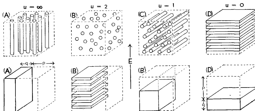
Fig. 12 Hypothetical simplest structures of the ice composing snow on which the Formzahl u can be obtained by theoretical calculation. The figures in the bottom row represent the electrical equivalences to those in the top row.
