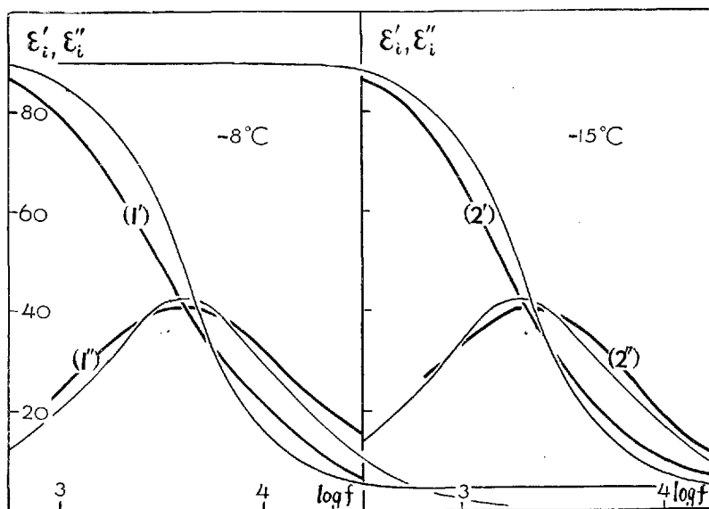
Fig. 3 Comparison of the theoretical and the experimental curves \epsilon'_i - \log f , \epsilon''_i - \log f of ice. The thin lines represent theoretical values drawn after the DEBYE formulae. The thick ones, the experimental, are the same as shown in Fig. 1 by the same marks.
