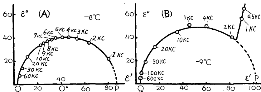
Fig. 2 \epsilon' - \epsilon'' curves of ice. Left: ice of distilled water. Point O is the centre of the half circle. Right: ice made by freezing melted snow.
