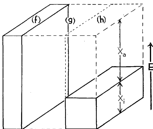
Fig. 14 Model representing the electrical equivalence of snow for any value of the Formzahl u . Parts (f) and (g) in combination represent the longitudinal continuation of ice within the snow while part (h) represents the transverse one.
