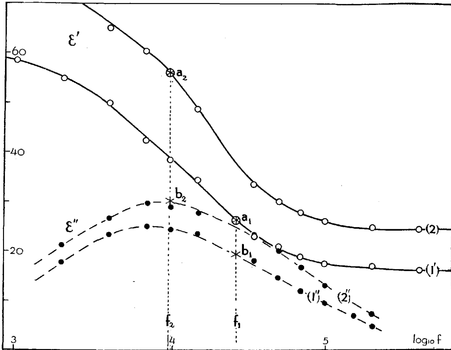
Fig. 16 Curves \epsilon' - \log f , \epsilon'' - \log f of pure snow before and after it is soaked with mineral oil. (1), (1'): before soaking; (2), (2'): after soaking.
