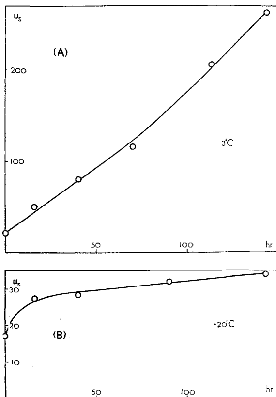
Fig. 13 The Formzahl u_s for the static dielectric constant of snow increases with time due to the sublimation metamorphosis.
