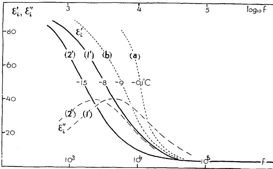
Fig. 1 Dielectric constant \epsilon'_i and dielectric loss factor \epsilon''_i of ice versus \log f . f : frequency (cycle/sec) of the applied alternating electric force.
