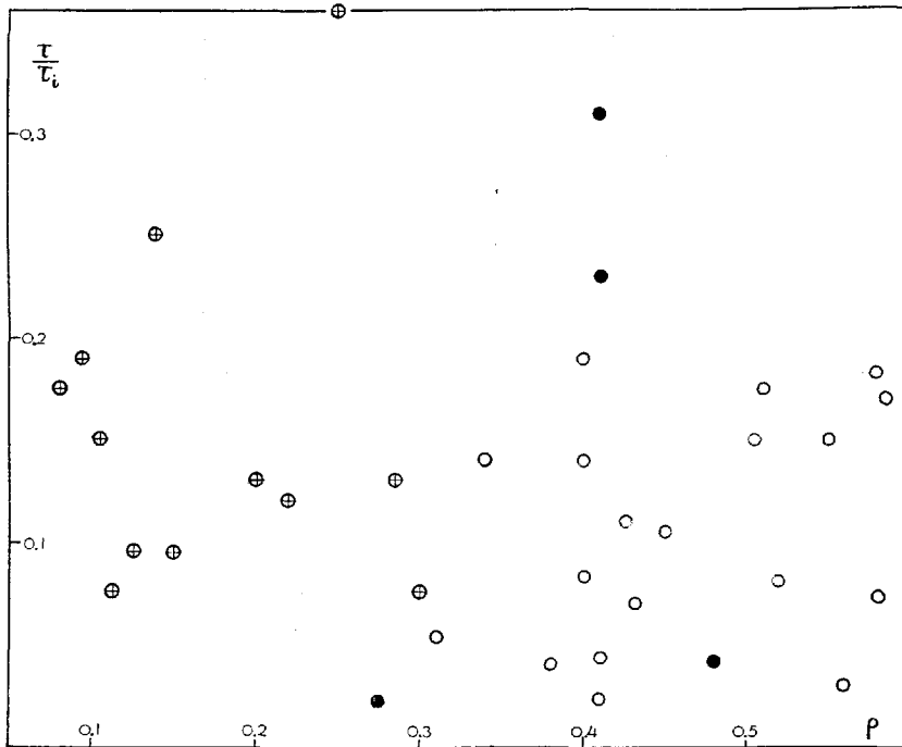
Fig. 11 The ratio of \tau to \tau_i versus the density \rho of snow. \tau and \tau_i are respectively the relaxation times of snow and ice at the same temperature. Cross in circle: soft snow; light circle: compact snow; solid circle: granular snow.
