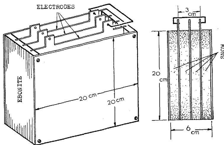
Fig. 4 Condenser used for determining \epsilon' and \epsilon'' of snow.
