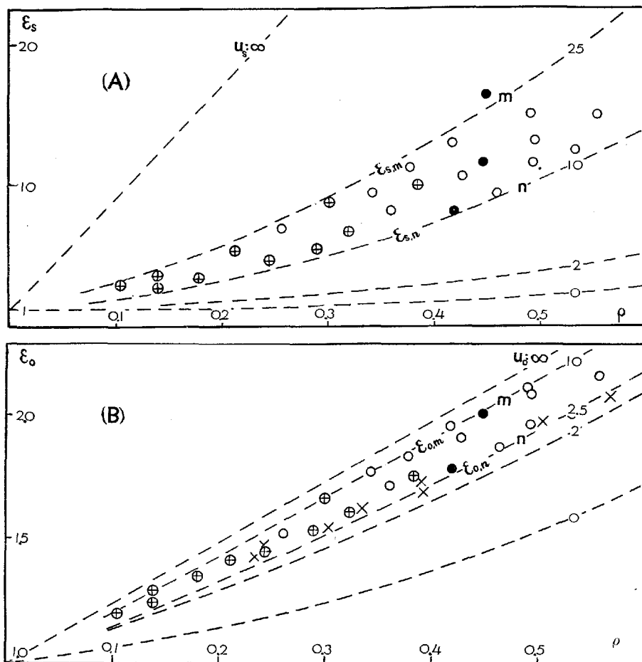
Fig. 10 Static dielectric constant \epsilon_s and optical dielectric constant \epsilon_0 of snow versus its density \rho . The broken curves represent WIENER's formula. Numerical figures attached to the curves indicate the value of Formzahl u . The observed points are distinguished according to the sort of snow: cross in circle—soft snow; light circle—compact snow; solid circle—granular snow. Mark of soft snow corresponding to \rho > 0.2 shows an artificially compacted soft snow. Crosses in the lower figure are after CUMMING.
