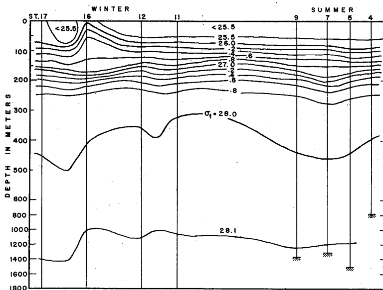
Fig. 13. Distribution of density ( \sigma_t ) in a vertical section between St. 4 and St. 17 at T-3.
