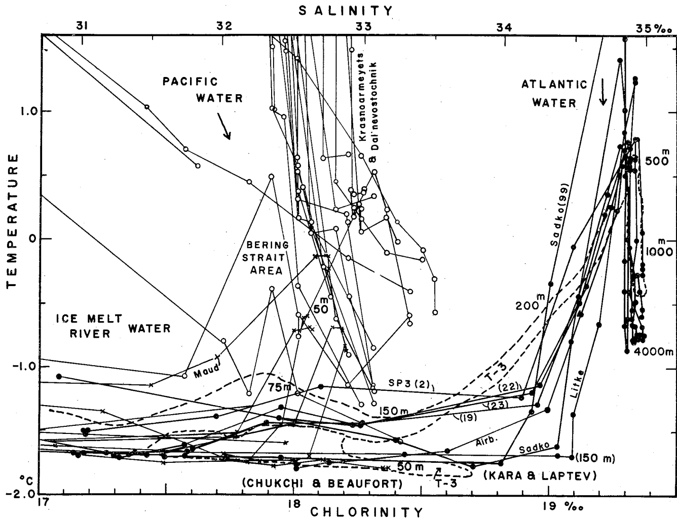
Fig. 26 b. Temperature-chlorinity diagram for the stations in the Arctic Ocean. Crosses: Maud , Open circles: Krasnoarmeyets and Dal'nevostochnik , Closed circles: Russian stations shown in Table 10 and Fig. 26 a.
