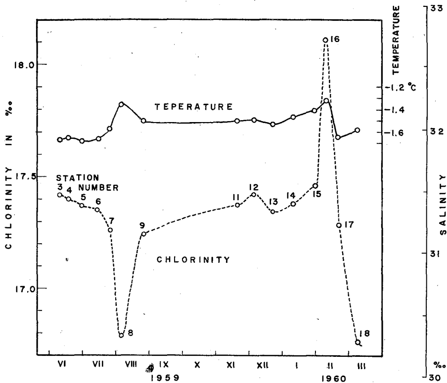
Fig. 28. Seasonal variation of chlorinity and temperature at 30 meters (Ice Island T-3).
