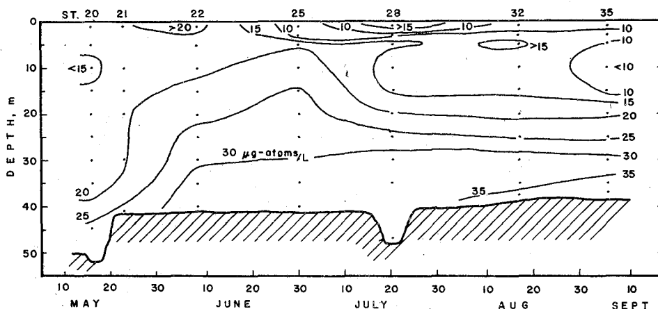
Fig. 21. Vertical distribution of silicate-silicon ( \mu\text{g-atoms/l} ) in a vertical section between St. 20 and St. 35 at T-3.
