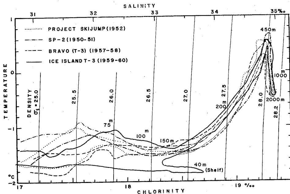
Fig. 25. Temperature-chlorinity diagram for the stations from T-3, SP-2, and Project Skijump.
