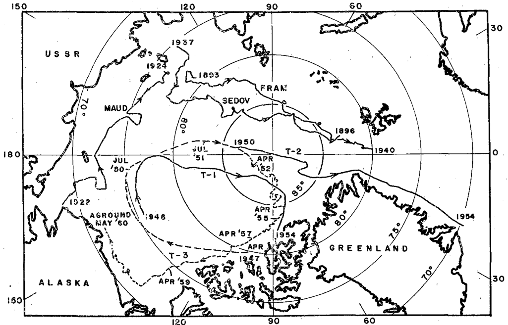
Fig. 2. Drift paths of ships and ice islands.
