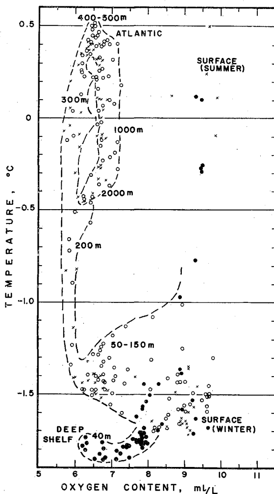
Fig. 18. Temperature-oxygen relationship for stations at T-3. Crosses: Sts. 4-10 (Summer). Open circles: Sts. 11-18 (winter). Closed circles: Sts. 20-35 (on the shelf).
