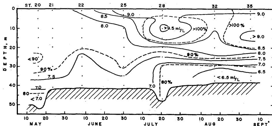
Fig. 16. Distribution of oxygen content (m/l) and percentage saturation in a vertical section between St. 20 and St. 35 at T-3.
