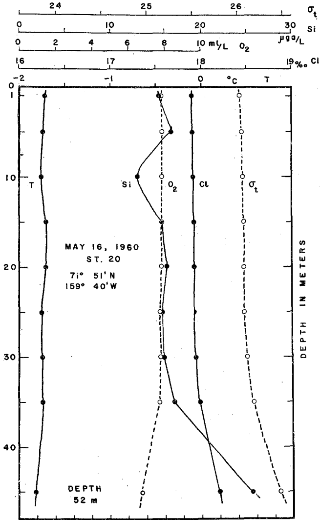
Fig. 6 d. Vertical distribution of temperature, density, and chemical elements at Station 20, May 16, 1960.
