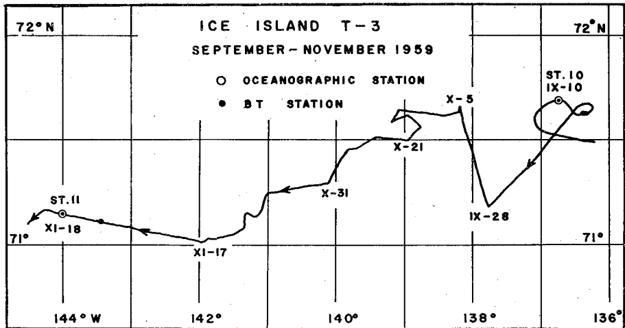
Fig. 4 b. Path of Ice Island T-3 and positions of stations, September-November 1959.
