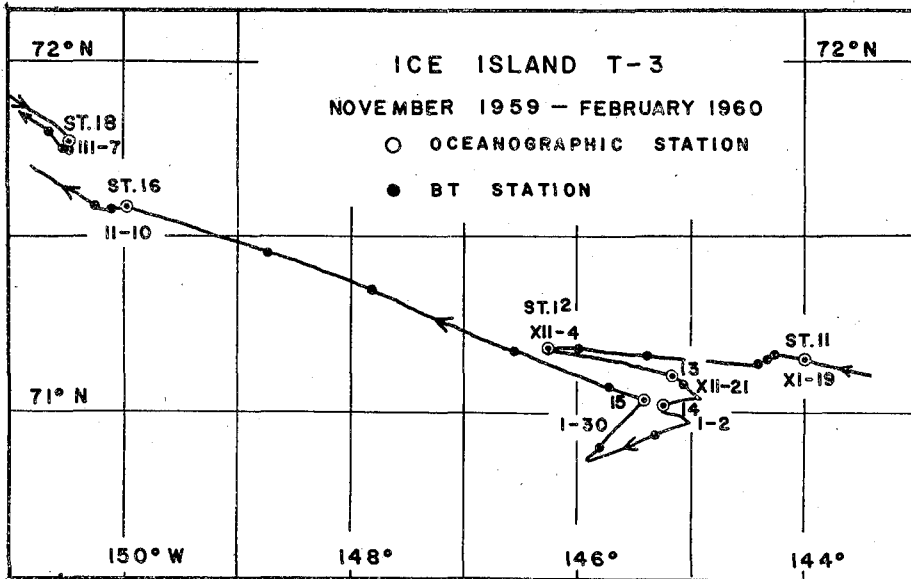
Fig. 4c. Path of Ice Island T-3 and positions of stations, November 1959-February 1960.
