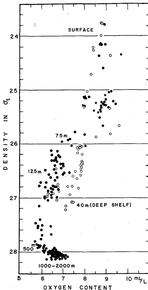
Fig. 17. Density ( \sigma_t )-oxygen relationship from data obtained at T-3.
