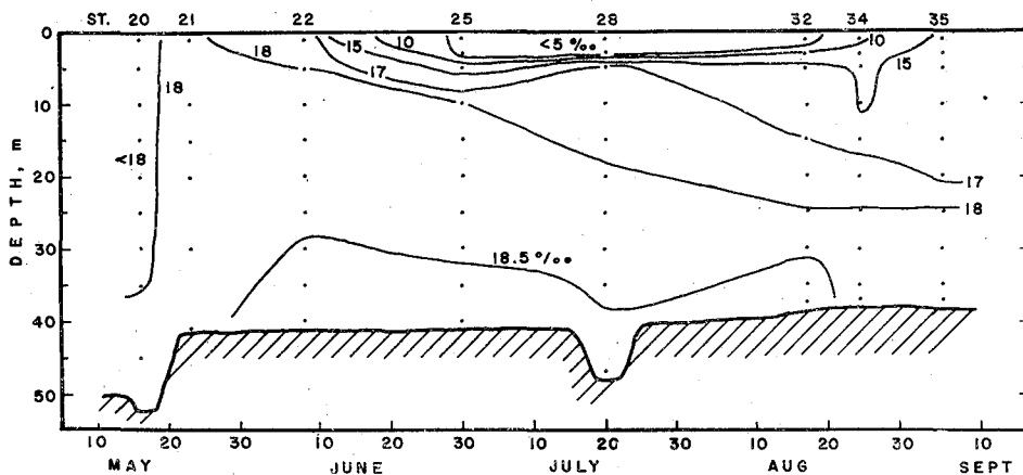
Fig. 11. Distribution of chlorinity in a vertical section between St. 20 and St. 35 at T-3.
