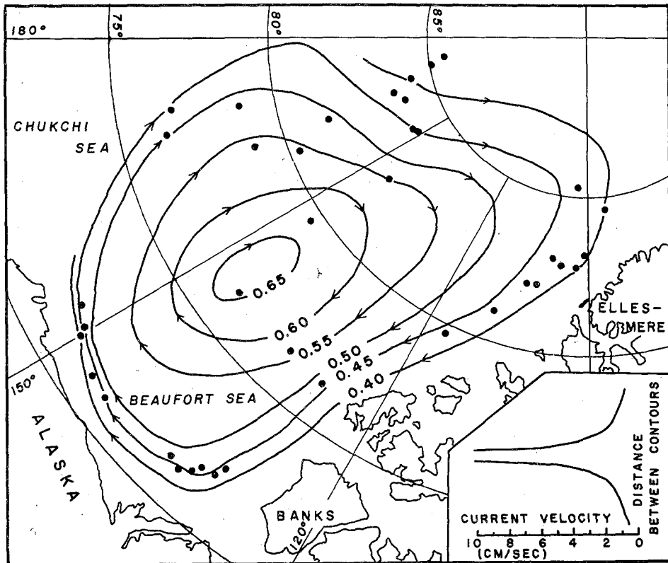
Fig. 31. Topography of the sea surface (dyn m) relative to the 600-decibar surface.
