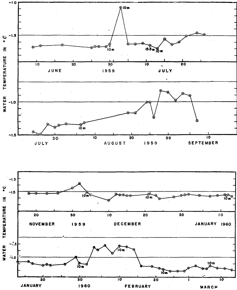
Fig. 7 a. Annual variation of temperature (at 15 meters except where noted otherwise). June 1959-September 1960.
