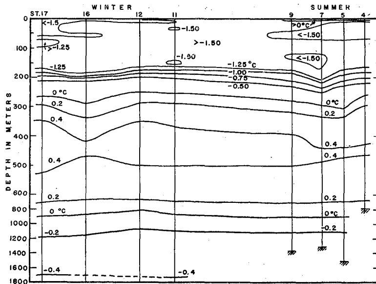
Fig. 8. Distribution of temperature in a vertical section between St. 4 and St. 17 at T-3.
