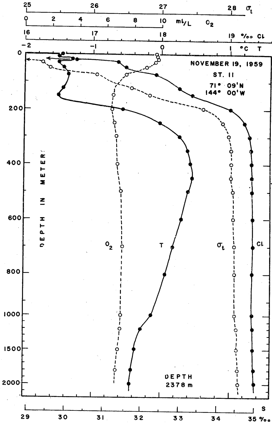
Fig. 6b. Vertical distribution of temperature, density, and chemical elements at Station 11, November 19, 1959.
