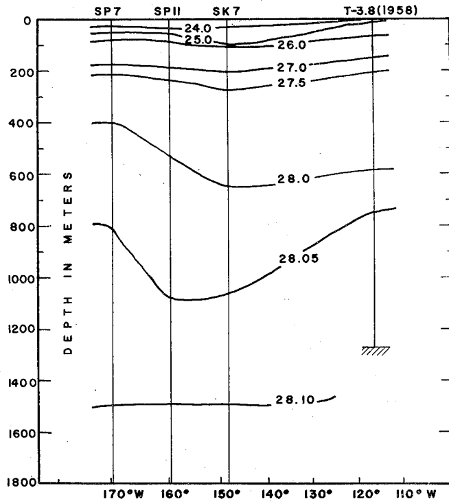
Fig. 30b. Density distribution in a vertical section along latitude 80°N. (Locations of the stations are shown in Fig. 2).
