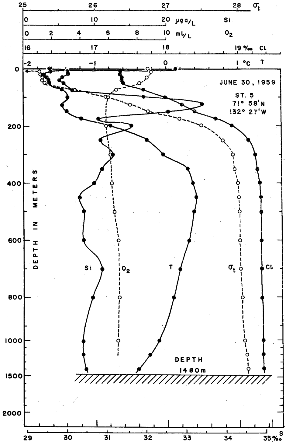
Fig. 6 a. Vertical distribution of temperature, density, and chemical elements at Station 5, June 30, 1959.
