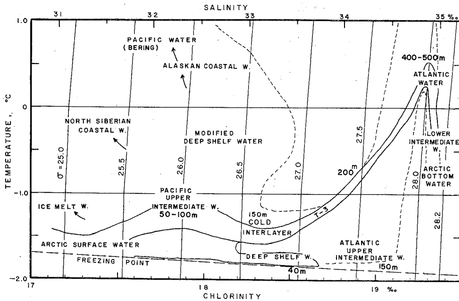
Fig. 29. Temperature-chlorinity relations of the water masses in the Arctic Ocean.
