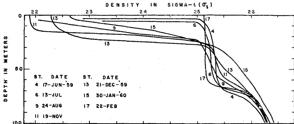
Fig. 27. Annual variation in density ( \sigma_t ) in the upper layer (0–100 m) observed at the Ice Island T-3.
