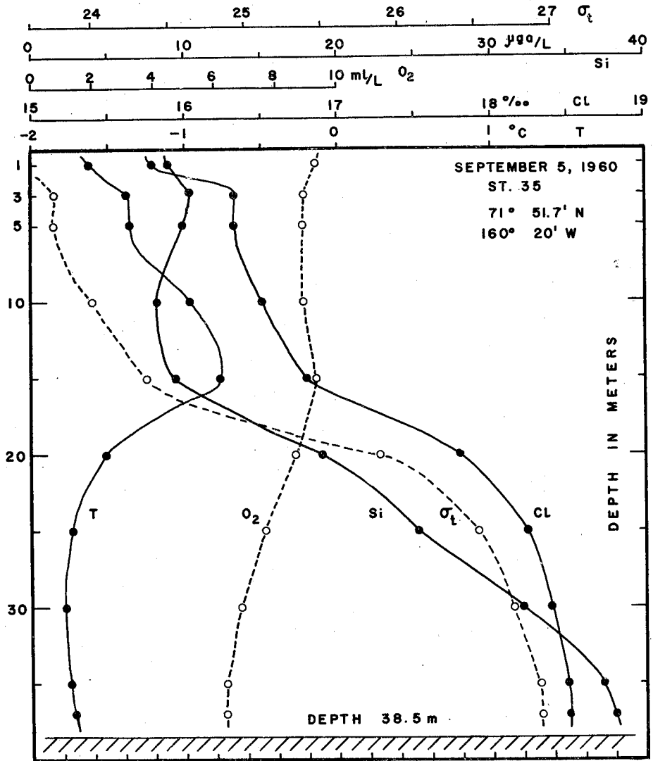
Fig. 6e. Vertical distribution of temperature, density, and chemical elements at Station 35, September 5, 1960.
