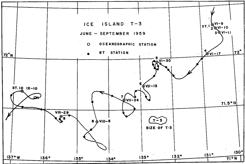
Fig. 4 a. Path of Ice Island T-3 and positions of stations, June-September 1959.
