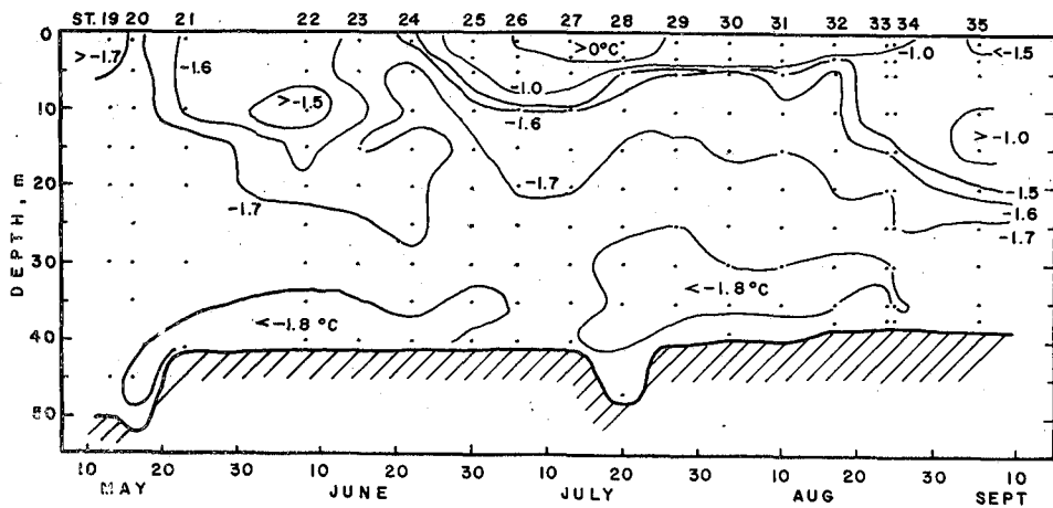
Fig. 9. Distribution of temperature in a vertical section between St. 19 and St. 35 at T-3.
