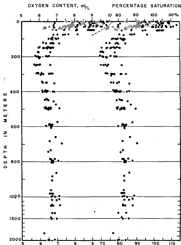
Fig. 14. Vertical distribution of dissolved oxygen content (ml/l) and percentage saturation (%) observed at T-3. Open circles indicate the values at Sts. 20-35.
