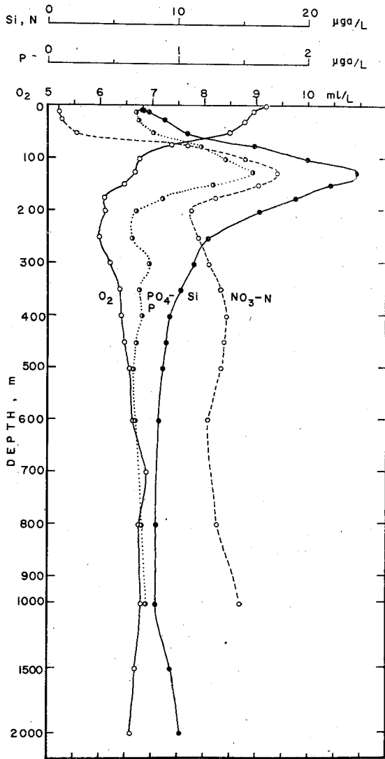
Fig. 22. Vertical distribution of average content of dissolved oxygen, nitrate-N, phosphate-P, and silicate-Si observed at Ice Island T-3.
