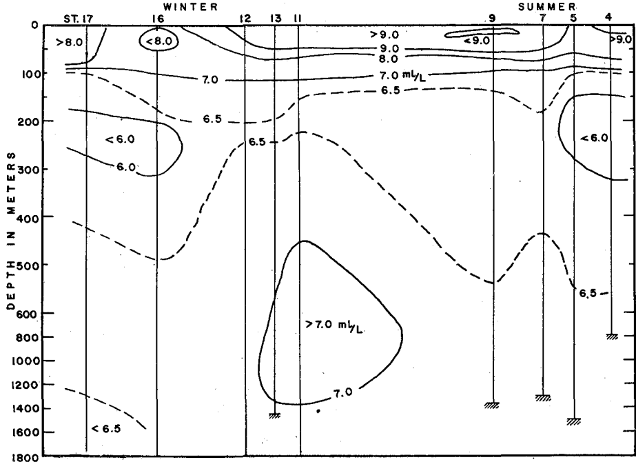
Fig. 15. Distribution of oxygen content (m/l) in a vertical section between St. 4 and St. 17 at T-3.
