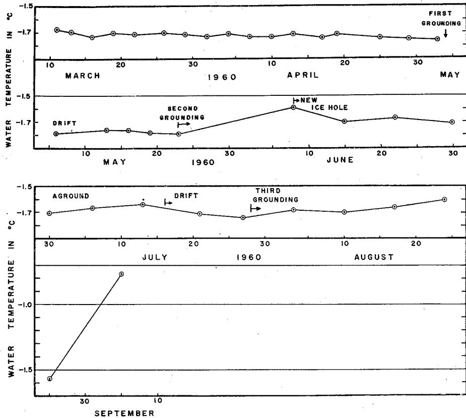
Fig. 7b. Annual variation of temperature (at 15 meters except where noted otherwise). June 1959--September 1960.
