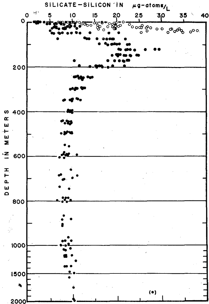
Fig. 19. Vertical distribution of silicate-silicon ( \mu\text{g-atoms/l} ) observed at T-3 in 1959-1960. Open circles indicate the values at Sts. 20-35.
