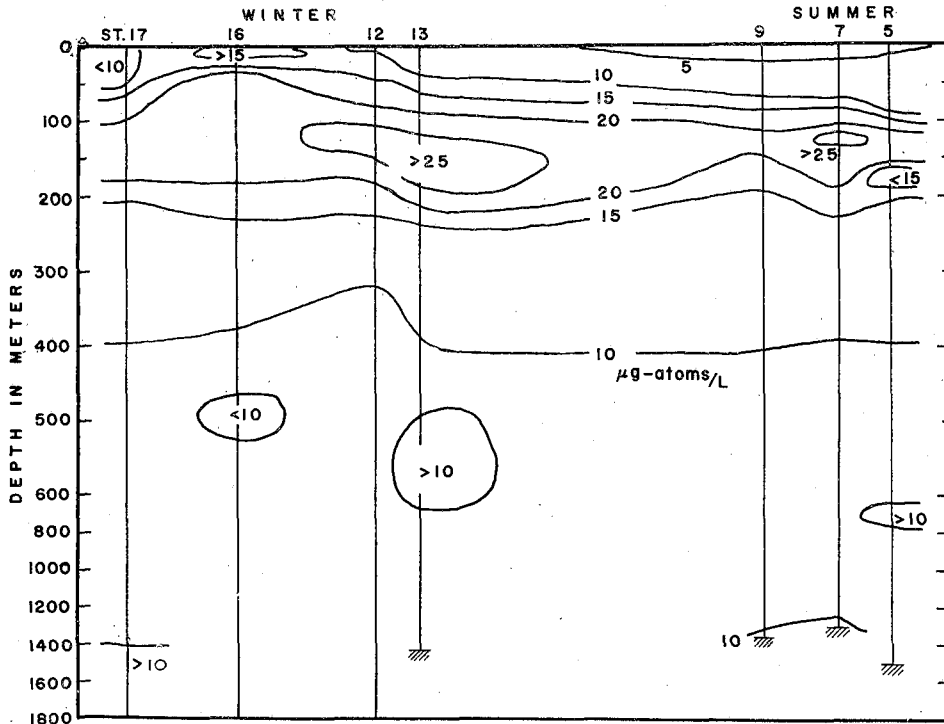
Fig. 20. Distribution of silicate-silicon ( \mu\text{g-atoms/l} ) in a vertical section between St. 5 and St. 17 at T-3.
