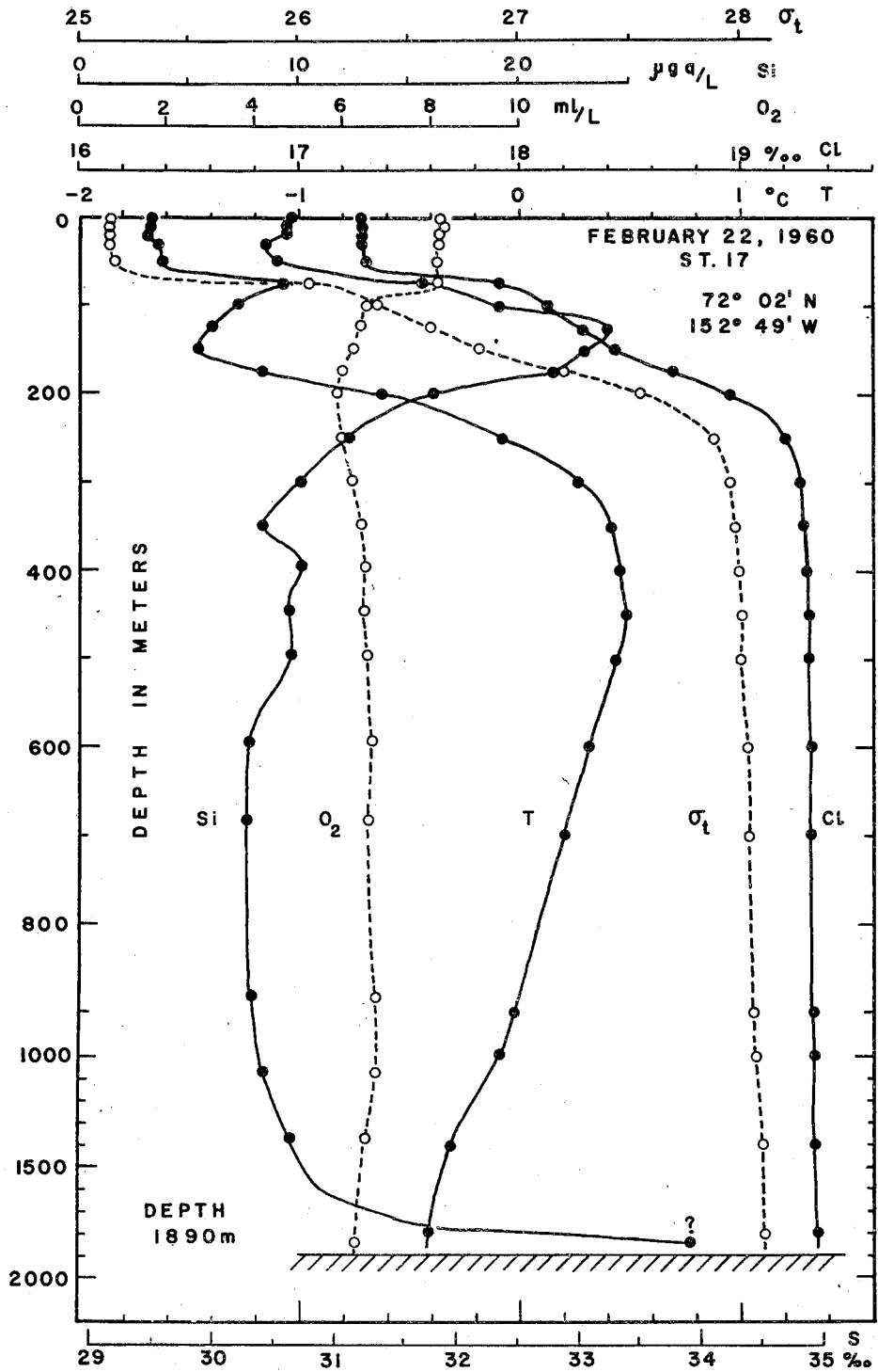
Fig. 6c. Vertical distribution of temperature, density, and chemical elements at Station 17, February 22, 1960.
