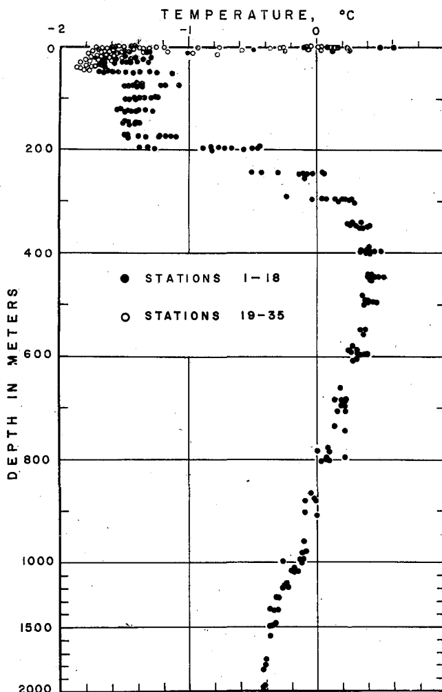
Fig. 5. Vertical distribution of temperatures observed at T-3 in 1959-1960.
