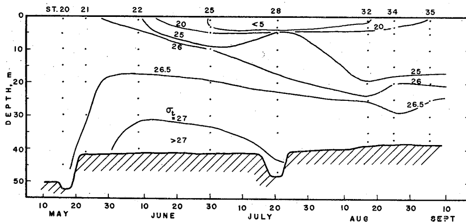
Fig. 12. Distribution of density ( \sigma_t ) in a vertical section between St. 20 and St. 35 at T-3.
