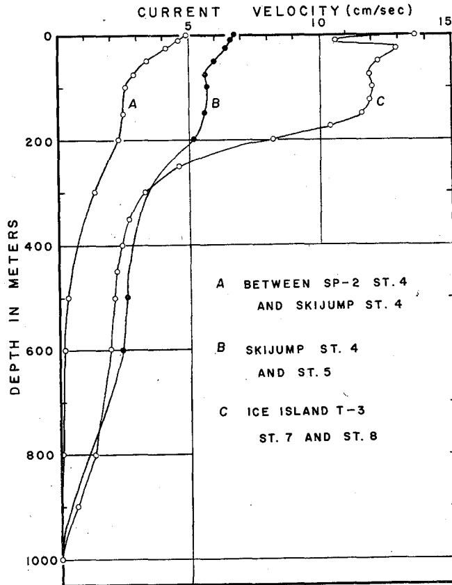
Fig. 32. Examples of the vertical distribution of current magnitude according to the dynamic computation.
