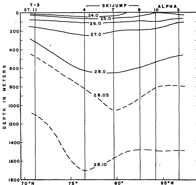
Fig. 30a. Density distribution in a vertical section along the 145°W meridian in the Pacific side of the Arctic Ocean. (Locations of stations are shown in Fig. 2).
