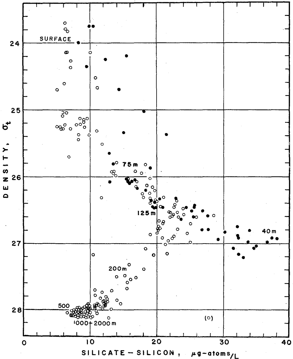
Fig. 23. Density ( \sigma_t )-silicon relationship for T-3 stations.
