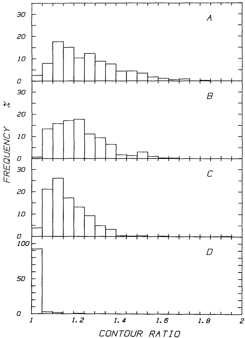
Fig. 27 Histograms of snow particle contour ratio r .
