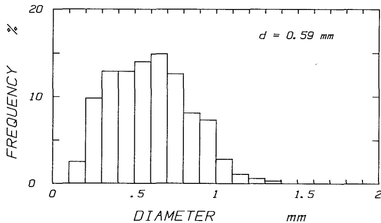
Fig. 7 Histogram of snow particle diameters.
