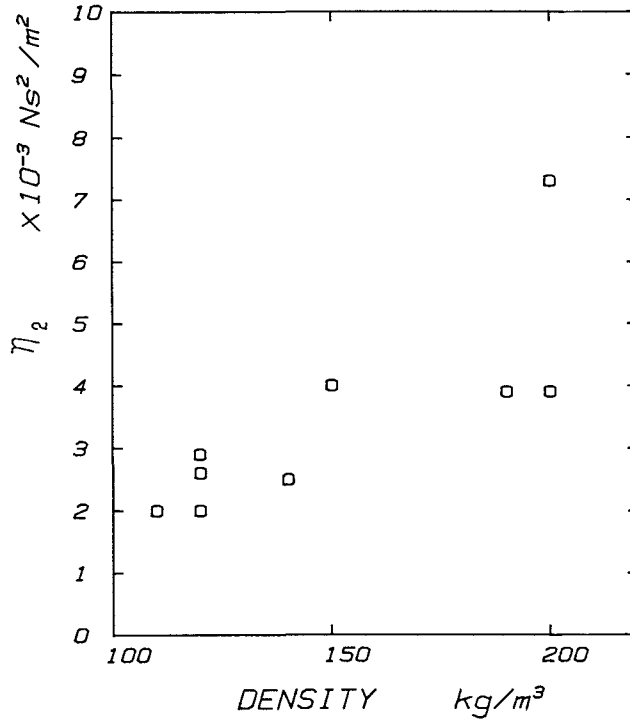
Fig. 38 \eta_2 of fluidized snow versus bulk density.
