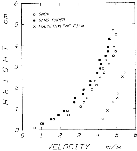
Fig. 10 Velocity profiles of the snow flow on various floor conditions.
