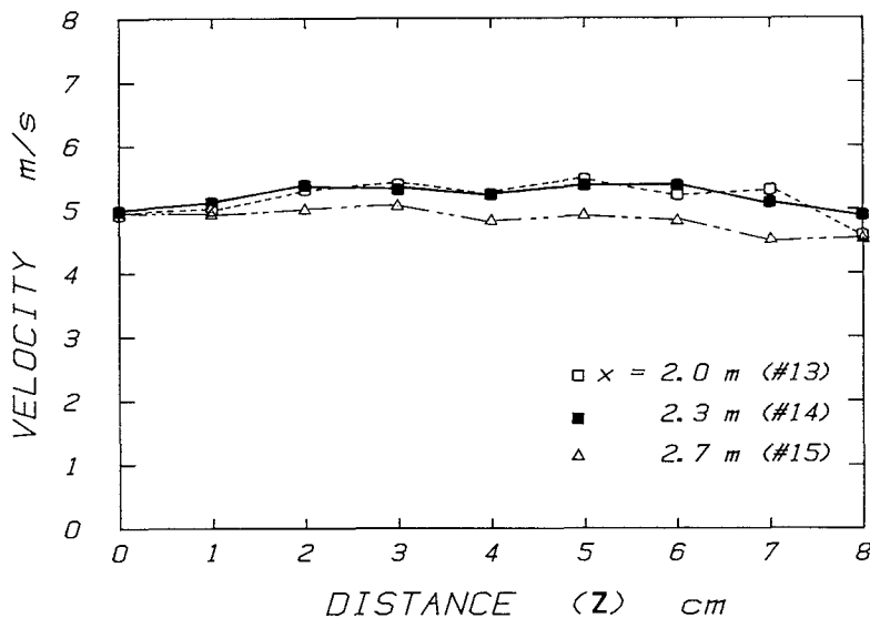
Fig. 9 Velocity profiles across a snow flow. Measured at x=2.0 , 2.3 and 2.7 m. Walls are glass ( z=0 ) or wood ( z=8 ).
