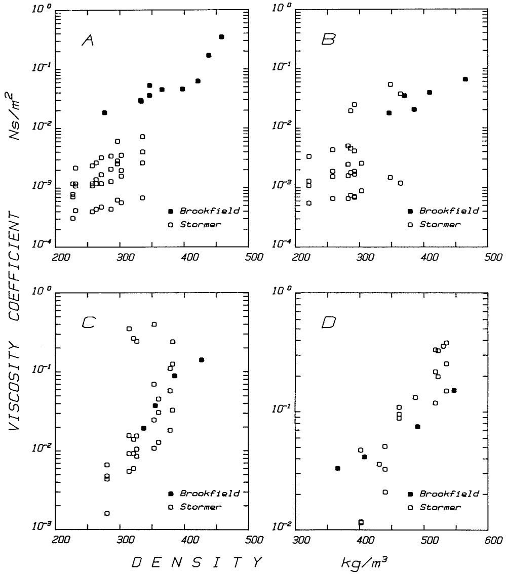
Fig. 33 Viscosity coefficients of the fluidized-bed of snow measured with the Brookfield viscometer and the modified Stormer-type viscometer.
