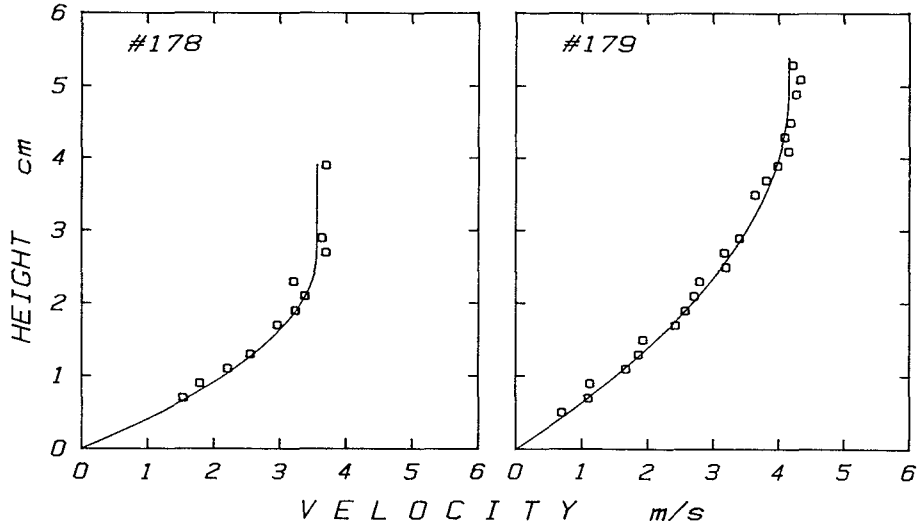
Fig. 19 Measured and calculated velocity profiles of snow flow (2). \tau_0 is 10.5 N/m 2 and 3.5 N/m 2 for #178 and #179 respectively.
