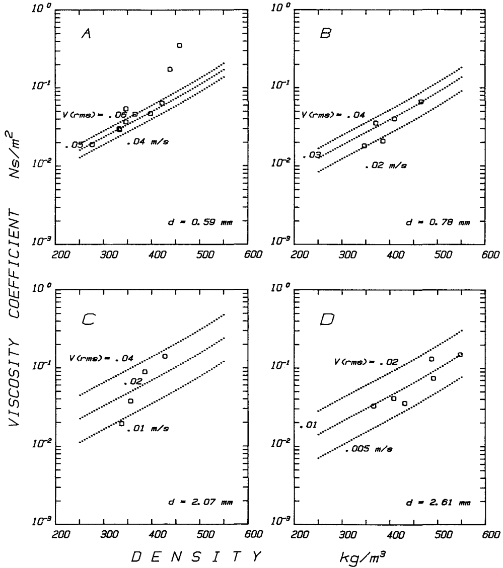
Fig. 41 Comparisons of the fluidized-bed experimental results with the calculated results. The dotted lines represent the theory of Savage & Jeffrey (1981).
