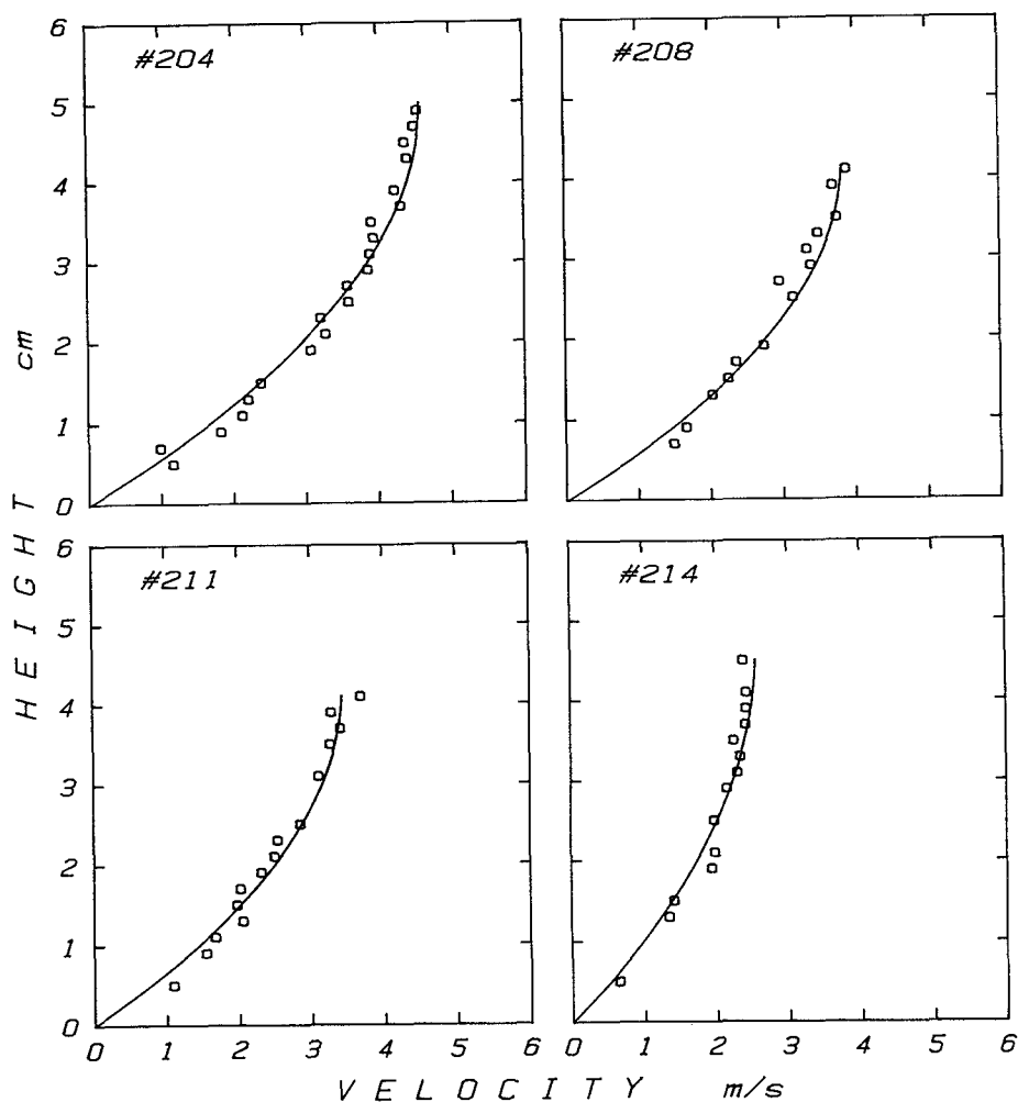
Fig. 20 Measured and calculated velocity profiles of snow flow (3). \tau_0 is 0 N/m 2 for all cases.
