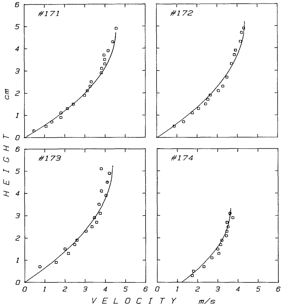
Fig. 18 Measured and calculated velocity profiles of snow flow (1). \tau_0 is 0 N/m 2 for all cases.
