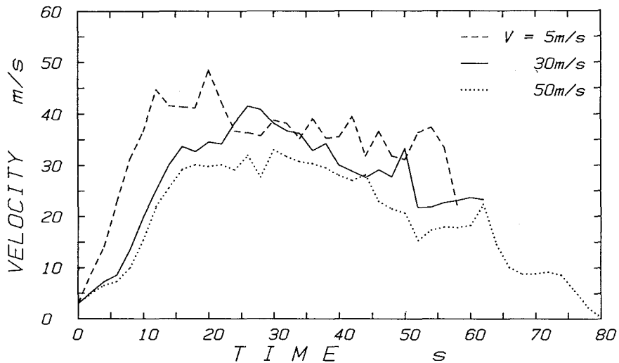
Fig. 45 Numerical simulations of the natural snow avalanche motions in the Shiai-dani region on February 3, 1988. Values of parameters selected are the same as in Fig. 44 but V in Eq. (23).
