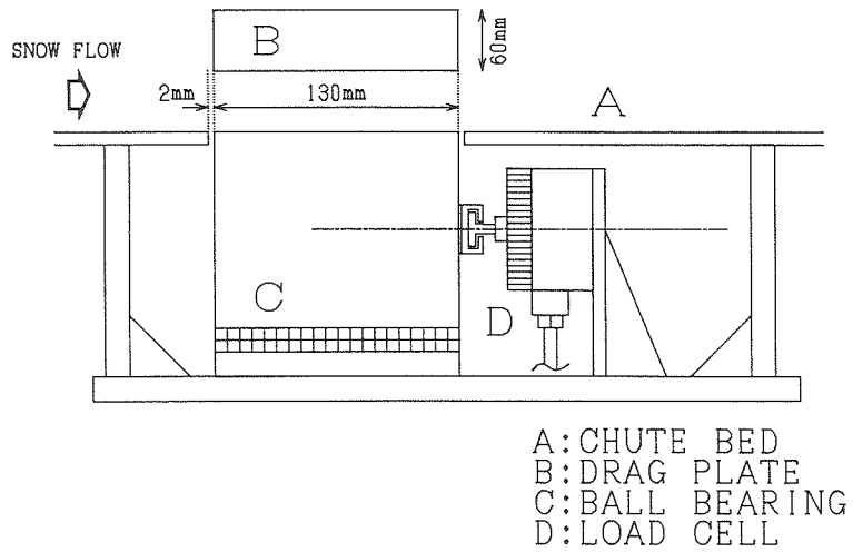
Fig. 4 Fundamentals of the drag meter's structure.
