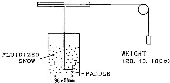
Fig. 24 Modified Stormer-type viscometer.
