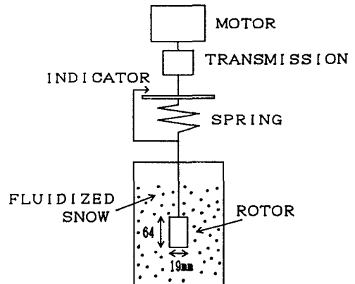
Fig. 23 Brookfield viscometer.
