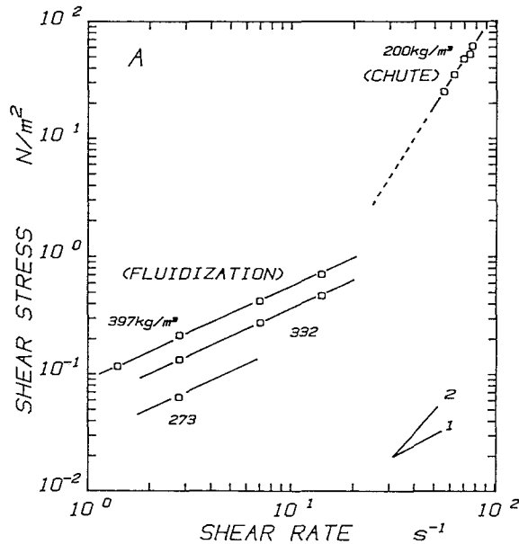
Fig. 39 Relation between the shear stress and the shear rate for the fluidized snow obtained with the inclined chute and the fluidized-bed experiments.
