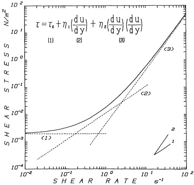
Fig. 42 Relation between the shear stress and the shear rate for the fluidized snow of 200 \text{ kg/m}^3 . Dotted lines show the individual contributions of Eq. (23) and solid line shows the total shear stress.
