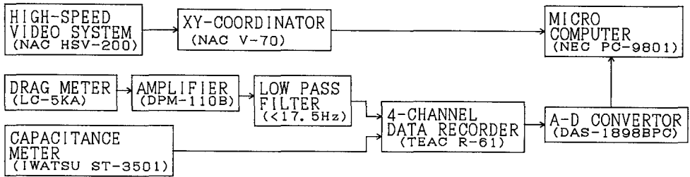
Fig. 6 Block diagram of the measuring and analyzing system.
