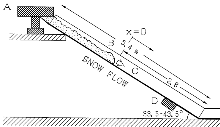
Fig. 1 Schematic diagram showing the experimental set-up.
