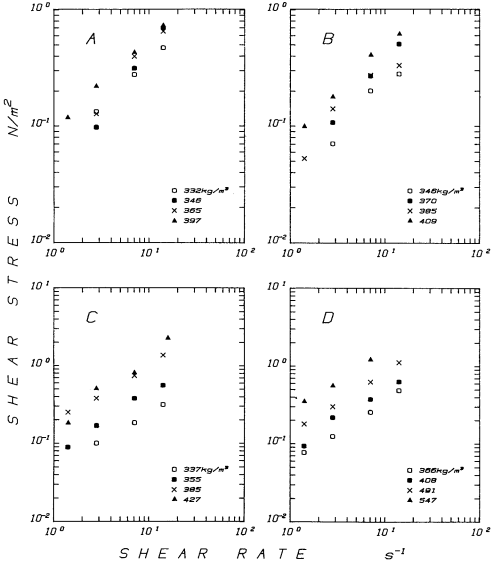
Fig. 28 Shear stress versus shear rate in the fluidized-bed of snow with the Brookfield viscometer. A: d = 0.59 mm, B: d = 0.78 mm, C: d = 2.07 mm and D: d = 2.61 mm.
