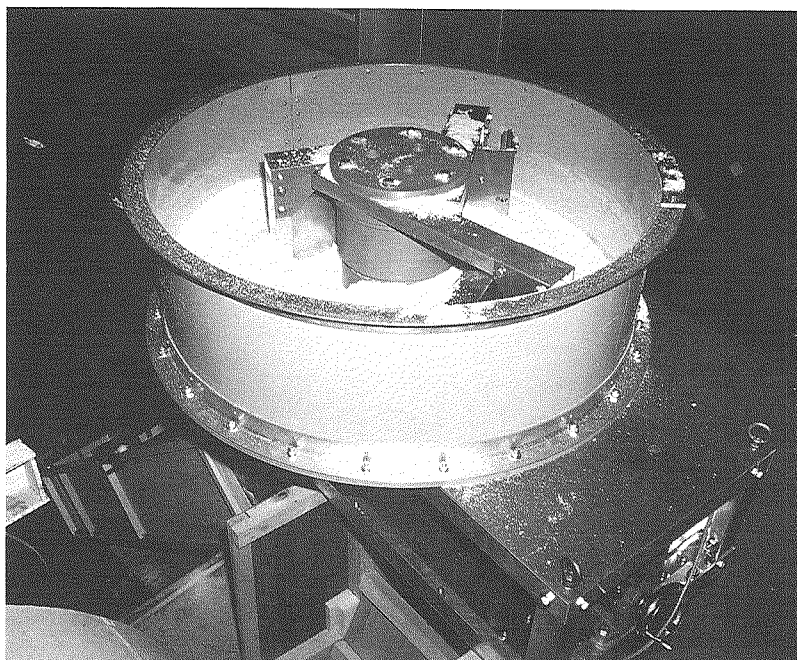
Fig. 2 Photograph of the fluidized snow feeder.
