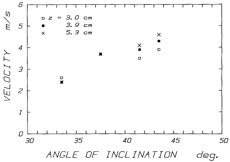
Fig. 15 Snow flow velocities versus chute angles.
