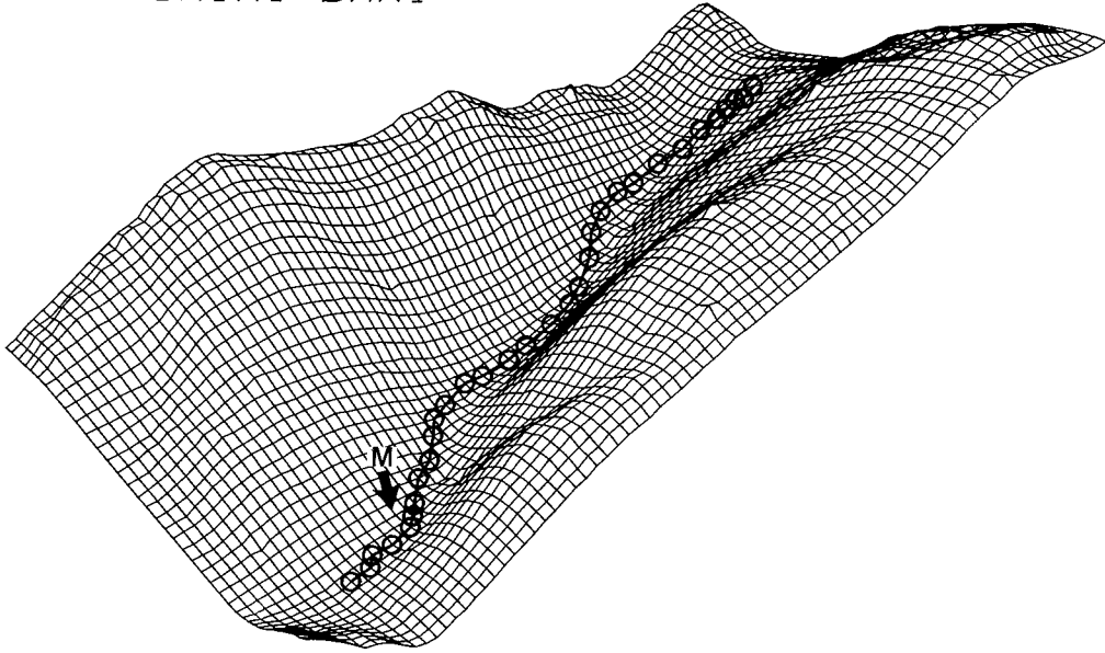
Fig. 46 Change in calculated velocities of snow avalanche along the avalanche shoot. M represents the observation site.
