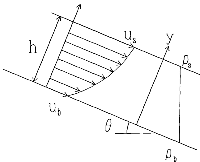
Fig. 35 Two dimensional snow flow down an inclined chute (II). \rho_s and \rho_b are bulk densities at surface and bed; u_b is a slip velocity.
