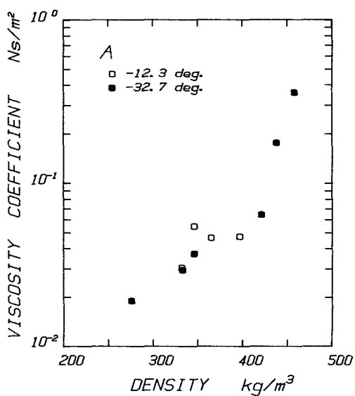
Fig. 29 Viscosity coefficients versus bulk densities for sample A ( d=0.59 mm).
