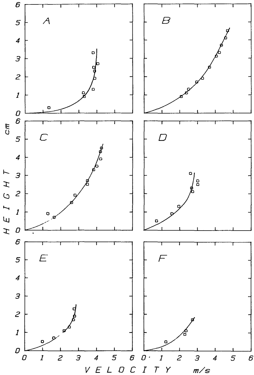
Fig. 12 Velocity profiles of the snow flow at A, B, C and D in Fig. 11.
