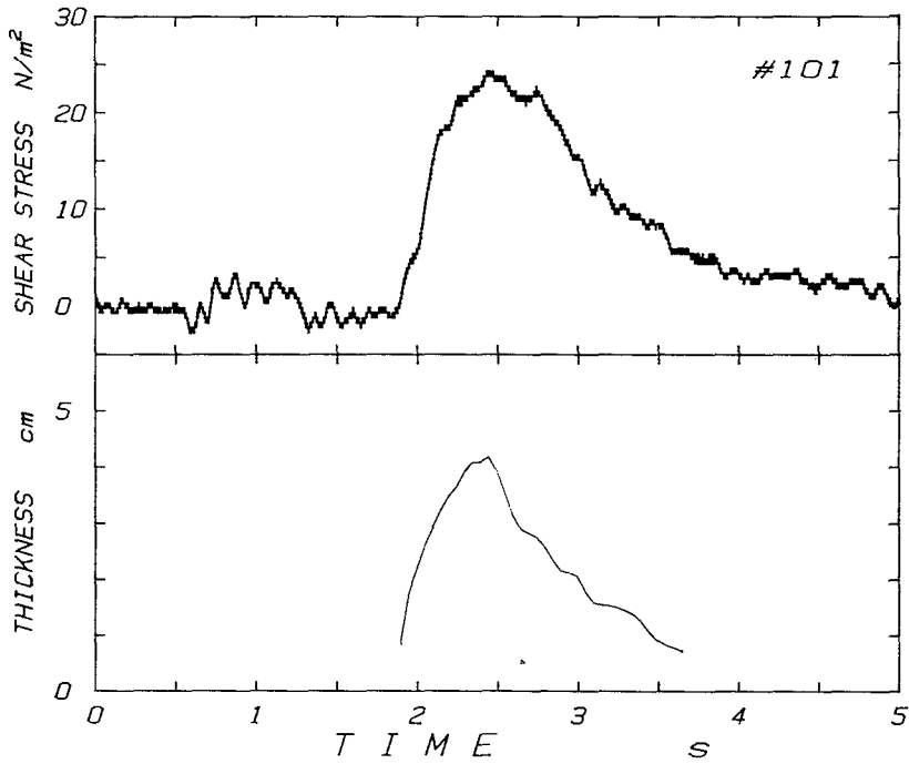
Fig. 16 Time variation of basal shear stress and snow flow thickness.
