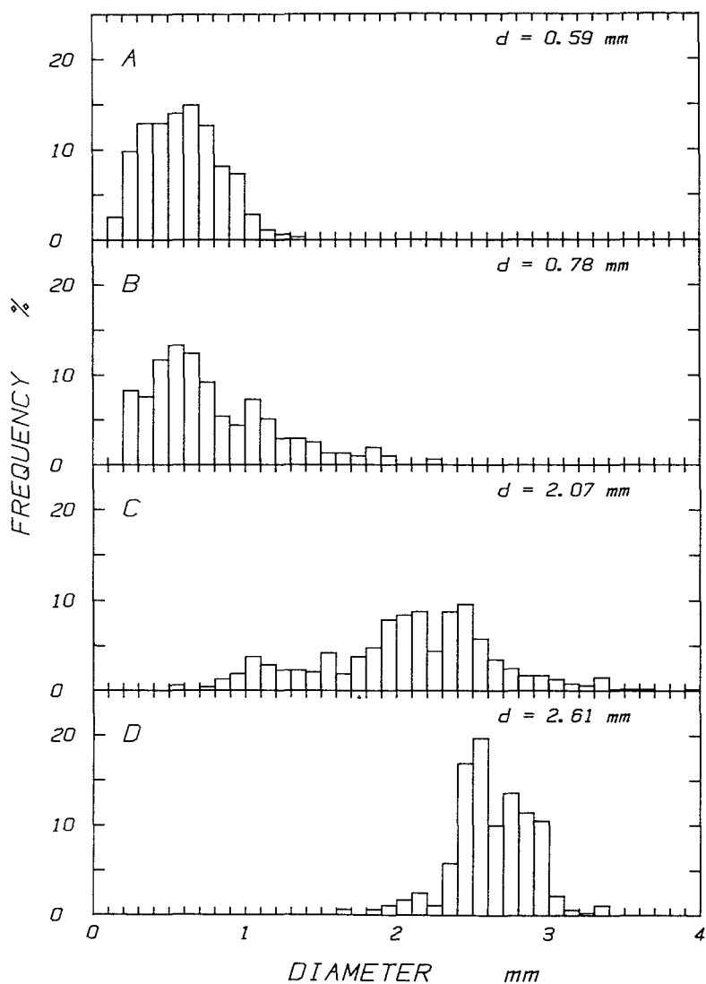
Fig. 26 Histograms of snow particle diameters.
