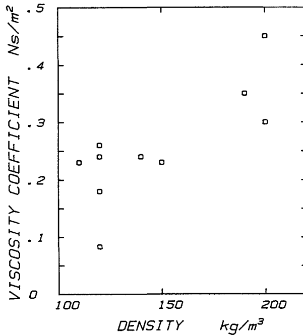
Fig. 21 Apparent viscosity coefficients of fluidized snow flow versus bulk snow densities.
