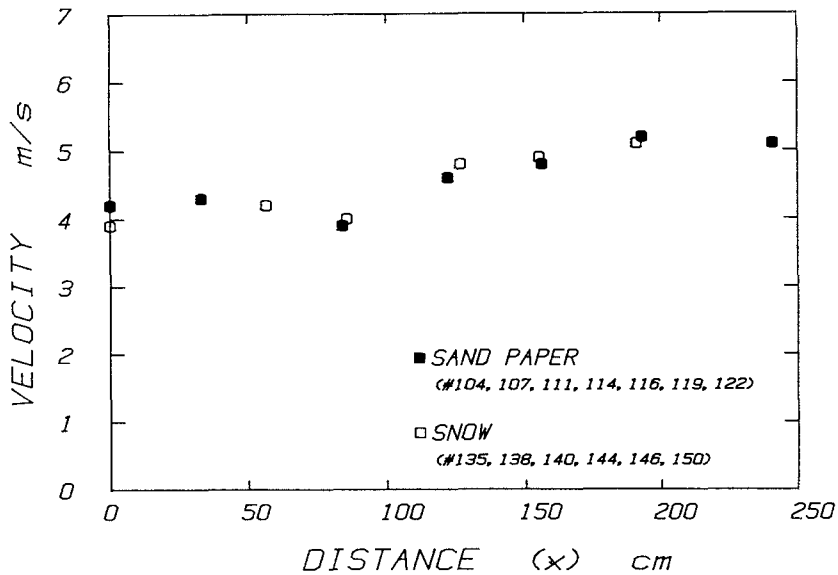
Fig. 13 Change in the snow flow velocity over the inclined chute.
