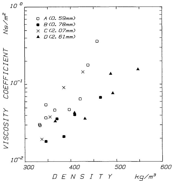
Fig. 31 Viscosity coefficients versus bulk densities for all samples: sample A ( d=0.59\text{ mm} ), B ( d=0.78\text{ mm} ), C ( d=2.07\text{ mm} ) and D ( d=2.61\text{ mm} ).
