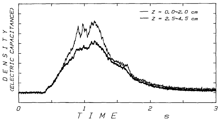
Fig. 36 Typical examples of the electric capacitance data. The unit of the vertical axis is arbitrary.
