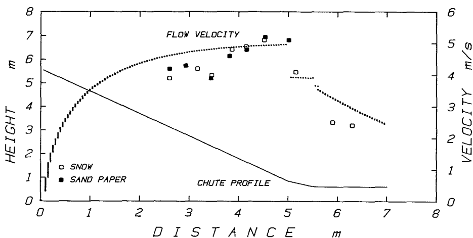
Fig. 43 Observed and calculated snow flow velocities along the inclined chute. Solid line shows the chute profile; Circles show the observed velocities ( \circ : snow floor, \bullet : sand paper floor); Dotted line represents the calculated velocity.
