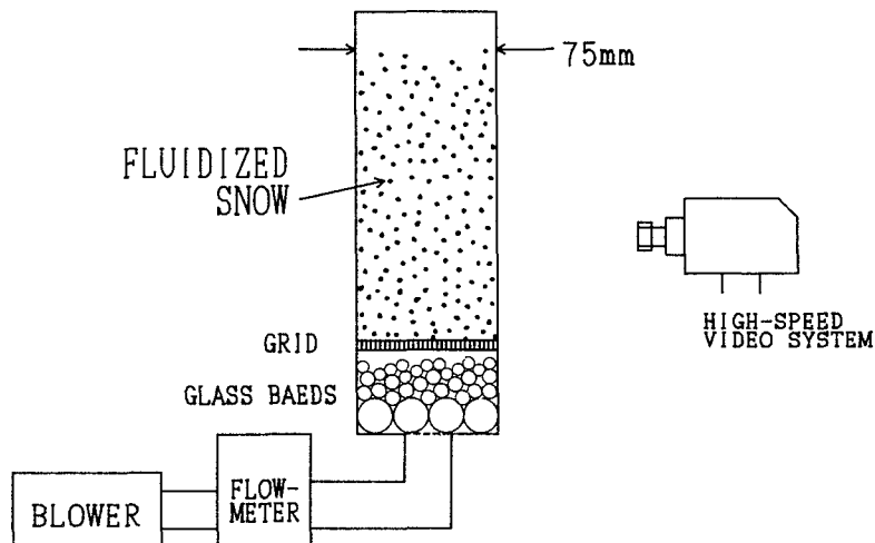
Fig. 22 Schematic diagram of the experimental apparatus for generating the fluidized snow.
