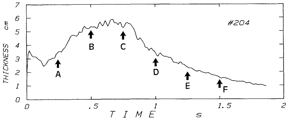
Fig. 11 Variation in snow flow depth with time.
