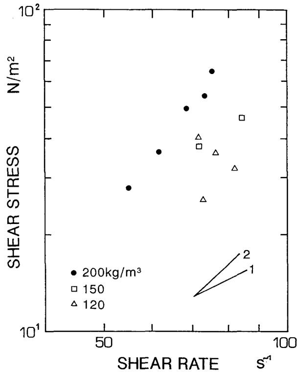
Fig. 34 Relation between the shear stress and the shear rate for the fluidized-snow obtained with the inclined chute experiments.
