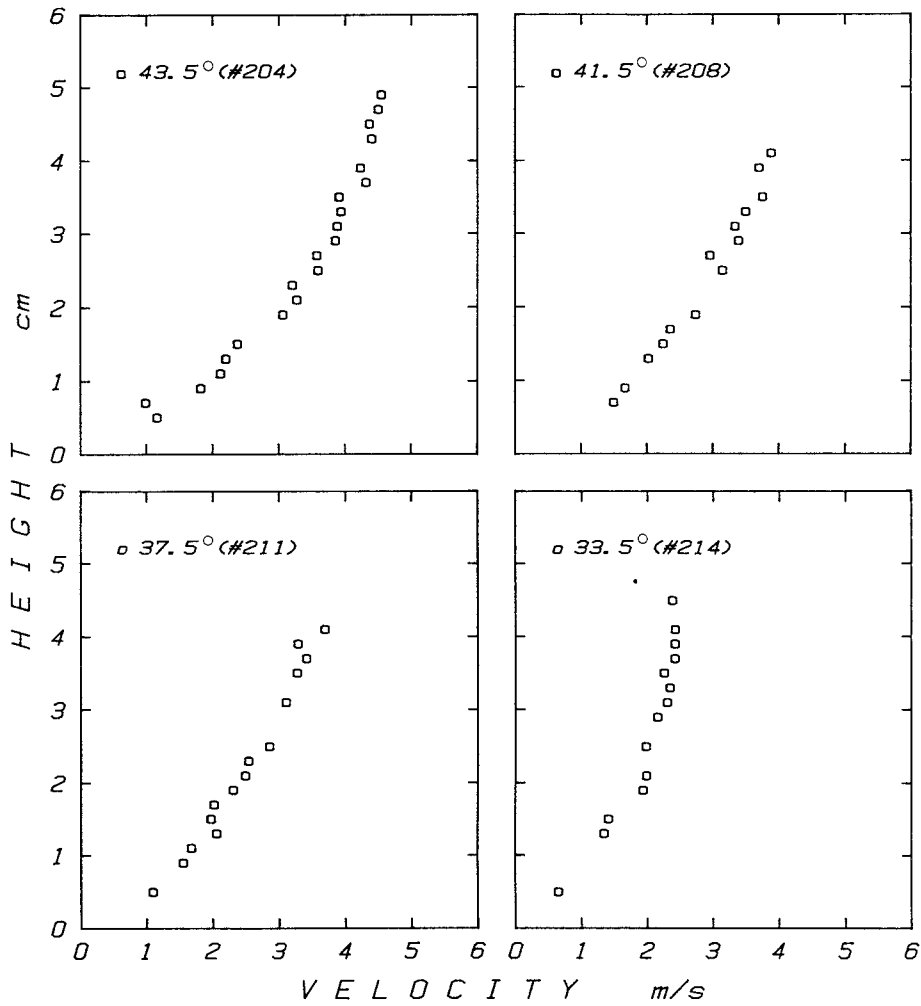
Fig. 14 Velocity profiles at various chute-inclinations.
