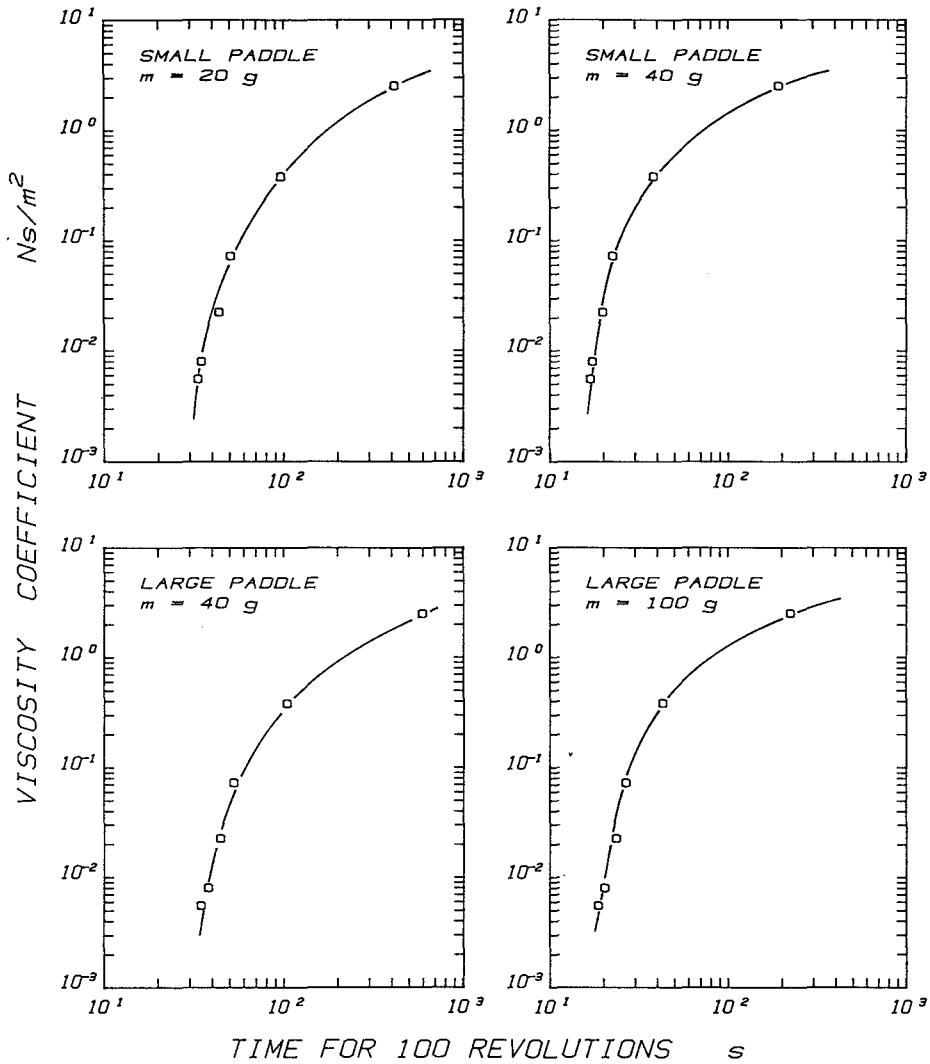
Fig. 25 Viscosity coefficients versus t_{100} measured with the modified Stormer-type viscometer.
