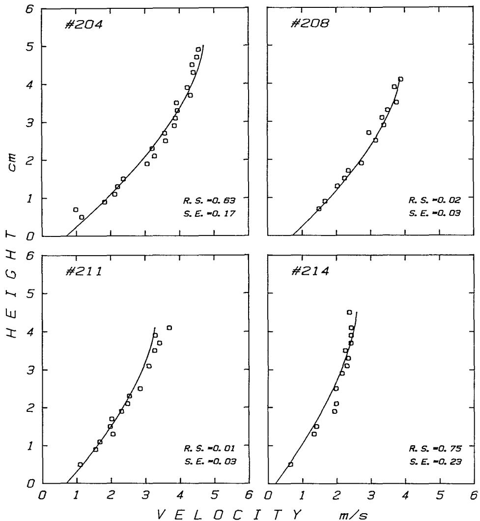
Fig. 37 Measured and calculated velocity profiles of snow flow (4). The solid curves represent the Eq. (21).
