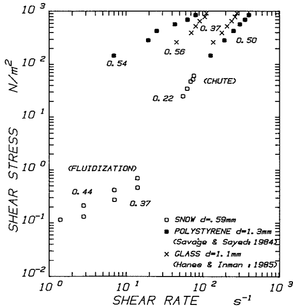
Fig. 40 Comparisons of the fluidized snow properties with polystyrene beads and glass beads ones.
