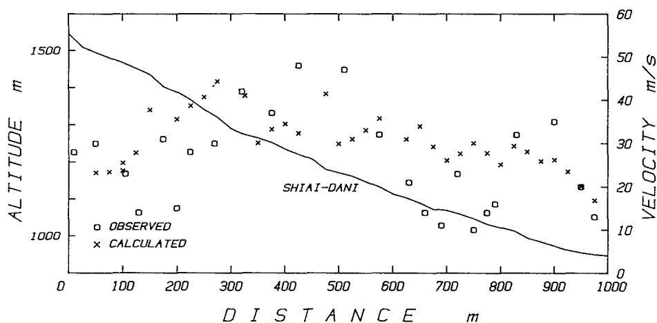
Fig. 44 Observed and calculated avalanche velocities. The avalanche was released artificially on February 1, 1988 at Shiai-dani. Open circles show the velocities of the avalanche front estimated from the video film; Crosses represent calculated avalanche velocity; Solid line is a cross section along the avalanche shoot.
