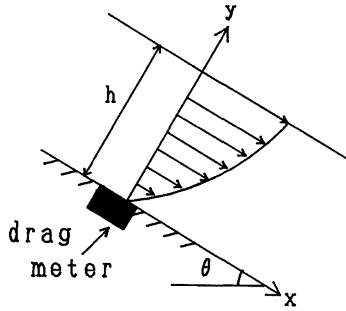
Fig. 17 Two-dimensional snow flow down an inclined chute.
