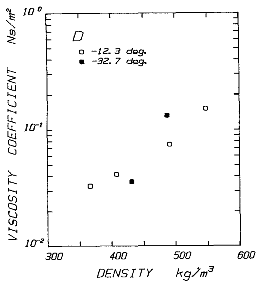
Fig. 30 Viscosity coefficients versus bulk densities for sample D ( d=2.61 mm).
