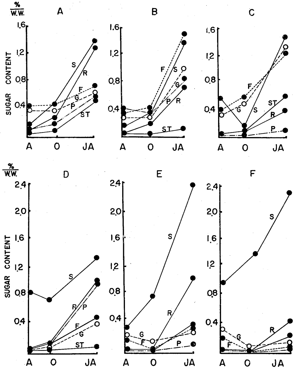
Fig. 3. Seasonal variations in sugars contained in twig bark of various woody plants. A Betula tauschii , B Rosa pendulina , C Larix leptolepis , D Salix koriyanagi , E Populus nigra , F Morus bombycis .
