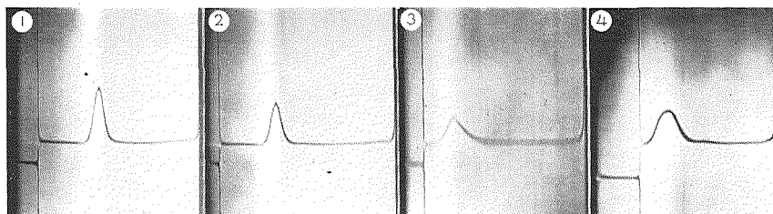
Fig. 1. Sedimentation diagrams of frozen-thawed and freeze-dried catalase 1 Native 32 min after full speed reached. S_{20,w}=11.5 2 Freeze-thawing. Freezing temp. -60^{\circ}\text{C} . 32 min. S_{20,w}=12.4 3 Freeze-drying. Freezing temp. -80^{\circ}\text{C} . 30 min. S_{20,w}=3.8 4 Freeze-drying. Freezing temp. -80^{\circ}\text{C} . 32 min. S_{20,w}=5.8 Protein concentration, 0.42%; Solvent, 0.075 M phosphate buffer (pH 7.0); 55430 r.p.m.; 20^{\circ}\text{C}
