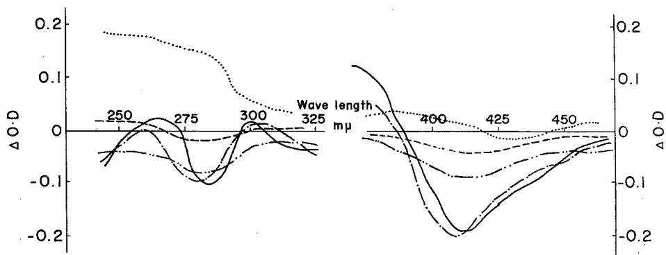
Fig. 6. Difference spectrum of freeze-dried catalase II Effect of the concentration of phosphate buffer solution Concentration of phosphate buffer solution (pH 7.0): —, O; — — —, 7.5 \times 10^{-3} M; - - - - , 1.5 \times 10^{-2} M; - · - · - , 3.7 \times 10^{-2} M; · · · · · , 5.6 \times 10^{-2} M. Protein concentration, 0.14%; Solvent, 7.5 \times 10^{-2} M phosphate buffer (pH 7.0) Reference, non-treated catalase
