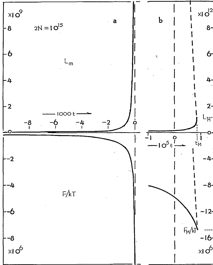
Fig. 6. L_M : total margin length of the group of islands F : free energy of the group. t = (T - T_c)/T_c
