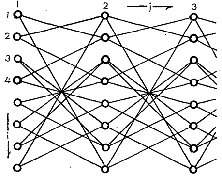
Fig. 9. Each circle represents a "substate" of islands realizable on a column, that is, ridge or groove. The two circles located on adjacent columns and joined by a straight line are two substates which do not conflict with "prohibition of contiguity"
