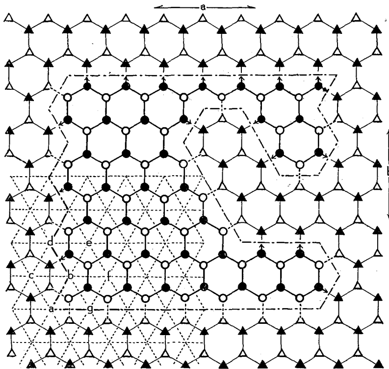
Fig. 1. Arrangement of molecules H_2O on (0001). Molecules are shown by circles and triangles joined by segments representing hydrogen bonds. Triangles, open and solid together, make the original or reference surface. Circles, both open and solid, are the molecules composing a positive island. Molecules of the same shape are assumed to lie evenly to form molecular net planes, although the open ones are actually positioned 0.923 \text{ \AA} above, namely on this side of, the solid ones. The distance between the net planes of circles and triangles measured perpendicular to the plane of paper is 3.694 \text{ \AA} . The two neighbouring molecules of the same shape, for instance open circle and open circle, are 4.524 \text{ \AA} apart
