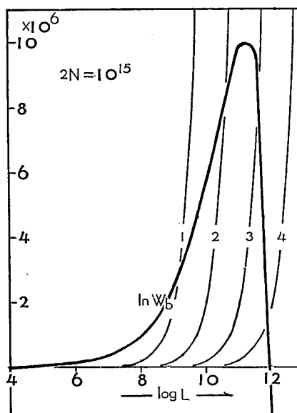
Fig. 5. Curves 1, 2, 3 and 4 stand for [(\epsilon/kT) - \alpha]L for different values of T less than T_c . From this figure it is seen that X/kT = [(\epsilon/kT) - \alpha]L - \ln W_b has a minimum of negative value at a given temperature lower than the critical temperature T_c .
