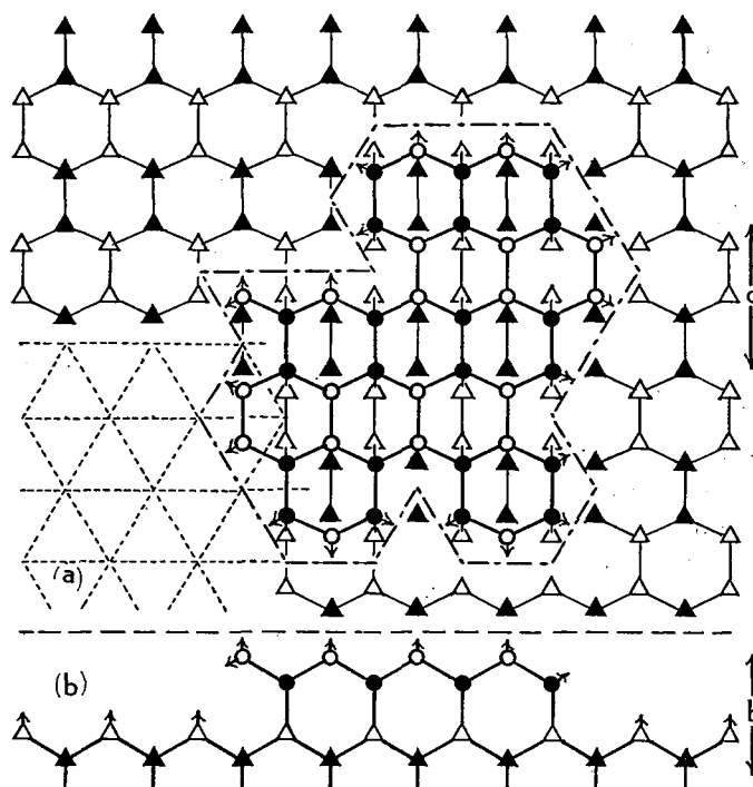
Fig. 2. Arrangement of molecules on (1\bar{1}00) . Figure (a) above the horizontal broken line is the plan while Fig. (b) below that line is the elevation in which the arrangement of molecules is the same as that in Fig. 1. Triangles are assumed to make the original net plane and the circles the net plane of a positive island, although open triangles and circles lie actually 1.306 \text{ \AA} above solid triangles and circles respectively
