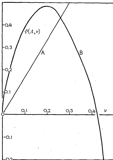
Fig. 10. Straight line A gives [(2T_b/T) - \ln 2]\nu . This figure shows that y = [(2T_b/T) - \ln 2]\nu - \psi(A, \nu) has a minimum of negative value at any temperature T
