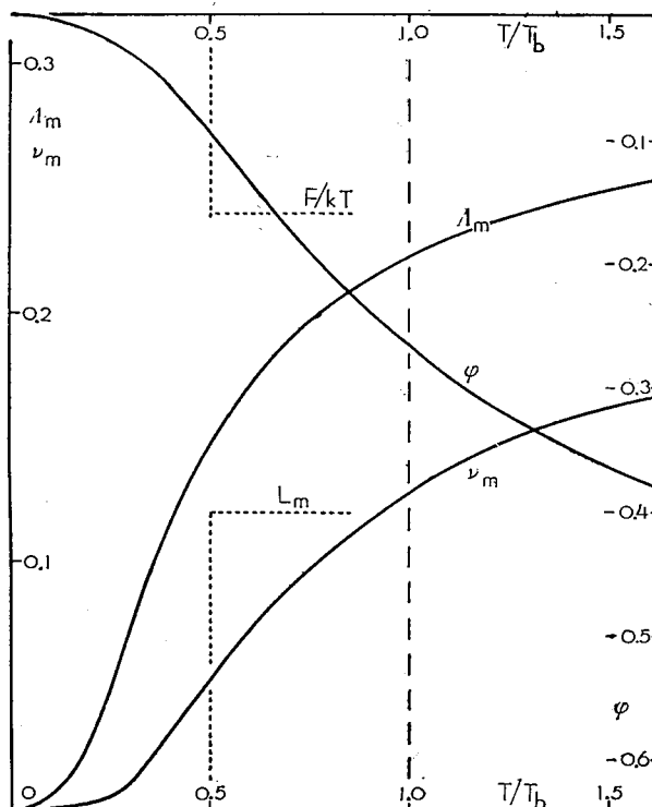
Fig. 11. \phi : free energy per molecule on (11\bar{2}0) divided by kT . \phi = -0.640 at T = \infty . \nu_m : mean number of islands on a column of Fig. 8 per unit length of it, vertical distance between two successive dots and circles on a column, which is 1.847 \text{ \AA} long. \nu_m = 0.240 at T = \infty . A_m : mean number of circles of Fig. 8 per unit length of the column. A_m = 0.304 at T = \infty . Ratio l_m = A_m/\nu_m gives the mean number of molecules composing an island. Dotted curves F/kT and L_m : schematic curves for the free energy and the roughness of surfaces (0001) and (1\bar{1}00)
