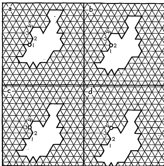
Fig. 4. Islands of the same shape but different in position
