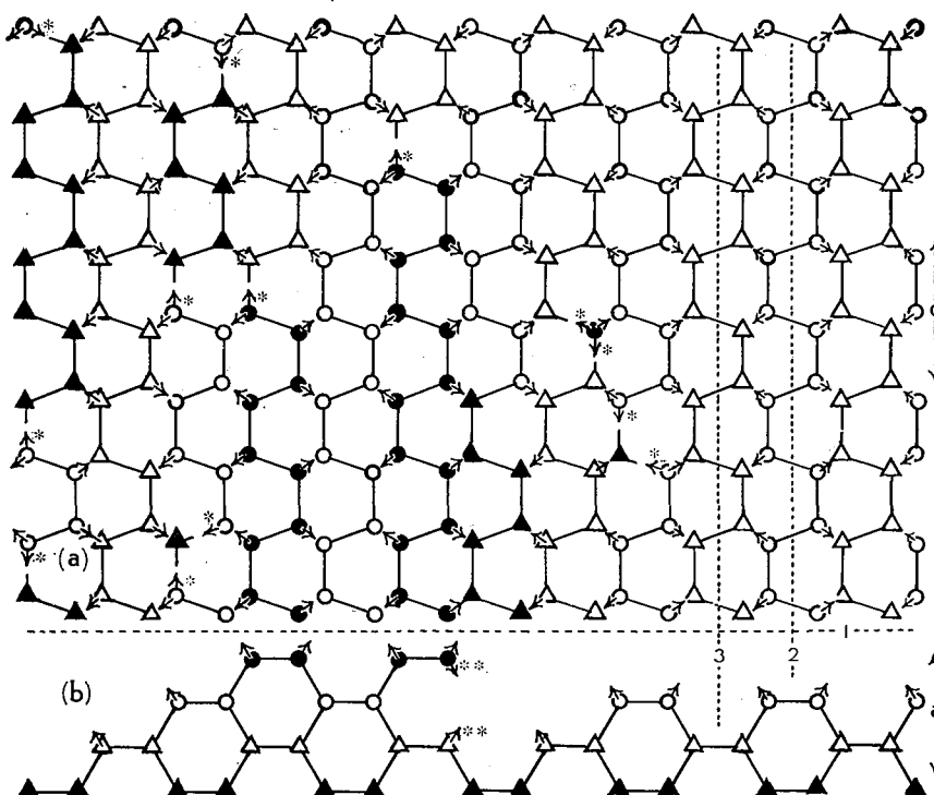
Fig. 7. Molecular arrangement of ( 11\bar{2}0 ). Open circles and triangles form the original surface. Solid circles and triangles make respectively positive and negative islands. Distance between dotted lines 2 and 3, central lines of ridge and groove respectively, is 3.9178 \text{ \AA} . Figure (b), the bottom figure, shows the side view of the surface. In this figure molecules are arranged in such a way as to form net plane of ( 0001 )
