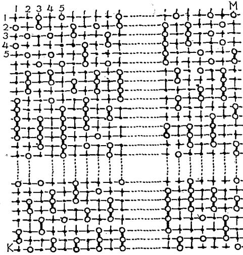
Fig. 8. The circles are the molecules composing islands while dots are those on the original surface. Columns composed of dots and circles represent alternately ridge and groove on (11 \bar{2} 0). The group of circles connected by thick segments forms an island
