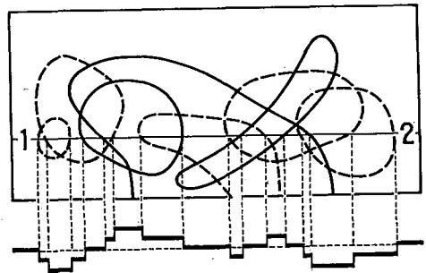
Fig. 3. Closed curves of full line represent positive islands while those of broken line negative islands. The islands overlap one another and give the crystal surface a rough structure. The bottom figure shows the side view of the section made along line 1-2
