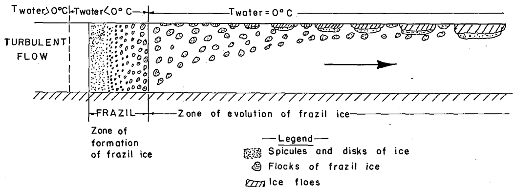
Fig. 4. Evolution of frazil ice in rivers
