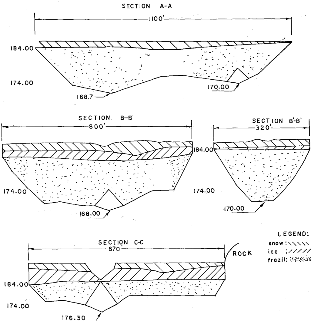
Fig. 8. Deposit of frazil ice in a reservoir, Charny-Chaudière River. Winter 1964
