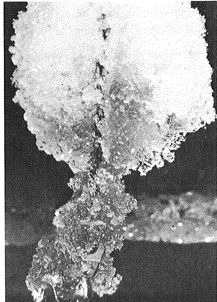
Agglomeration of new frazil flocks on a rope
