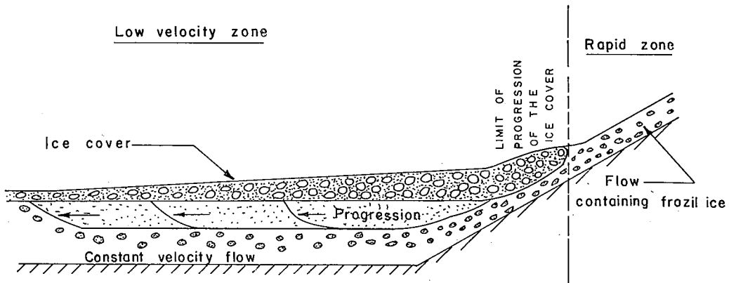
Fig. 7. Hanging dam at the foot of a rapid and progressive deposit of frazil ice downstream
