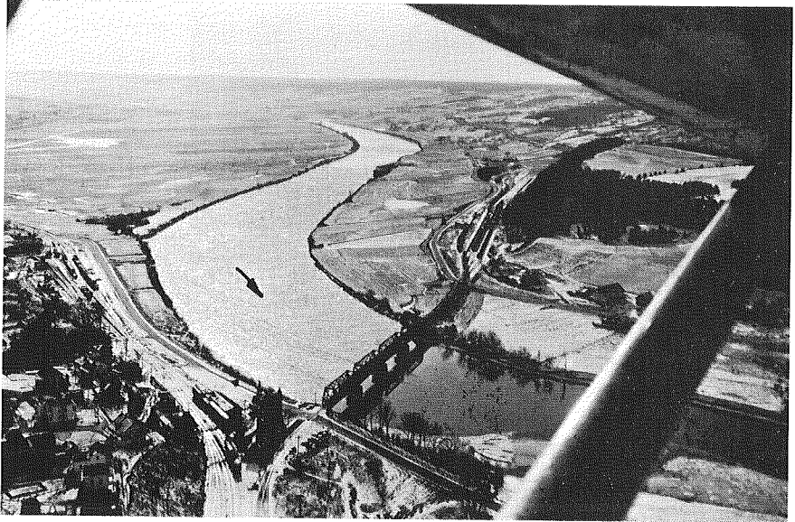
Ice cover initiated at a bridge pier
