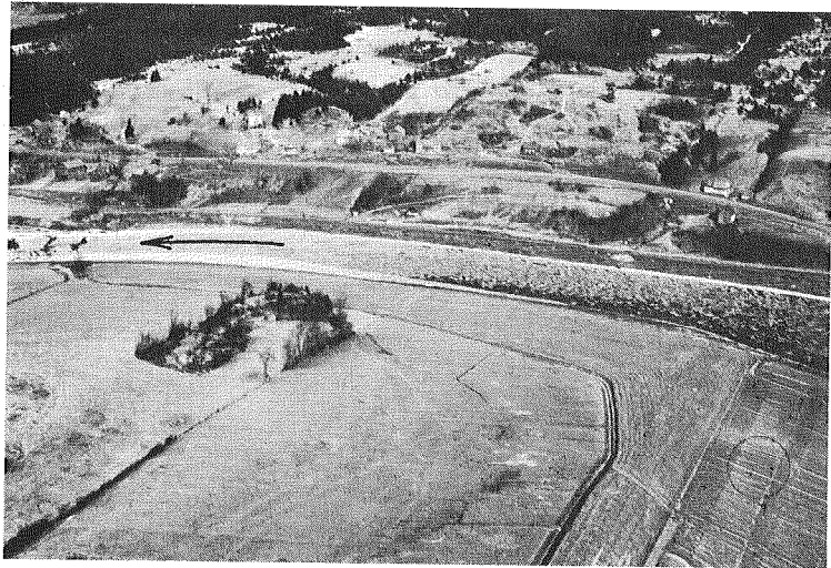
Fig. 6. Beginning of an ice cover with floes coming from frazil ice evolution. Chaudière River. December 1963
