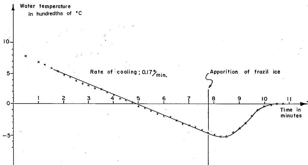
Fig. 1. Evolution of water temperature during the formation of frazil ice
