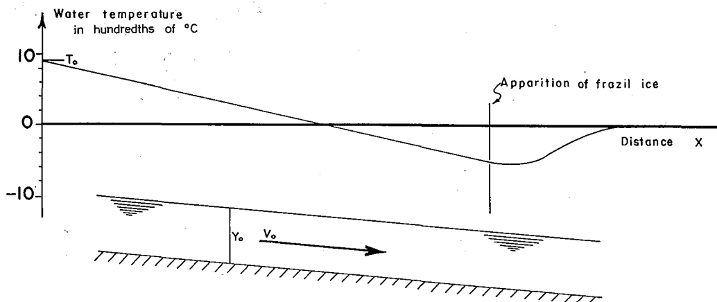
Fig. 3. Evolution of water temperature along the axis of a uniform flow
