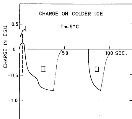
Fig. 13. Electrification in middle range
