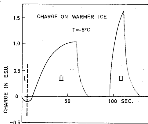
Fig. 14. Electrification in middle range
