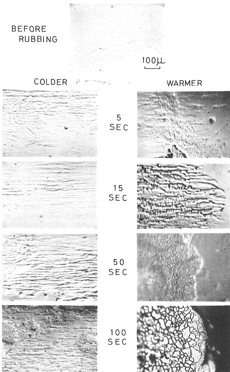
Fig. 10. Change of contact surface due to rubbing ( T = -16^{\circ}\text{C} )
