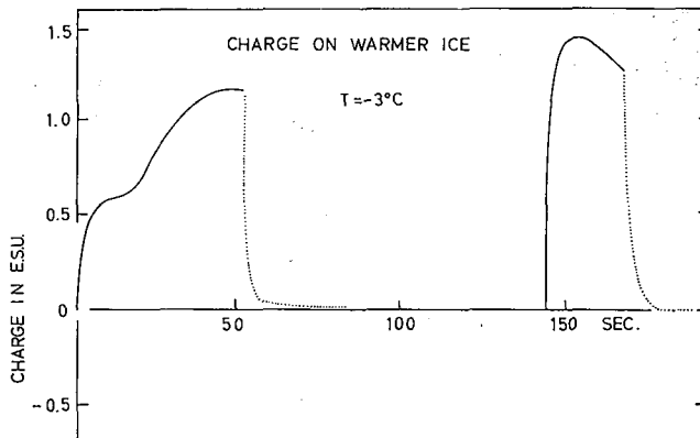
Fig. 16. Electrification in warm range
