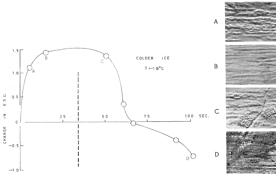
Fig. 11. Change of contact surface of colder ice
