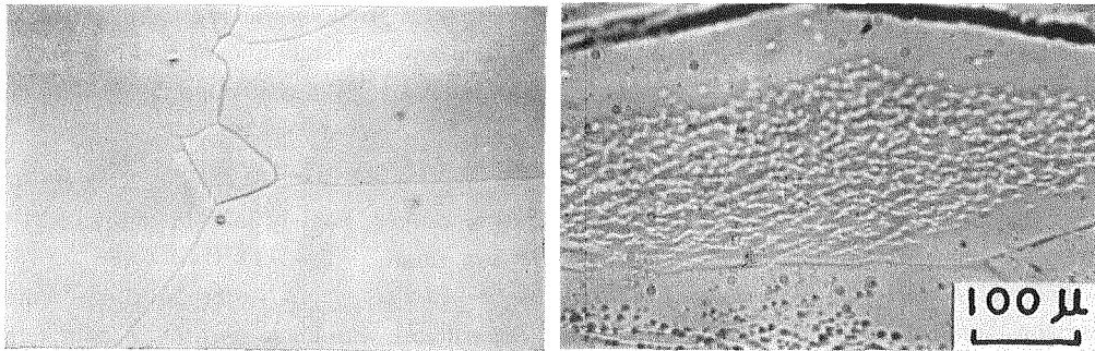
After 4 hrs After 24 hrs Fig. 2. Natural change in surface of ice due to evaporation
