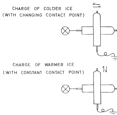
Fig. 3. Asymmetric rubbing of ice against ice
