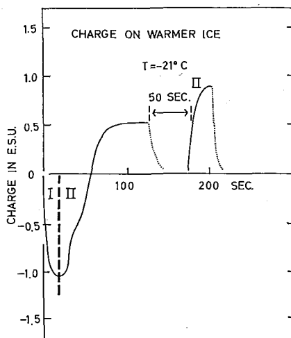
Fig. 7. Occurrence of 2nd stage
