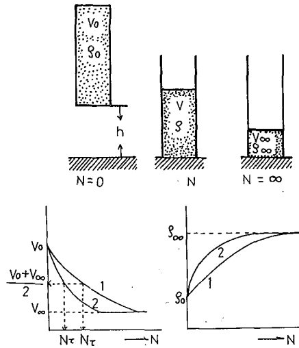
Fig. 12. Schematic diagrams of compaction process of snow by tapping
