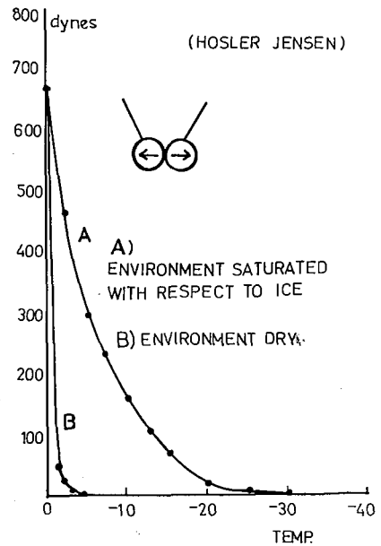
Fig. 9. Temperature dependence of cohesive force between two ice spheres (Hosler and Jensen, 1957)
