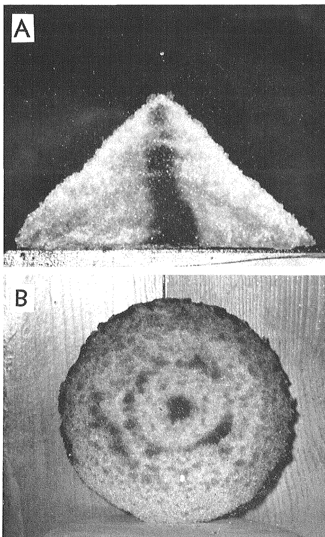
Fig. 11. Cross sections of snow cones. A: Vertical, B; Horizontal
