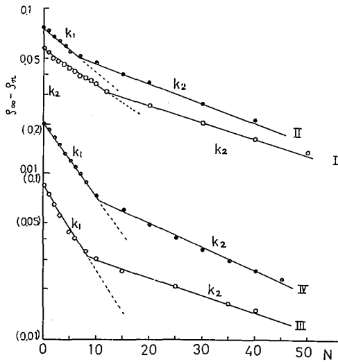
Fig. 16. Density change against tapping number N
