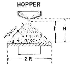
Fig. 5. Definition of angle of repose
