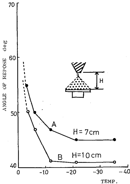
Fig. 8. Temperature dependence of angle of repose of pulverized snow
