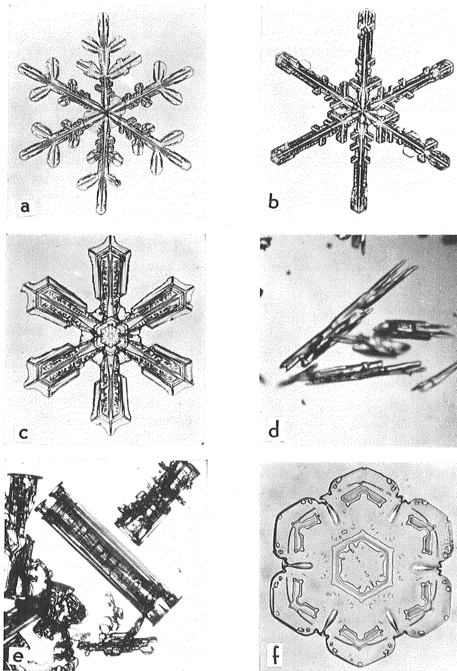
Fig. 2. Surface irregularities of various kinds of snow crystals
