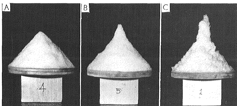
Fig. 7. Temperature dependence of angle of repose of pulverized snow A: -35^\circ\text{C} , B: -3.5^\circ\text{C} , C: 0^\circ\text{C}
