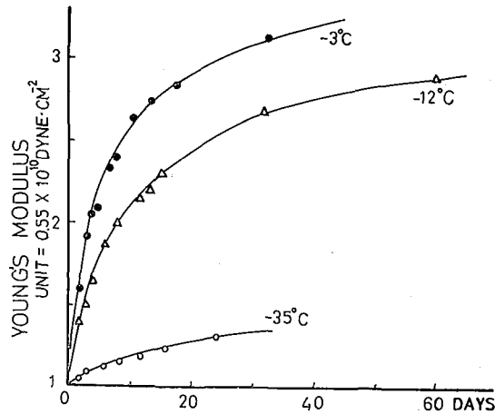
Fig. 19. Change of Young's modulus with sintering time and temperatures
