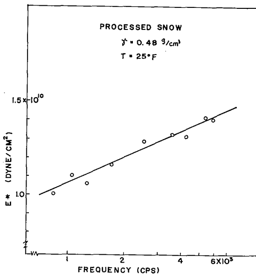
Fig. 9. Loss factor vs. frequency
