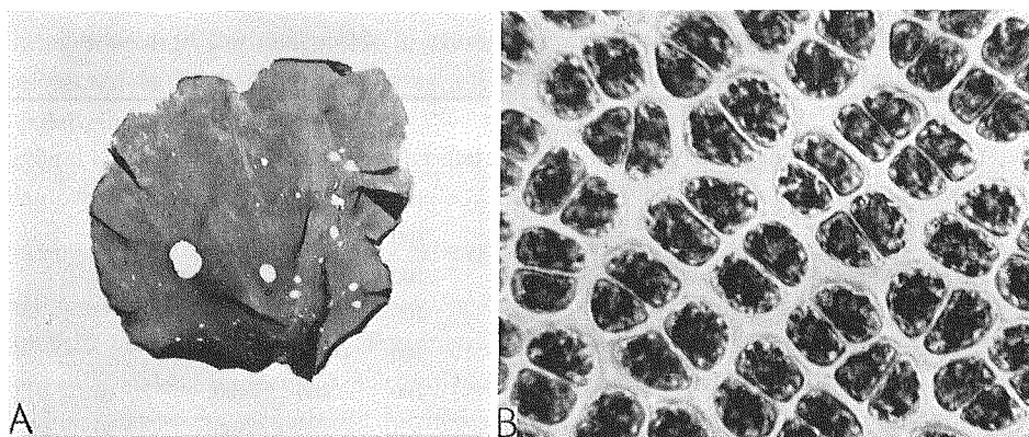
Fig. 9. A marine red alga, Porphyra yezoensis A: A thallus. \times 1 B: Cells in a thallus. \times 625
