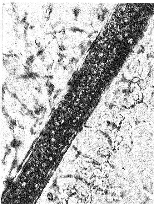
Fig. 7. A filamentous cell of lake ball, extracellularly frozen in 2M methanol at -18^{\circ}\text{C} . Note the unchanged appearance of the frozen cell. Freezing is entirely innocuous to the cell. \times 350
