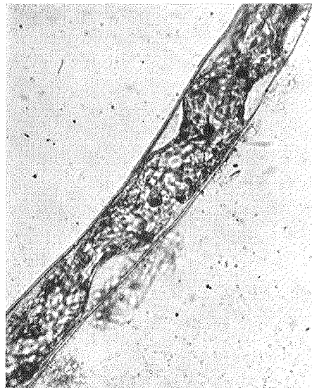
Fig. 2. A filamentous cell of lake ball plasmolysed in 1 M balanced salt solution at room temperature. \times 280
