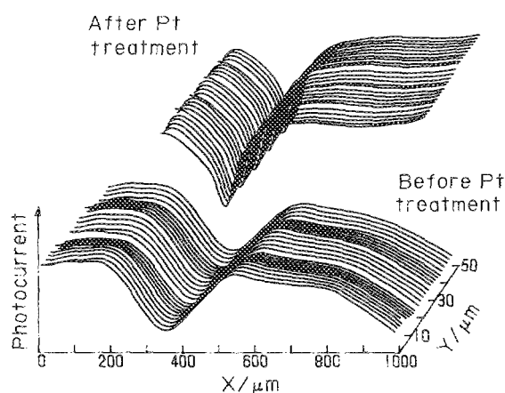
FIG. 2. Line plot showing the laser spot photocurrent across a step on an InSe electrode before (lower lines) and after Pt treatment (upper lines).
