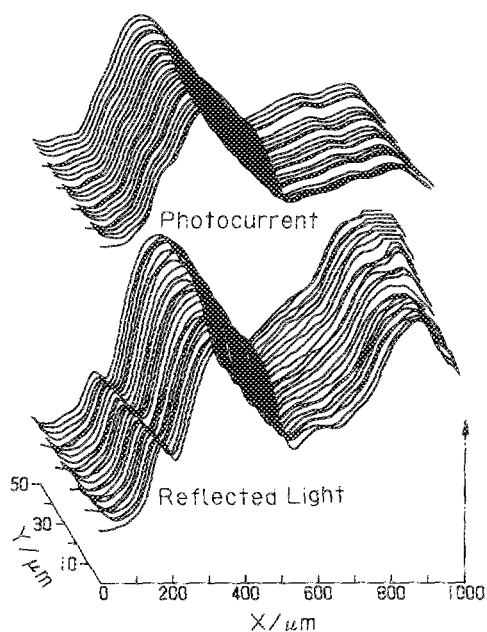
FIG. 4. Reflected light (lower lines) and laser spot photocurrent (upper lines) from the same area. The increase in photocurrent is correlated with an increase in the intensity of the reflected light.
