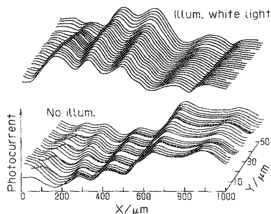
FIG. 3. Line plot of the laser spot photocurrent when the electrode is simultaneously illuminated with white light (upper lines) and without white light illumination (lower lines).
