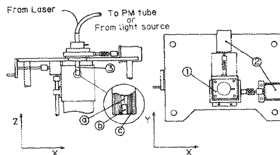
FIG. 1. Experimental configuration. (1) X - Y coordinate table. (2) Step motors. (3) Laser spot probe with (a) single-mode optical fiber, (b) Selfoc microlens, and (c) assembly of optical fibers.
