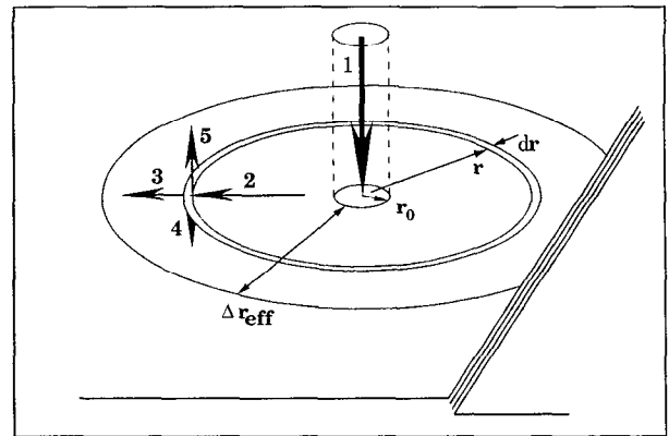
FIG. 4. Schematic diagram of the illuminated area ( r < r_0 ) and the charged disk ( r < r_0 + \Delta r_{eff} ), illustrating the elementary processes (1–5) in our model, and showing the truncation of the charged disk when approaching a step in the surface.
