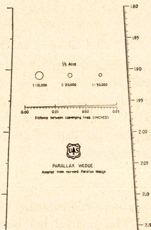
3. Parallax wedge.
