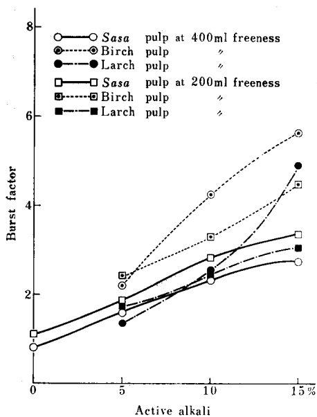
Fig. 11. Burst factor of the pulps and active alkali at 160°C.
