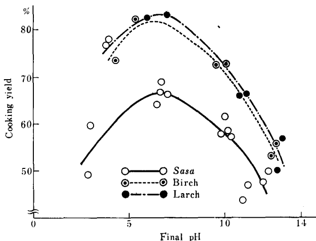
Fig. 4. Cooking yield and final pH.
