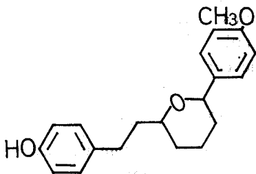
XIII Centrolobine ( Centrolobium : Leguminosae )
