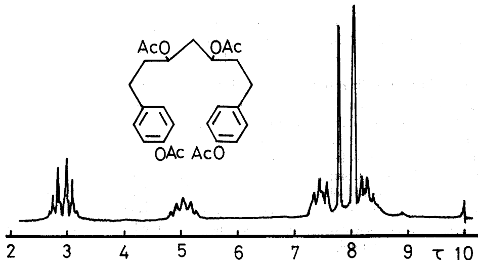
Fig. 15. NMR spectrum of E-3 (1,7-di-( p -hydroxyphenyl)-heptane-3,5-diol) tetraacetate.
