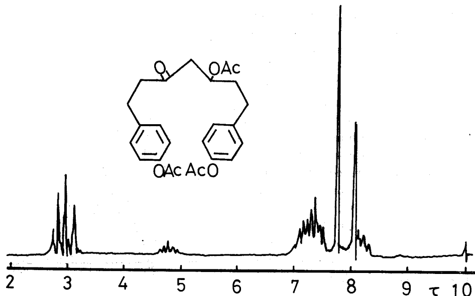
Fig. 19. MNR spectrum of E-4 (1,7-di-( p -hydroxyphenyl)-heptane-3-one-5-ol) triacetate.
