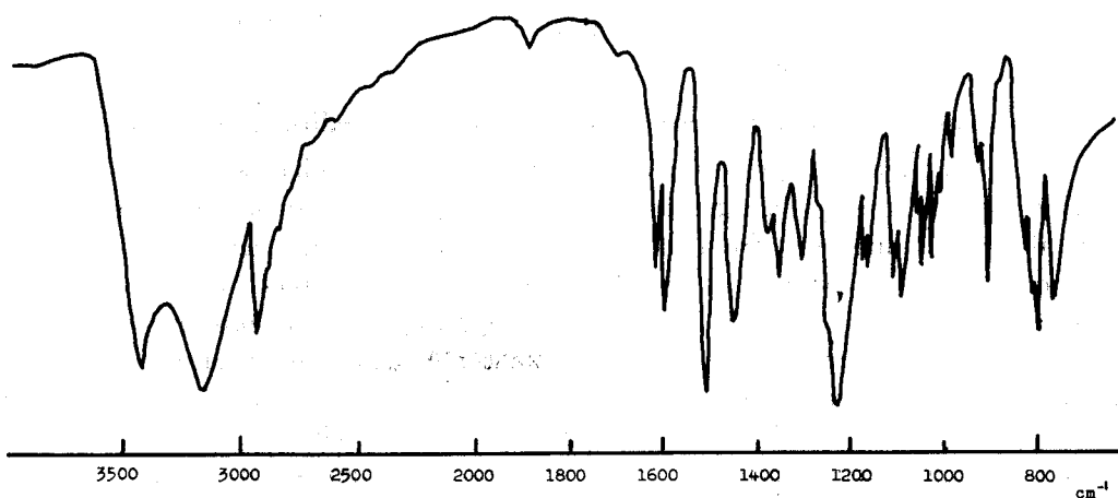
Fig. 14. Infra red absorption spectrum of E-3 (1,7-di- p -hydroxyphenyl)-heptane-3,5-diol).
