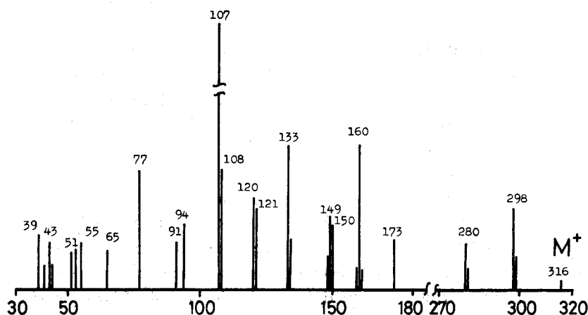
Fig. 16. Mass spectrum of E-3 (1, 7-di-( p -hydroxyphenyl)-heptane-3, 5-diol)
