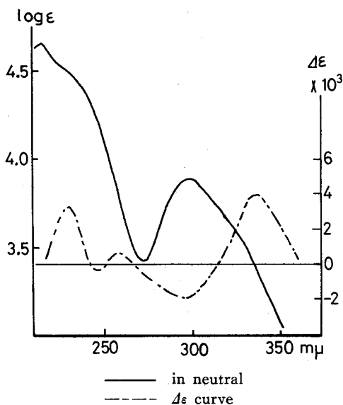
Fig. 1. Ultra violet absorption spectrum and its \Delta\epsilon curve of E-1 (trideoxysadanin-8-ene).
