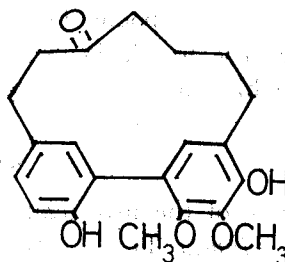
XIV Myricanone ( Myrica : Myricaceae )
