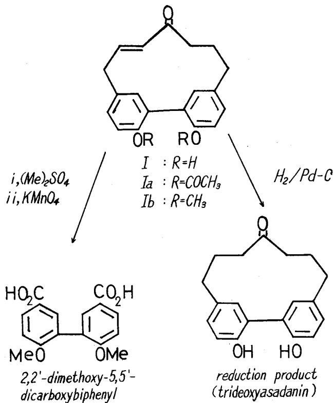
Fig. 3. Degradation and reduction products from E-1.
