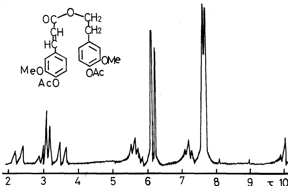
Fig. 10. NMR spectrum of E-2 diacetate.
