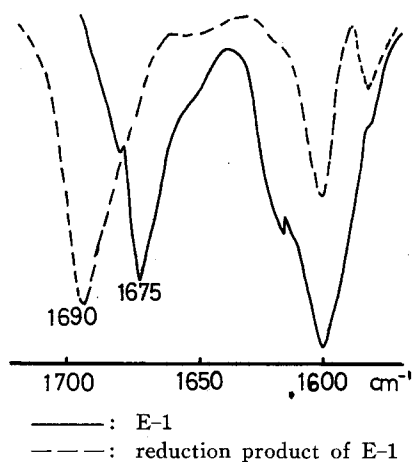
Fig. 2. Carbonyl bands in Infra red absorption spectra of E-1 and reduction product.
