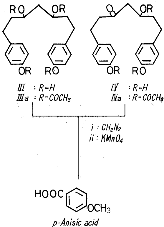
Fig. 12. Degradation product from methyl ether of E-3 and E-4 with potassium permanganate.
