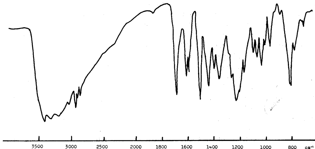
Fig. 18. Infra red absorption spectrum of E-4 (1,7-di- p -hydroxyphenyl)-heptane-3-one-5-ol)
