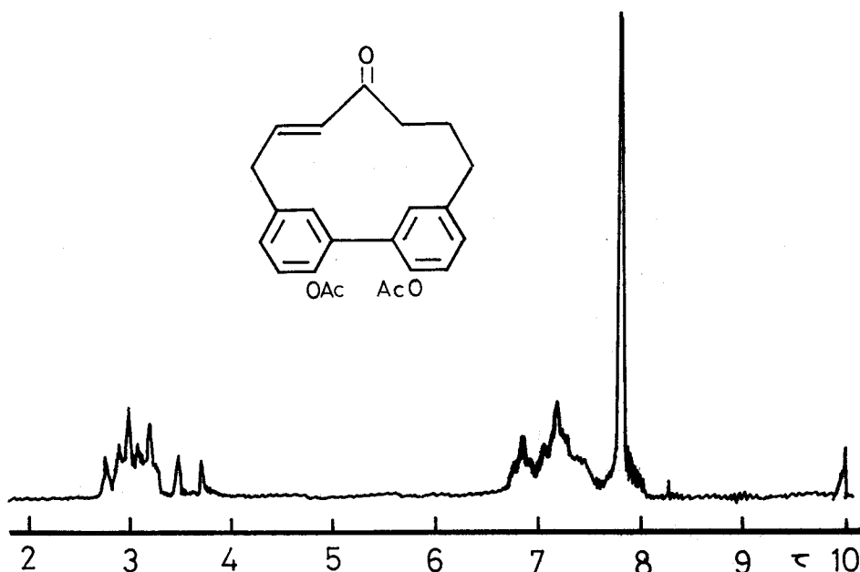
Fig. 5. NMR spectrum of E-1 diacetate.
