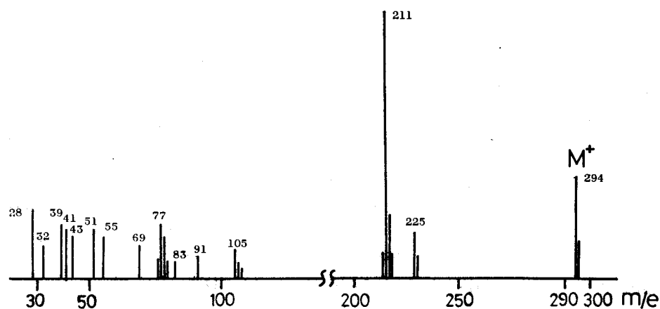
Fig. 4. Mass spectrum of E-1 (trideoxyasadanin-8-ene).
