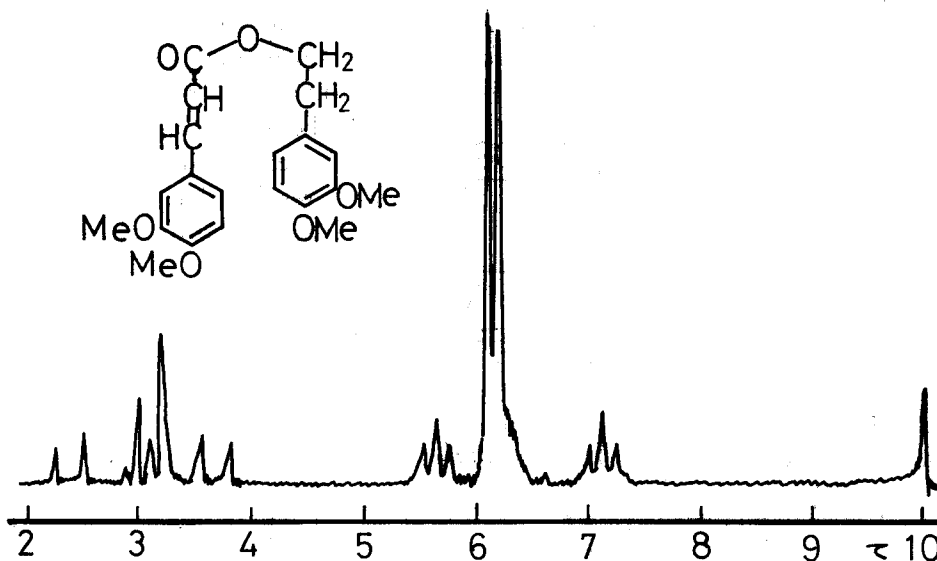
Fig. 11. NMR spectrum of E-2 dimethyl ether.
