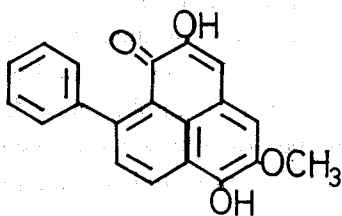
XV 9-Phenylperinaphthenone ( Lachnanthes : Haemodoraceae )
