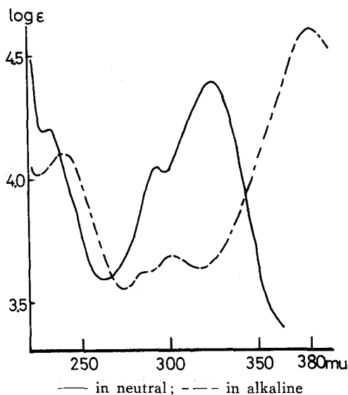
Fig. 6. Ultra violet absorption spectra of E-2 ( \beta -guaiacyl ethyl ferulate). — in neutral; --- in alkaline
