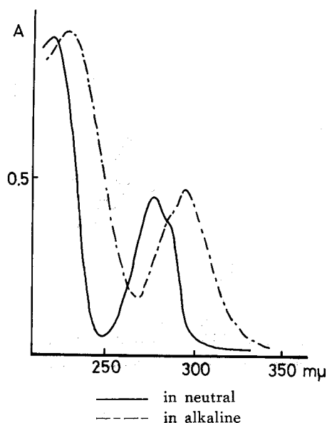
Fig. 17. Ultra violet absorption spectra of E-4 (1,7-di- p -hydroxyphenyl)-3-one-5-ol).
