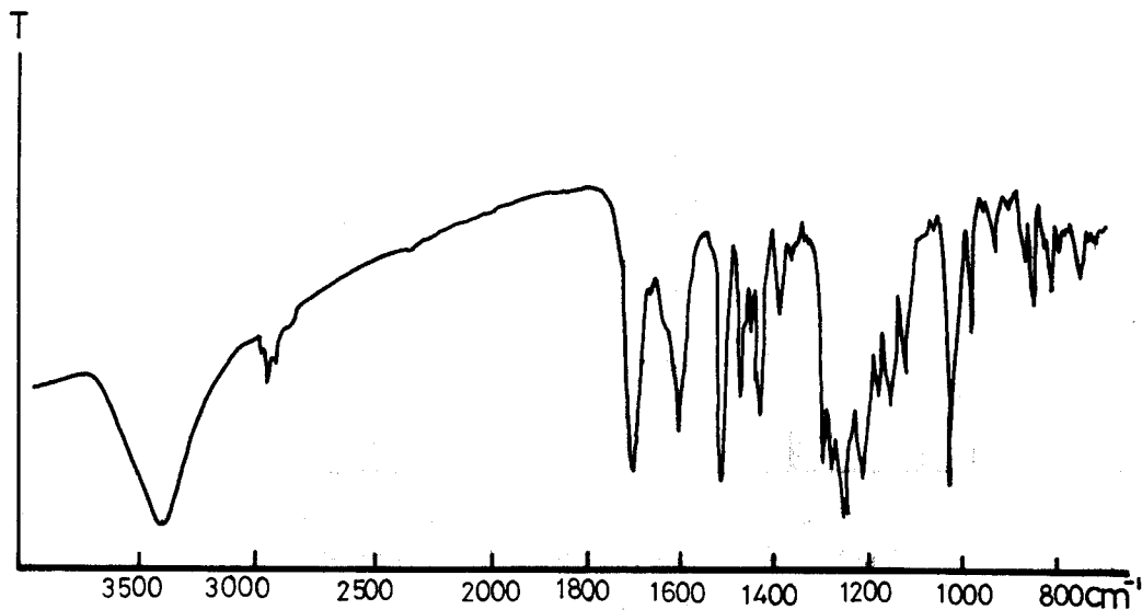
Fig. 7. Infra red absorption spectrum of E-2 ( \beta -guaiacylethyl ferulate).
