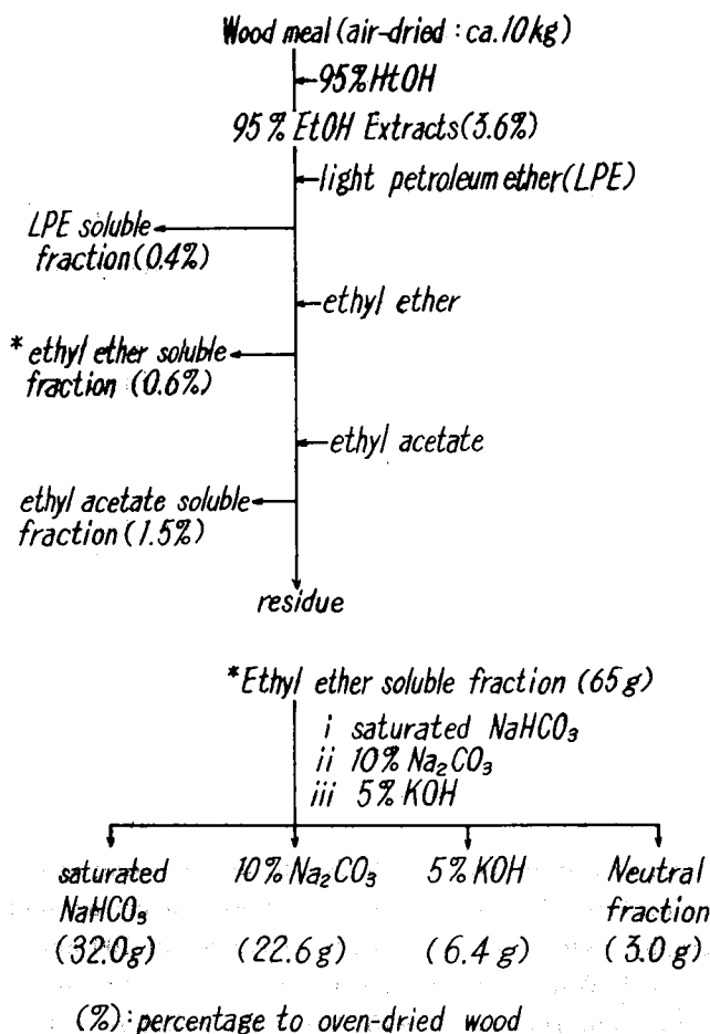
Fig. 24. Separation scheme of extracts from the wood of Alnus hirsuta TURCZ.
