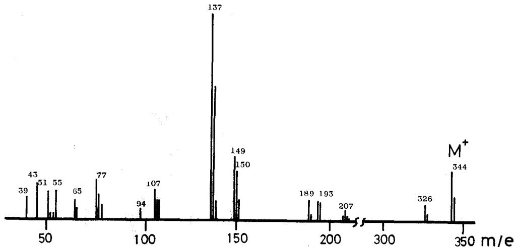
Fig. 9. Mass spectrum of E-2 ( \beta -guaiacyl ethyl ferulate).
