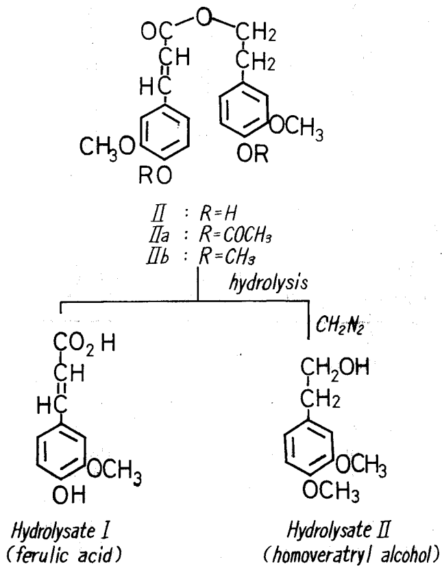
Fig. 8. Hydrolysates from E-2 with alcoholic potassium hydroxide.
