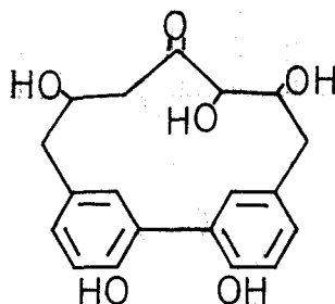
XI Asadanin ( Ostrya japonica )
