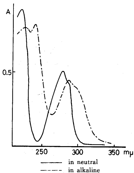
Fig. 13. Ultra violet absorption spectra of E-3 (1,7-di- p -hydroxyphenyl)-heptane-3,5-diol).
