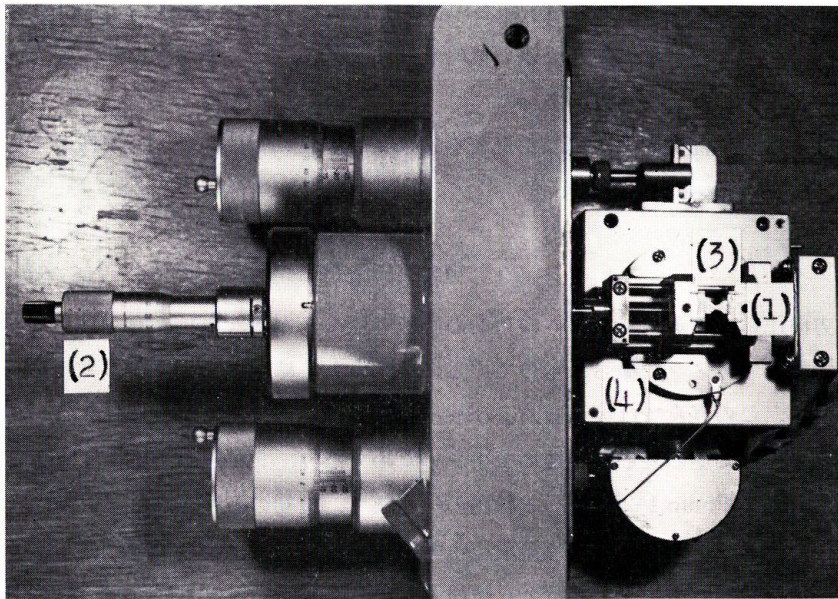
Fig. 2. Specimen stage.
