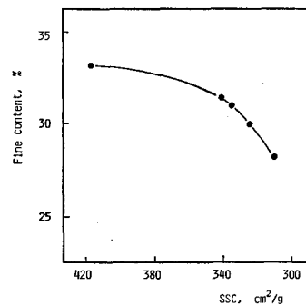
Fig. 14. Specific Scattering Coefficient (SSC) as a Function of Fine Content of Pulp from the Pretreated Chips.
