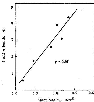
Fig. 5. Sheet Density as a Function of Breaking Length of Pulps from the Untreated and Pretreated Chips.
