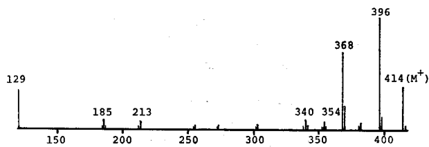
Fig. 33. Mass Spectrum of Compound P 4 ( \beta -Sitosterol).
