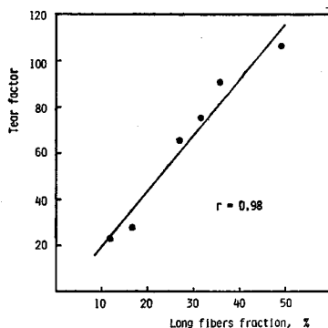
Fig. 7. Relationship between Long Fibers Fraction and Tear Factor of Pulps from the Untreated and Pretreated Chips.
