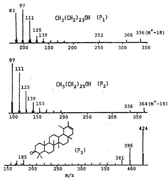
Fig. 32. Mass Spectra of Compounds P 1 (1-Tetracosanol), P 2 (1-Hexacosanol), and P 3 ( \psi -Taraxasterone).
