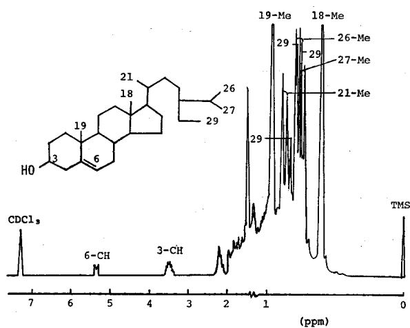
Fig. 34. NMR Spectrum and Chemical Structure of Compound P 4 ( \beta -Sitosterol).
