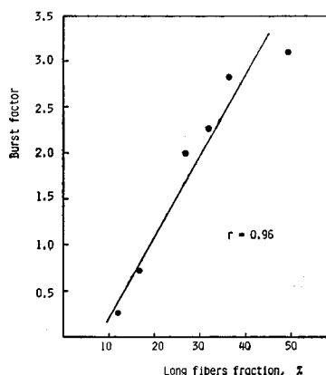
Fig. 8. Relationship between Long Fibers Fraction and Burst Factor of Pulps from the Untreated and Pretreated Chips.
