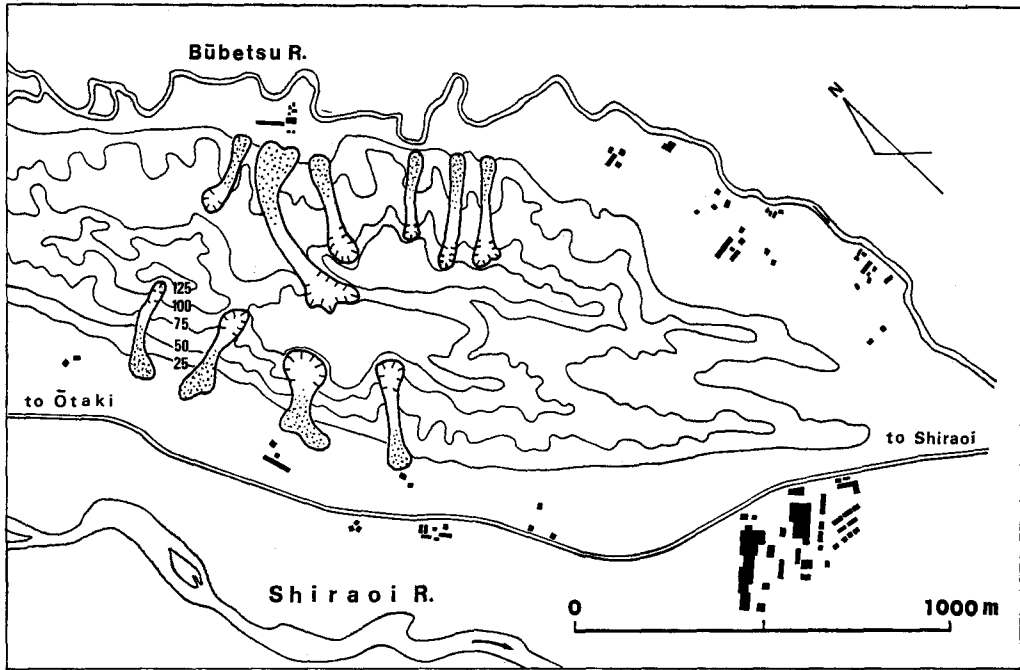
Fig. 12. Slope failure in Shiraoi at 1979.
