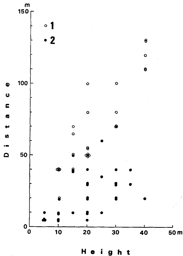
Fig. 24. Relationship between the height of slope failure( h ) (the length from the foot of slope to the top of scar) and the length of debris ( l ) (distance from the foot of slope to the end of debris deposit).
