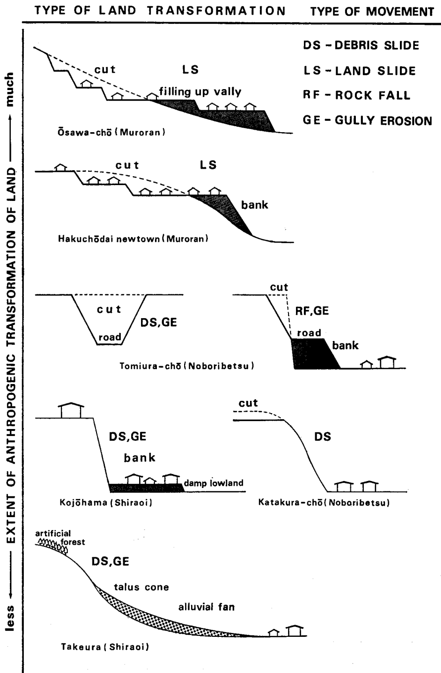
Fig. 22. Classification of land transformation and slope failure.
