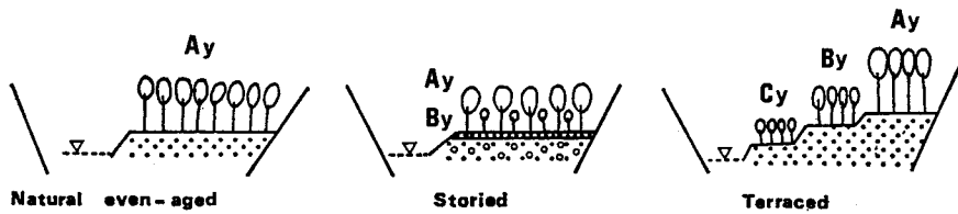
Fig. 3. Typical forests on the stepped deposits (ARAYA, 1982).
