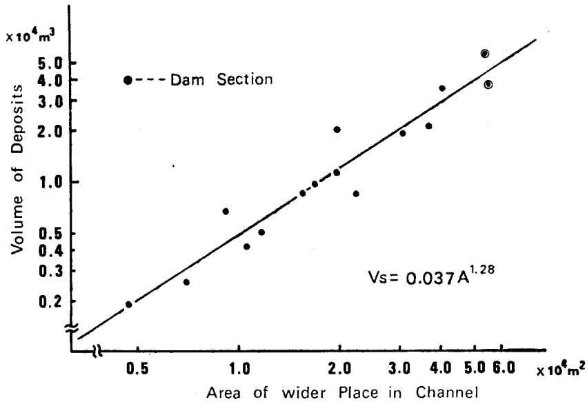
Fig. 17. The relation between the area of channel bed and the volume of sediment.
