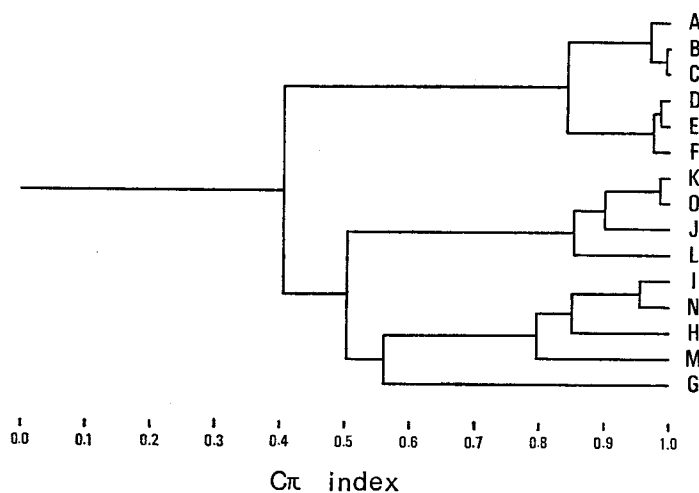
Fig. 3. The UPGMA clustering of trap sites based on the faunal similarities estimated by C_x index.
