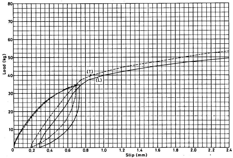
Fig. 3. Effect of the grain direction of main-member.
