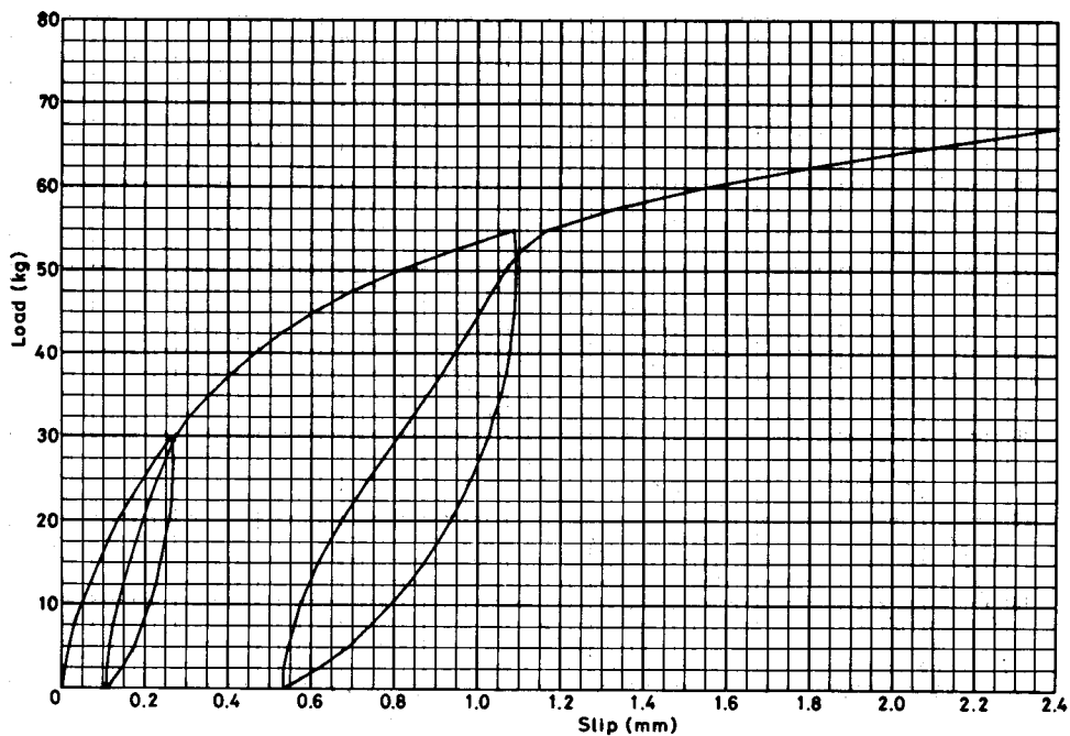
Fig. 5. (9) Continued. (Hem-fir 204 and Kapor 9 mm plywood)
