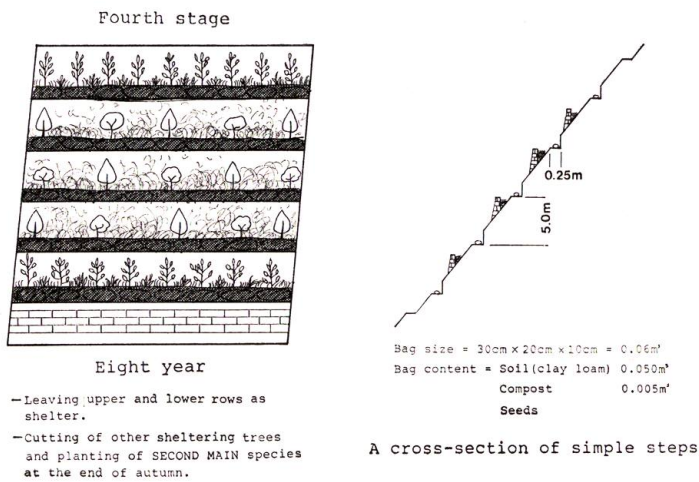
Fig. 31 c. Planting of first and second main tree species in highly disturbed hillslope.
