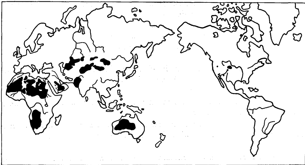
Fig. 3. World distribution of desert big active and fixed Pleistocene sand dune fields.
