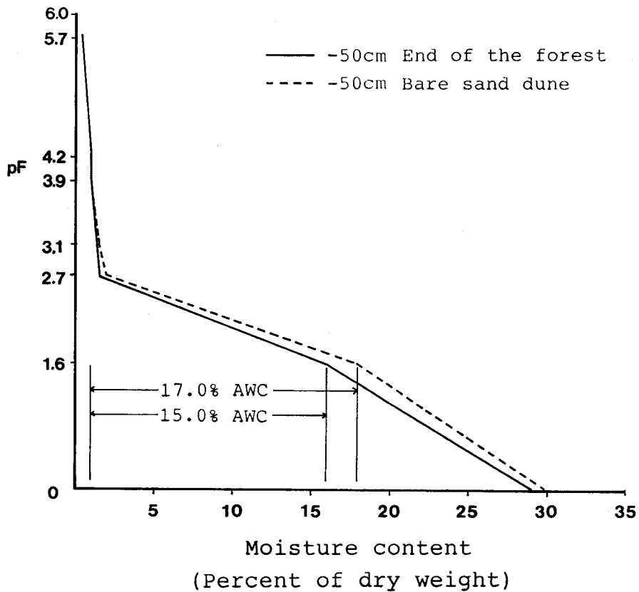
Fig. 21 d. Soil moisture retention characteristics of 50 cm deep layers in Sunasaka.
