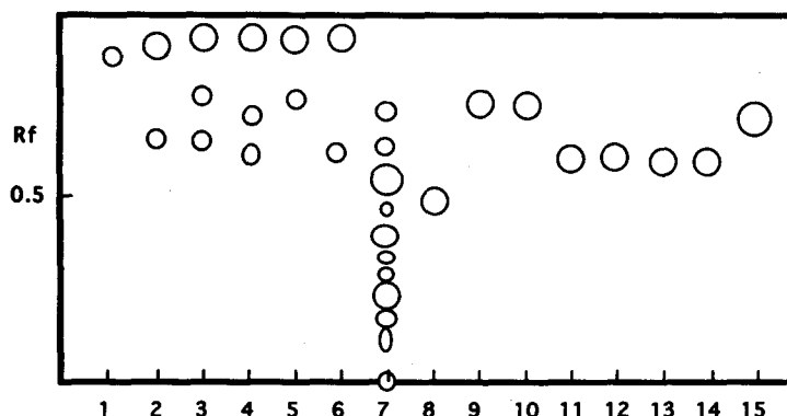
Fig. 2 Thin layer chromatograms of monoterpenes and LPE-sol from the bark of M. kobus DC. var. borealis Sarg. 1: camphene, 2: \alpha -pinene, 3: dl -limonene, 4: 3-carene, 5: \beta -pinene, 6: d -limonene, 7: LPE-sol, 8: fenchone, 9: d -camphor, 10: isobornyl acetate, 11: \alpha -terpineol, 12: (+)-terpinen-4-ol, 13: citronellol, 14: nerol, 15: \alpha -tocopherol. Developing solvent was n-hexane: acetone (2 : 1, v/v).
