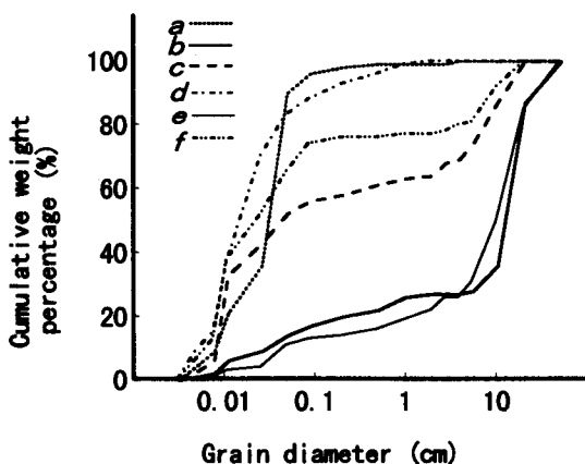
Fig. 5 Particle size distribution of soil samples expressed by cumulative weight curves.
