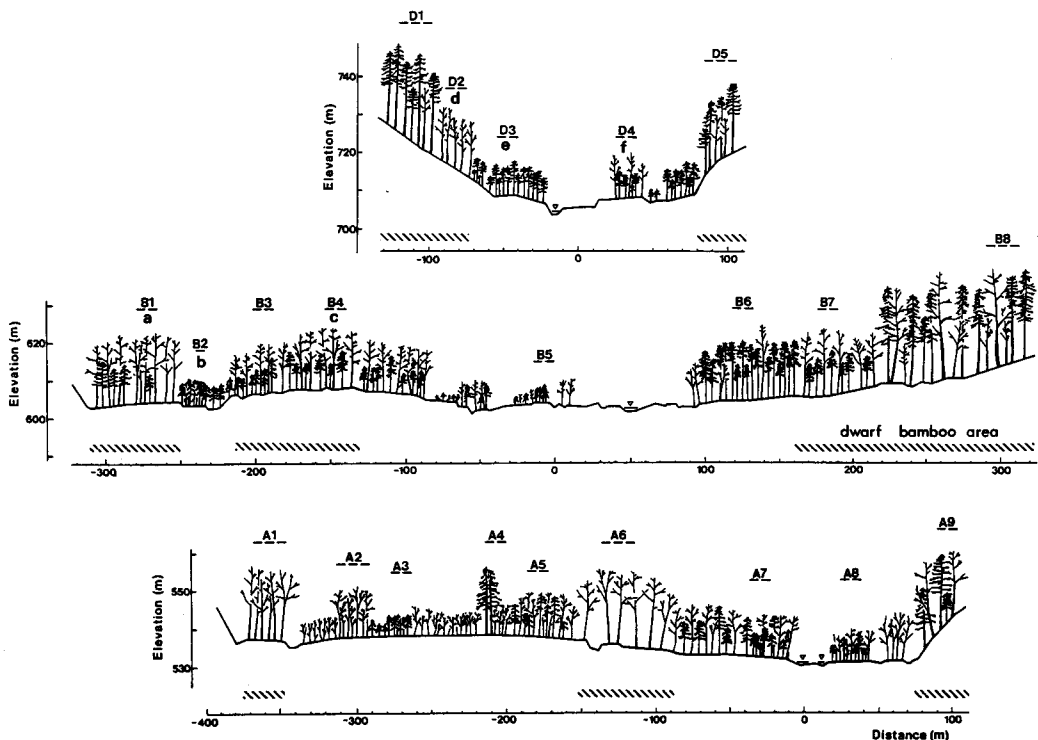
Fig. 3 Cross-sectional views of landforms and forest stands in the lines A, B and D with location of investigated sites (Fig. 2). These diagrams were drawn by looking upstream at the cross-sections.
