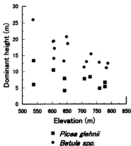
Fig. 6 Relationships between elevation and dominant height of Betula spp. and Picea glehnii stands. Only a correlation coefficient for Betula spp. stands is significant ( p < 0.01 ).
