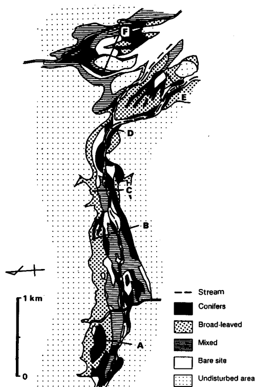
Fig. 4 Regenerated forest stands interpreted by aerial photographs. Elongated patches of classified stands were distributed parallel to the mudflow direction.
