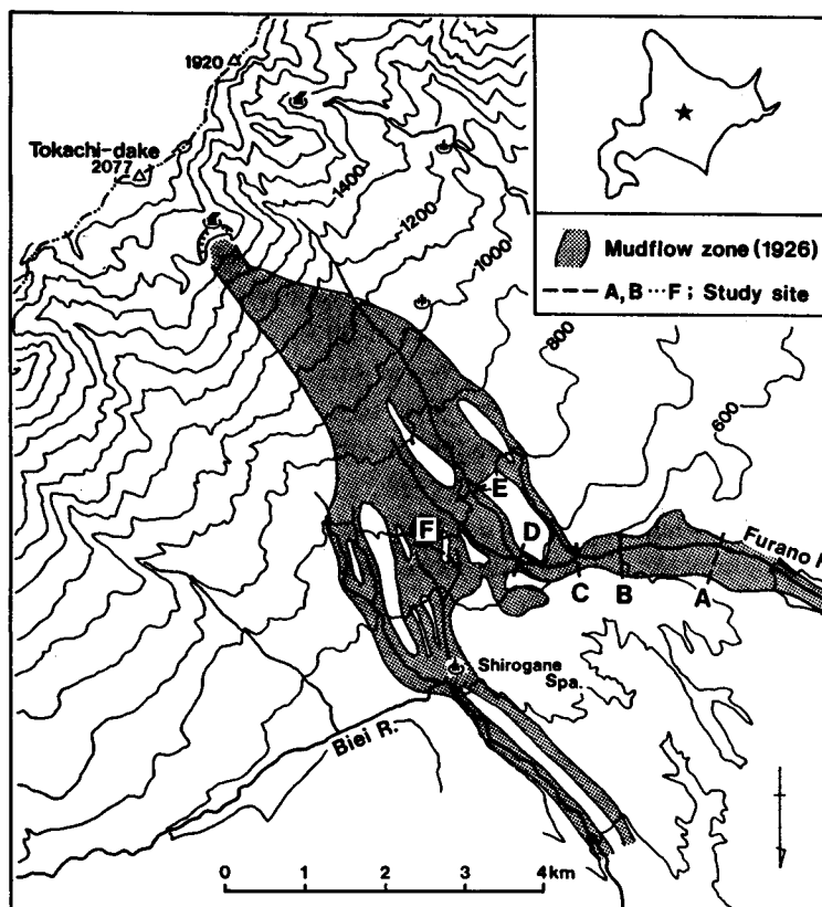
Fig. 1 The 1926 mudflow zone and study sites at Mount Tokachi Volcano.
