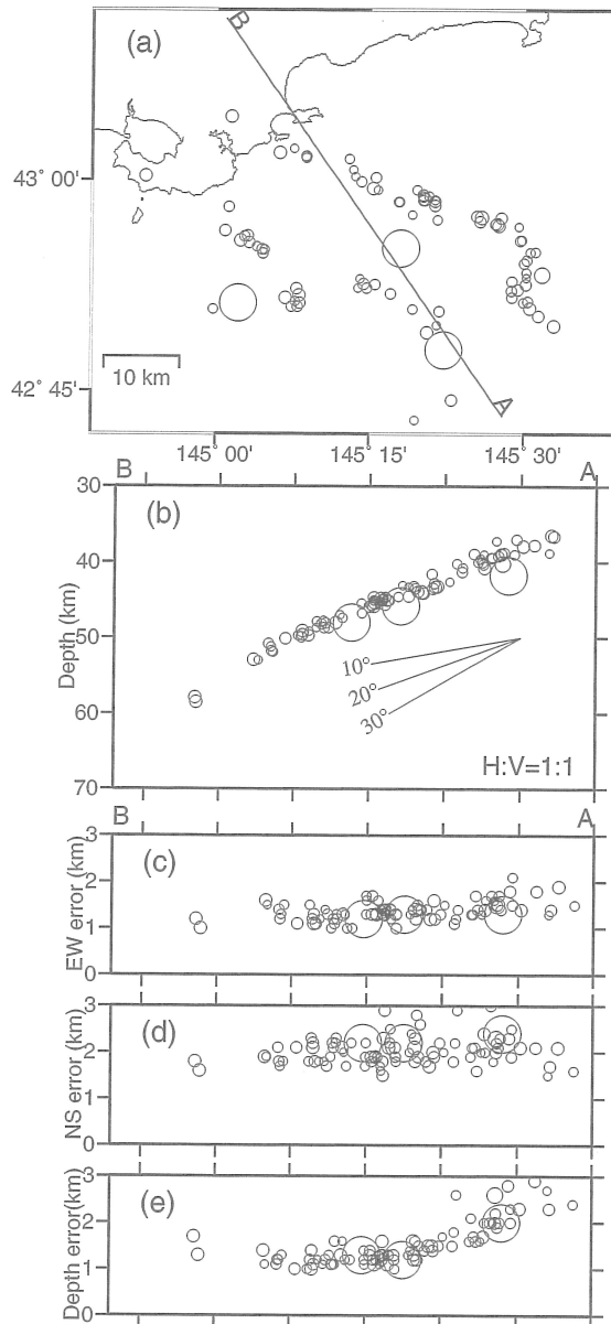
Fig. 9. Aftershocks of the 29 November 2005 Kushiro-Oki earthquake relocated by using three-dimensional velocity structure based on Data set 2. The time period is from 29 November 2004 to 29 January 2005, and the magnitude is 3.5 or larger. (a) Map view and (b) vertical cross section along the line A-B in (a). (c)-(e) The location errors defined in the section 3.3 in this paper.
