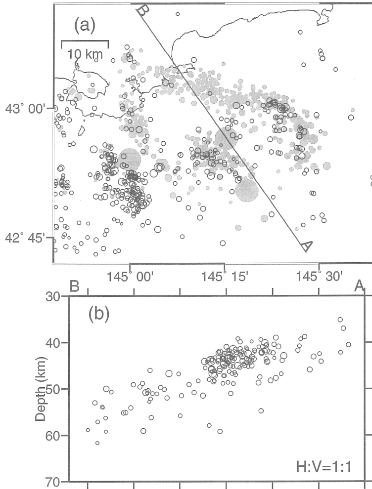
Fig. 8. Background seismicity from 1 January 2002 to 28 November 2004 (open circles) and the aftershocks of the 29 November 2004 Koshiro-Oki earthquake (gray circles). (a) Map view and (b) vertical cross section along the line A-B in (a). Note that the aftershocks were not plotted on (b).
