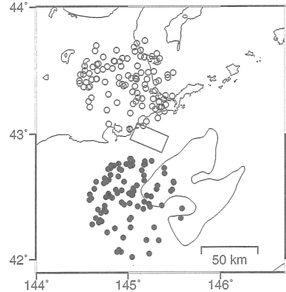
Fig. 13. Aftershock area, asperity, and change in seismicity rate. Earthquakes within the Pacific plate has been suffered from the seismic quiescence (open circles) and the seismic activation (closed circles) since May 2000 (Katsumata and Kasahara, 2004). A rectangle indicates the area ruptured by the main shock on 29 November 2004, which is same as that in Fig. 11. A contour of 1 m represents the asperity ruptured by the 1973 Nemuro-Oki earthquake determined by Yamanaka and Kikuchi (2002).
