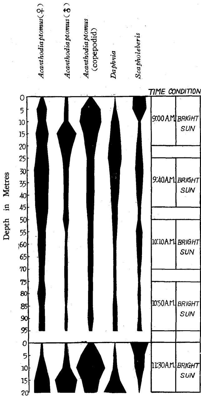
Fig. 2. Vertical distribution of plankton crustaceans in daytime under bright sun on August 15th, 1943, in the deep water of Lake Shikotsu (Observation 2)
