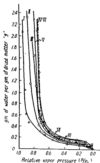
Fig. 15-1. "g— p/p_0 " curves of Stichopus japonicus meat immersed in NaCl solution of various concentrations
