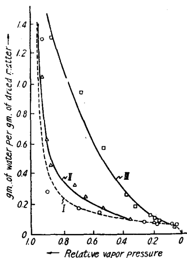
Fig. 16-1. “ g-p/p_0 ” curves of raw meat, meat immersed in water and boiled meat of Stichopus japonicus
