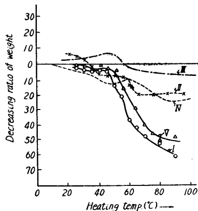
Fig. 11-1. Dehydrating curves of Stichopus japonicus and other fish meat
