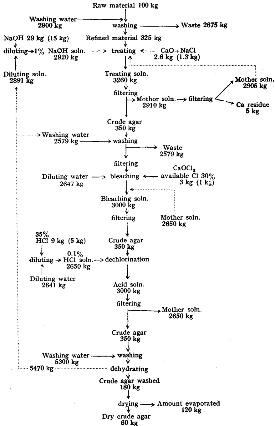
Flow diagram of crude agar manufacture from G. verrucosa (Kojima et al. , 1952)
