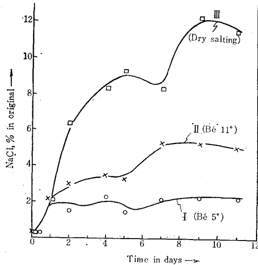
Fig. 33-b. The variation of the amount of NaCl ( S ) in the original samples during the salting
