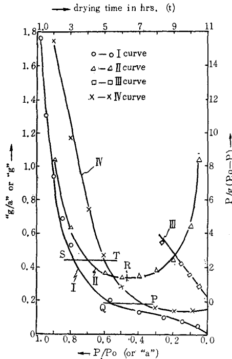
Fig. 12. Atka mackerel meat
