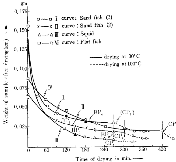
The amount of Bound water per gm of dried matter
