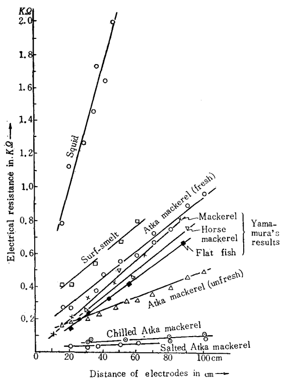
Fig. 5. Relation between the electrical resistance at 50 cycles and the distance of electrodes for various kinds of fish meat (Temp., 15°~16°C)
