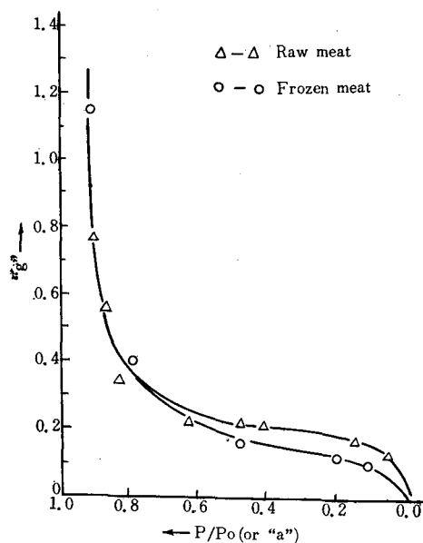
Fig. 24. "g-a" curves for the fresh raw and frozen Atka mackerel meat
