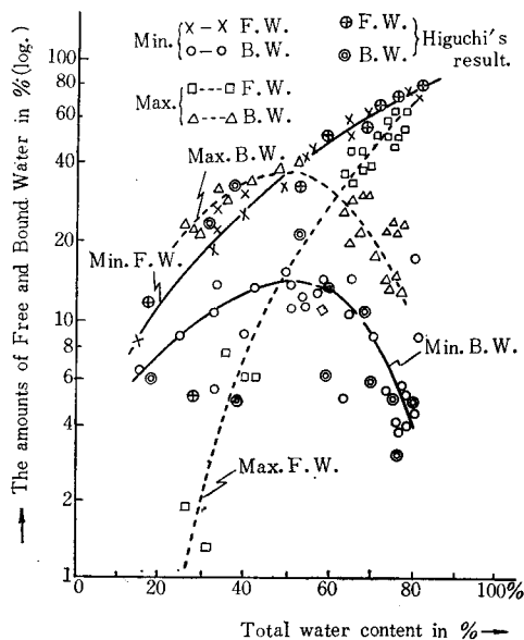
Fig. 2. Variation of the amounts of Free (F.W.) and Bound Water (B.W.) in the course of drying
