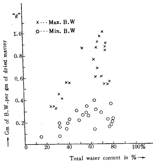
Fig. 3. Distribution of the absolute amount of Bound Water in the course of drying
