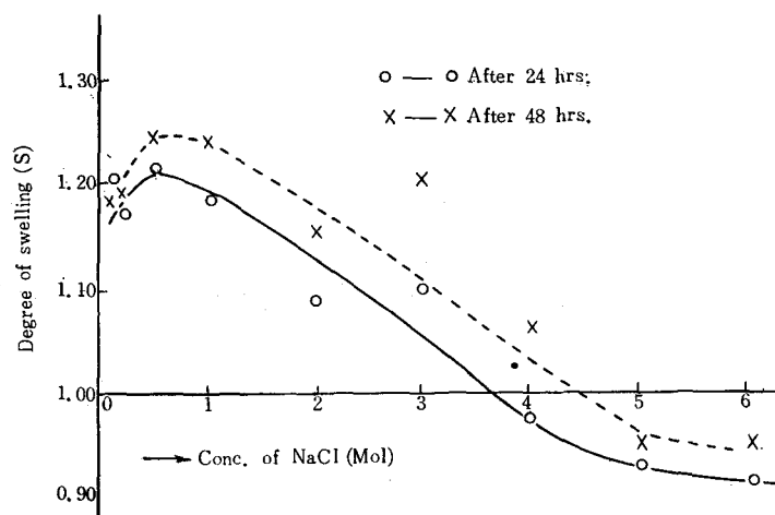
Fig. 29. "Conc.—S" curve for Atka mackerel meat in NaCl solution
