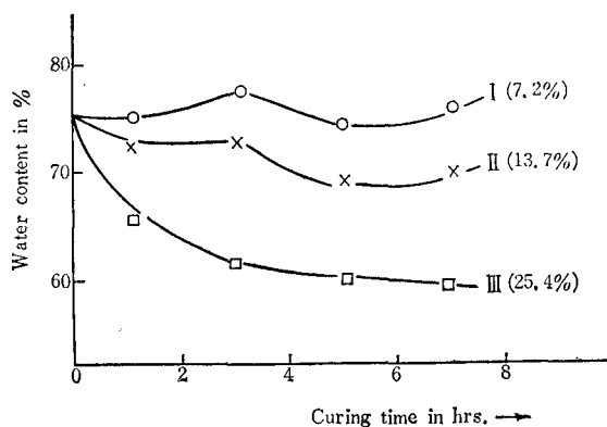
Fig. 32-a. The variation of the amount of water-content ( m ) during the salting
