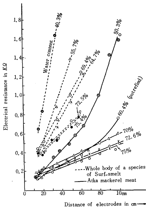
Fig. 6. Relation among the electrical resistance (50 cycles), the distance of the electrodes and the total water-contents in fish meat in various conditions
