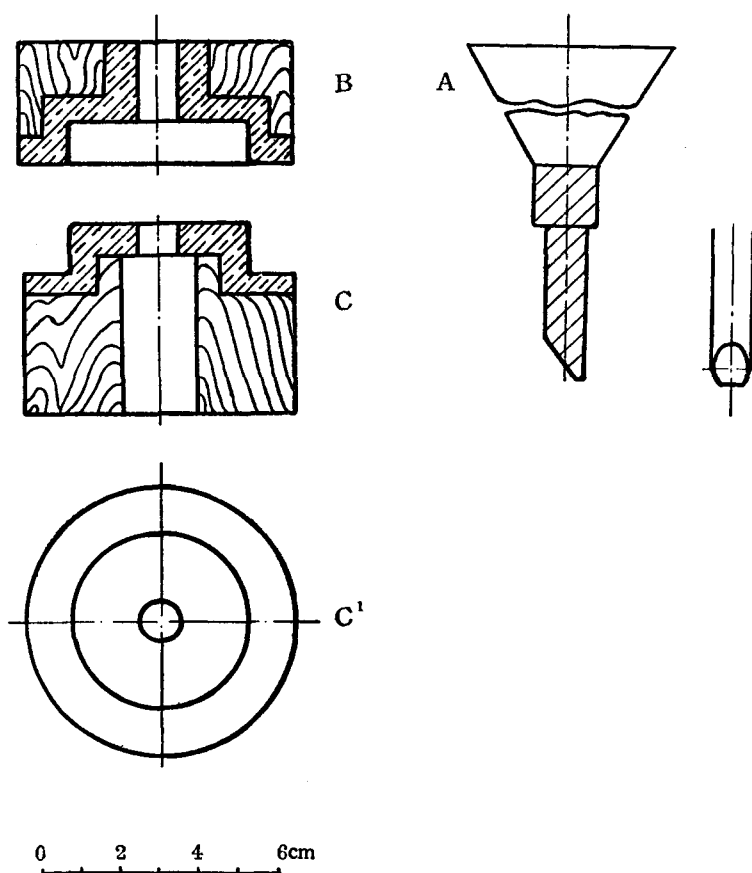
Fig. 7. Device for measuring shearing force
