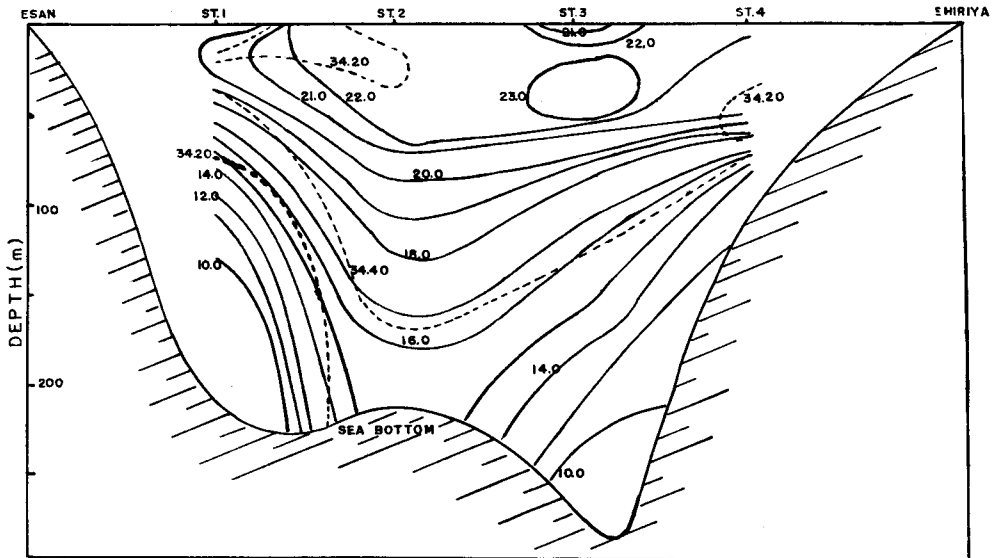
Fig. 24. Vertical section of water temperature and salinity in the water between Esan and Cape Shiriya in September 1960. — water temperature, - - - salinity
