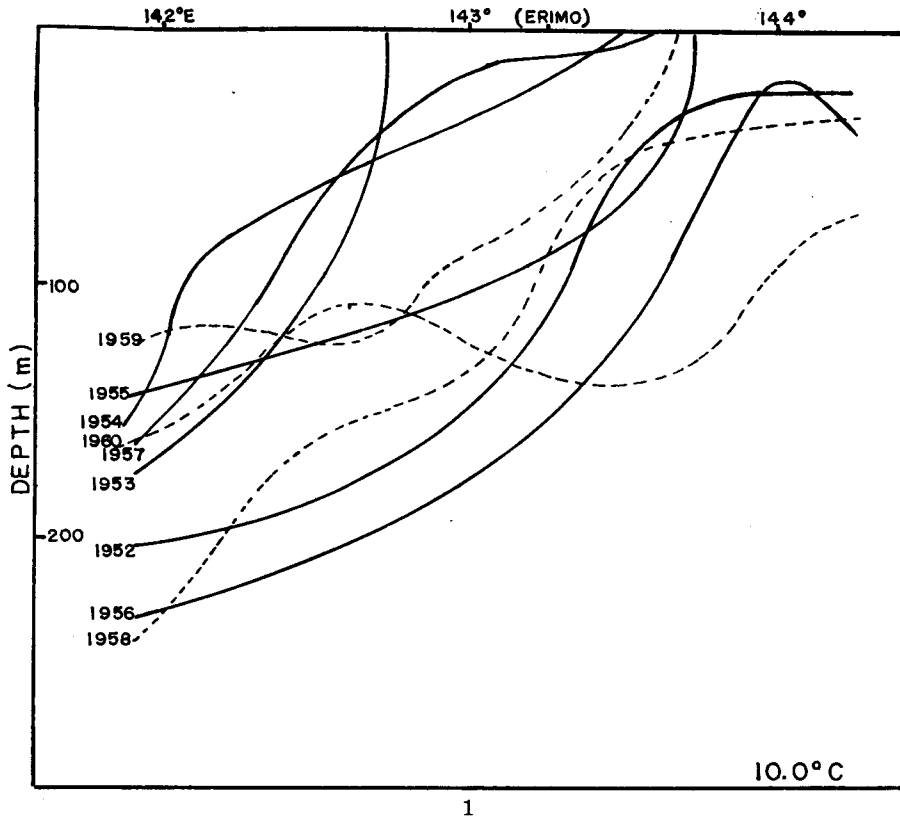
Fig. 44-1. Vertical distributions of isotherms of water temperatures 10°C and 12°C in the sea east off Cape Shiriya (Lat 41°-26'N) in November 1952-1960
