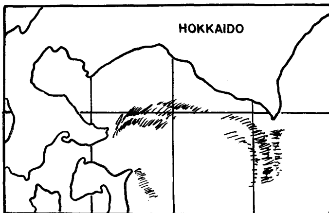
Fig. 30. Rough air sketches of current rips in southeastern waters off Hokkaido
