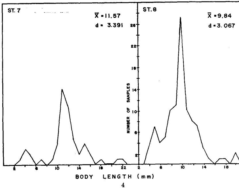
Fig. 41, 3-4. Body length composition of Euphausia pacifica collected from DSL in the sea adjacent to Cape Erimo, August 1960
