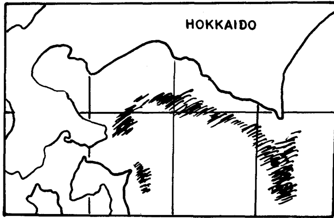
Fig. 34. Distribution of DSL in southeastern waters off Hokkaido
