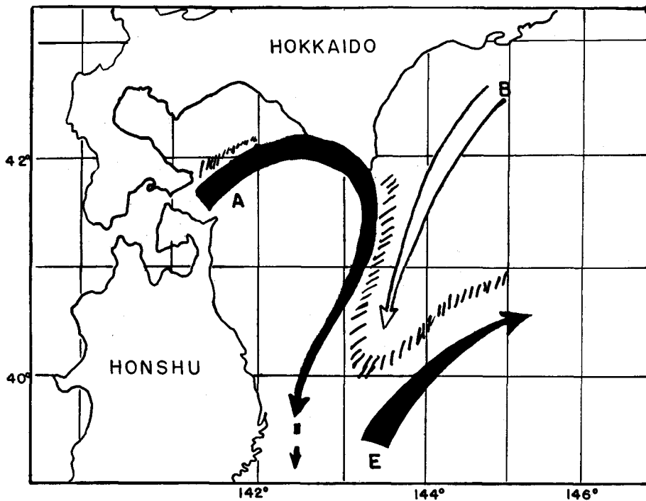
Fig. 14. Schematic representation of the hydrographic conditions near the Tsugaru Warm Current zone (Type D—Flowing southward type No. 2). A—Tsugaru Warm Current, B—Coastal Branch of the Oyashio, E—Warm water masses in the Transition Area
