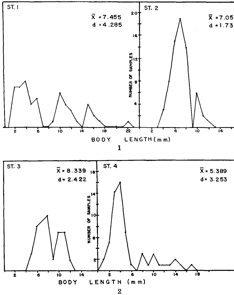
Fig. 41, 1-2. Body length composition of Euphausia pacifica collected from DSL in the sea adjacent to Cape Erimo, August 1960
