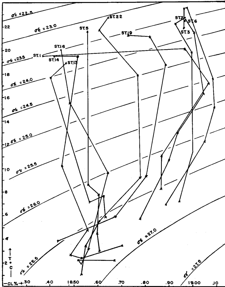
Fig. 26. T-Cl diagram in the southeastern regional waters of Hokkaido in September 1960
