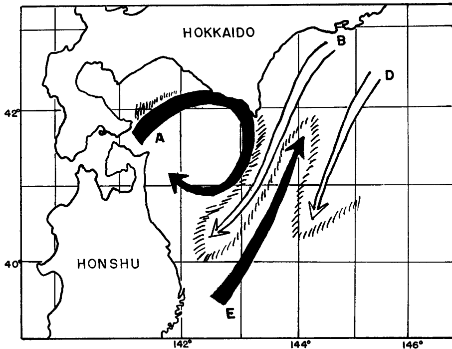
Fig. 12. Schematic representation of the hydrographic conditions near the Tsugaru Warm Current zone (Type B—Stagnating type No. 2). A—Tsugaru Warm Current, B—Coastal Branch of the Oyashio, C—Oyashio, D—Oyashio, E—Warm water masses in the Transition Area
