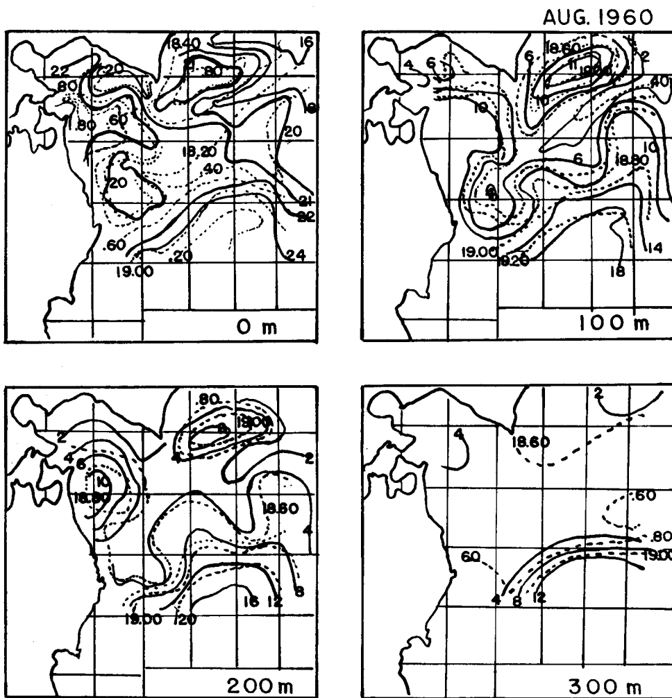
Fig. 28. Horizontal distribution of water temperature and chlorinity at surface, 100 m, 200 m and 300 m depths in August 1960. — water temperature, ---- chlorinity
