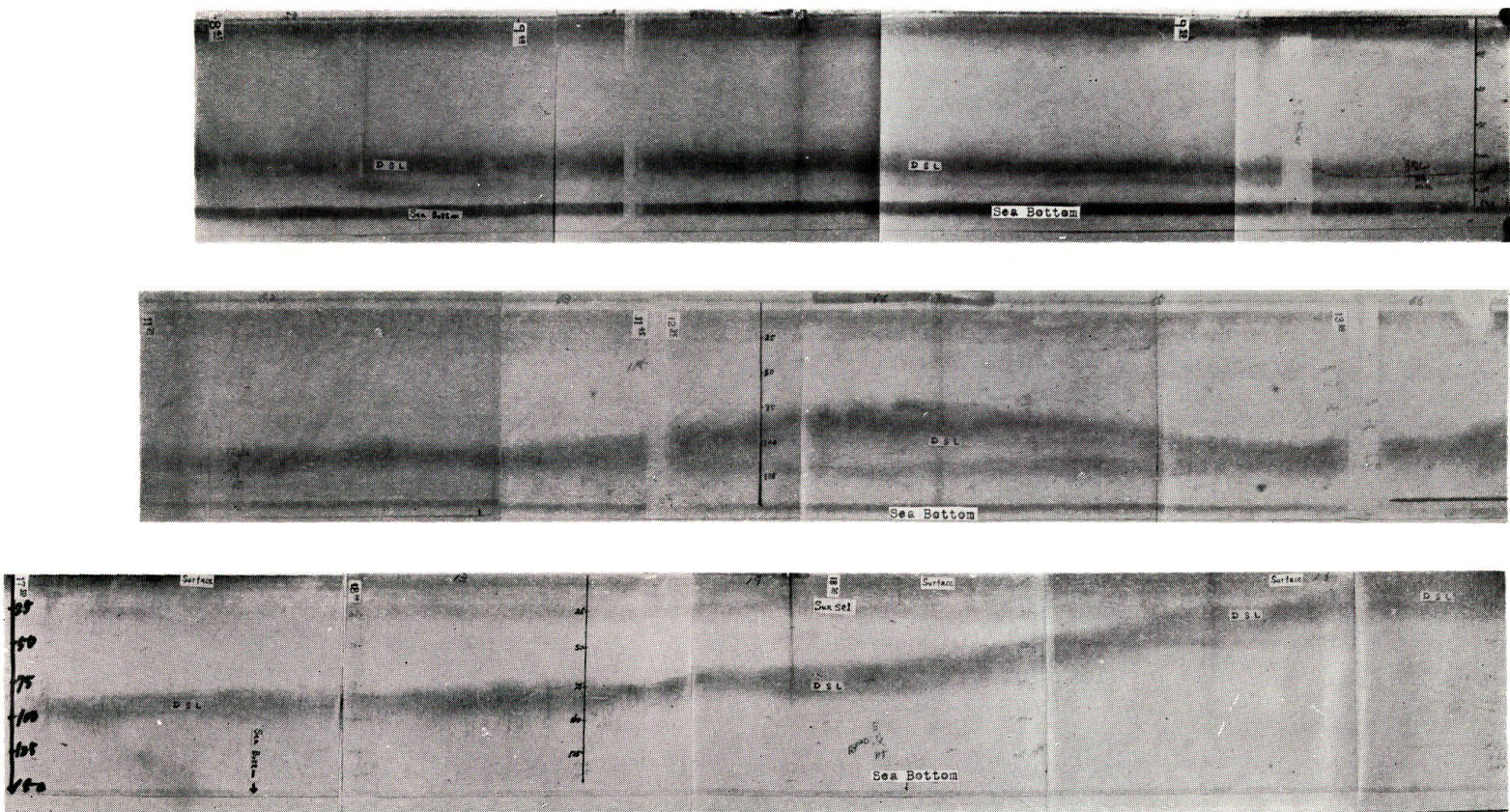
Fig. 33. Echo-image of DSL in the hours 8.00-19.00 in the sea adjacent to Cape Erimo in August 1961
