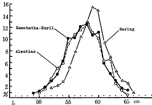
Fig. 5-14. Frequency distribution of oceanic 3+ group sockeye salmon by the area (1960)
