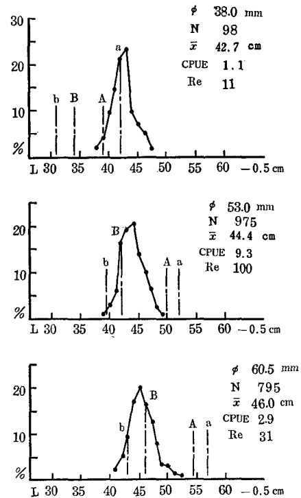
Fig. 5-4. Relation between length composition of the catch and the selective range of the mesh, of pink salmon by mesh " \phi ", size of mesh; N, number of sample; \bar{x} , mean length; CPUE, catch per "tan"; A-B, a-b, selective range of mesh and its limits Catch data by the Oshoro Maru (1957)
