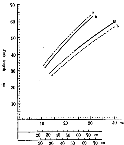
Fig. 4-8. Relationship between "L" and " \phi " of pink salmon
