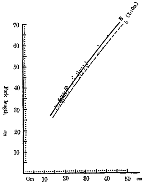
Fig. 4-3. Relationship between "L" and "G m " of sockeye salmon
