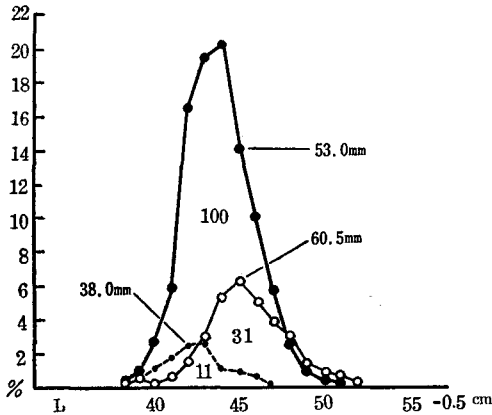
Fig. 5-5. Length composition of the catch by mesh located by the relative efficiency ( R_e ) of each mesh of pink salmon \phi , size of mesh R_e , Relative efficiency of meshes (53,0 mm...100) Data by the Oshoro Maru (1957)
