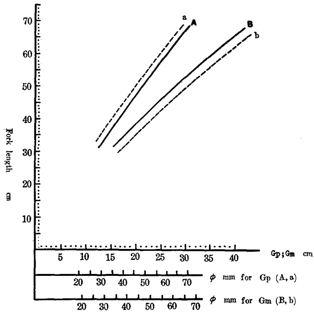
Fig. 4-6. Relationship between "L" and "phi" of chum salmon
