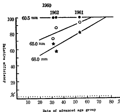
Fig. 6-4. Relation between rate of advanced age group and relative efficiency of three mesh, in chum salmon
