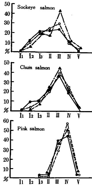
Fig. 4-1. Percentage of catch, by mesh and by division in Fig. 3-1
