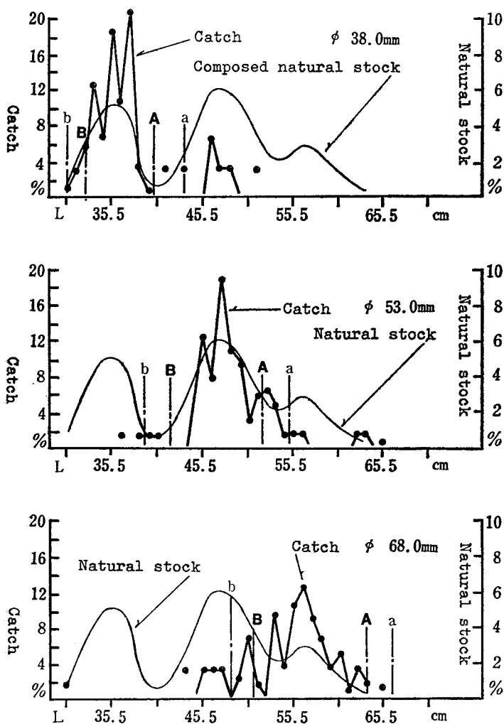
Fig. 5-1. Gill net selection from natural stock by various mesh, of sockeye salmon Original data by the Oshoro-maru (1957)
