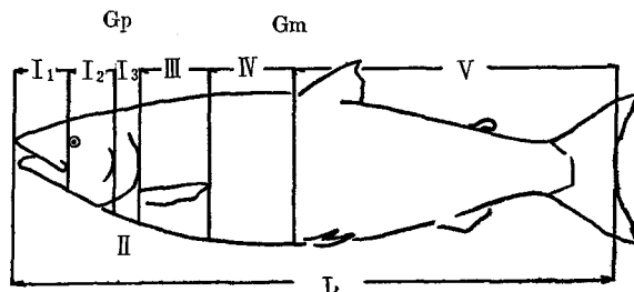
Fig. 3-1. Parts of the body
