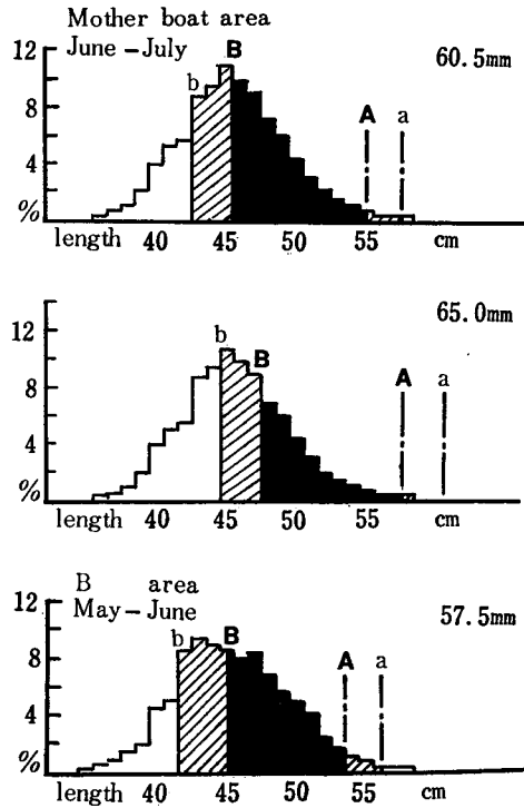
Fig. 5-23. Fishing efficiency by mesh, in each pink salmon groups
