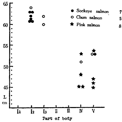
Fig. 5-7. Relation between length of net-marked salmon and the part where it was gilled
