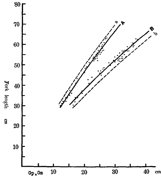
Fig. 4-5. Relationship between "L" and "G p ", "L" and "G m " of chum salmon
