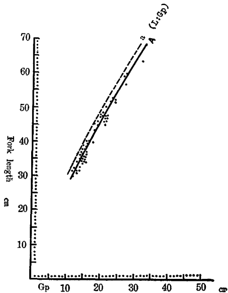
Fig. 4-2. Relationship between "L" and "G p " of sockeye salmon
