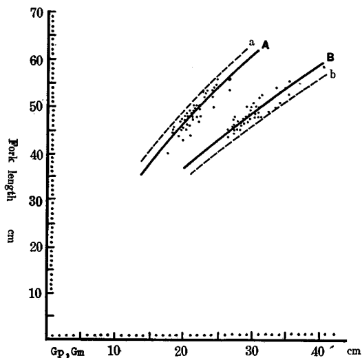
Fig. 4-7. Relationship between "L" and "G p ", "L" and "G m " of pink salmon
