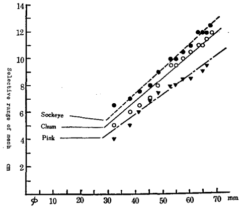
Fig. 5-6. Relationship between size of mesh ( \phi ) and selective range of mesh ( S_r ) by species
