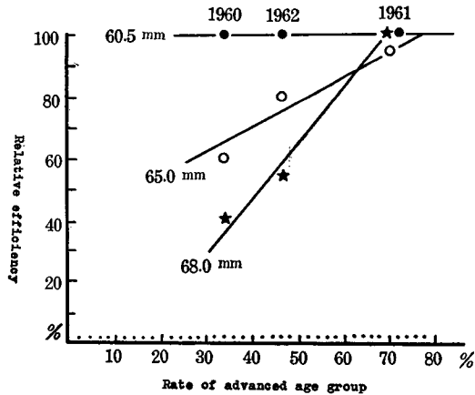
Fig. 6-2. Relation between rate of advanced oceanic age group and relative efficiency of three mesh, in sockeye salmon
