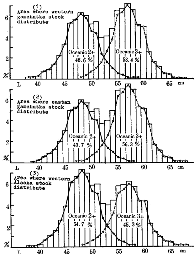
Fig. 6-1. Frequency distribution of available sockeye salmon stock by the area
