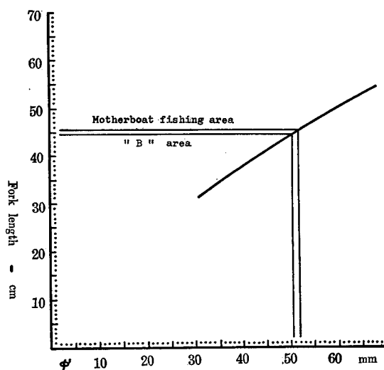
Fig. 5-20. Relationship between fork length and its optimum mesh size ( \phi ) in pink salmon
