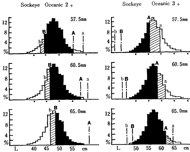
Fig. 5-21. Fishing efficiency by mesh, in each sockeye salmon oceanic age groups
