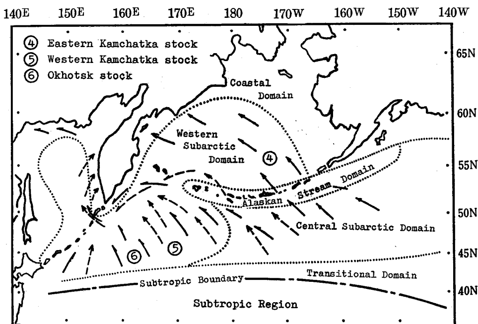
Fig. 2-2. Schematic diagram of distribution and migration of mature chum salmon by local stocks -1
