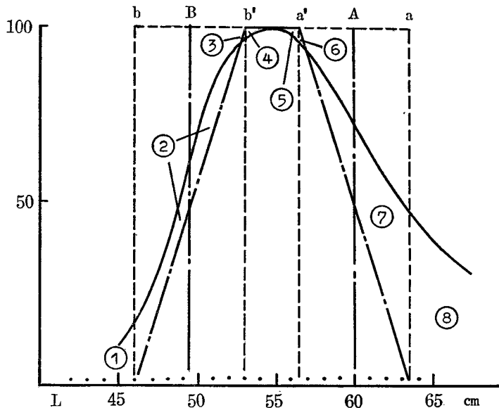
Fig. 5-10. Relation between the selectivity curve (Ishida, 1963) and the selective range of the mesh (in this paper), on chum salmon A-B, the selective range of the mesh (60.5 mm) a-b, the range of variation on L : G_p b-b, the range of variation on L : G_m
