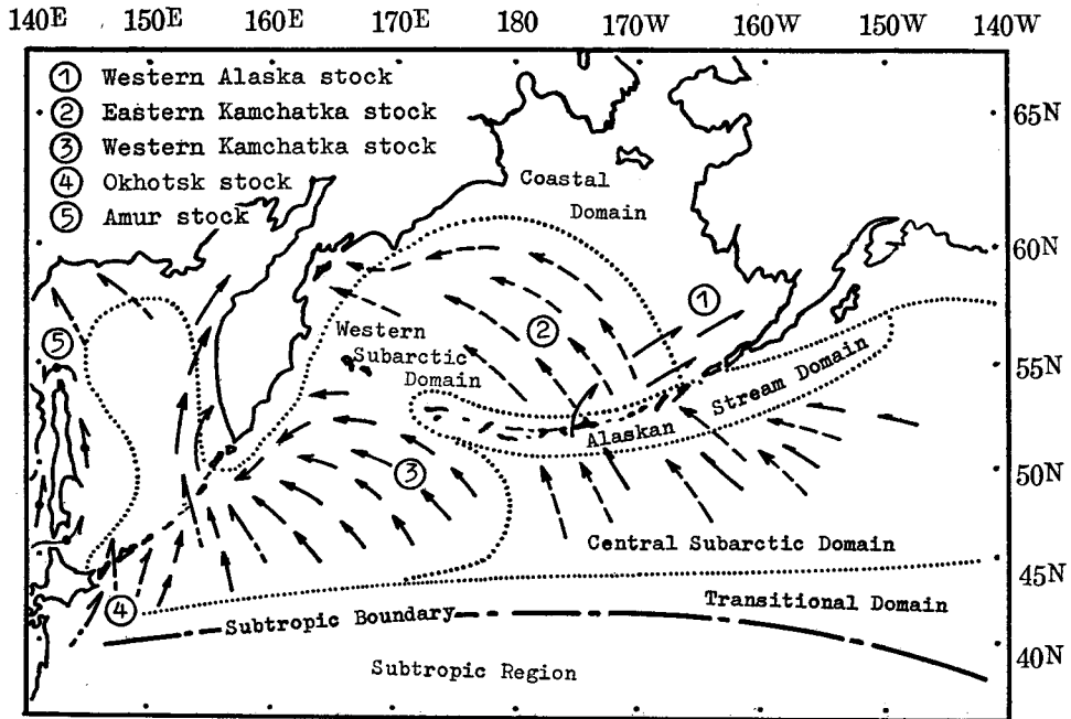
Fig. 2-4. Schematic Diagram of distribution and migration of pink salmon by local stocks
