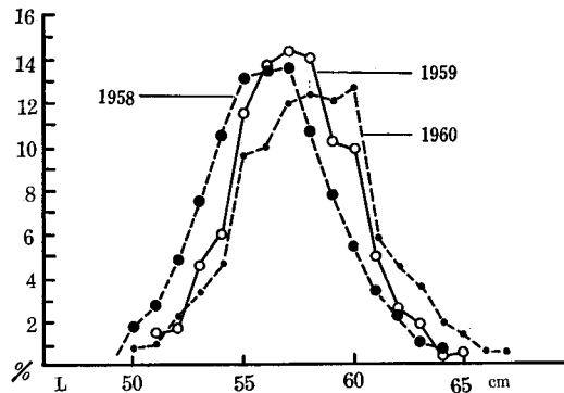
Fig. 5-13. Frequency distribution of fork length of 6_3 sockeye salmon in catch by the year 1958-1960, in the Kamchatka-Kuril area
