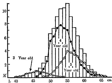
Fig. 6-3. Frequency distribution of available chum salmon stock in the mother boat area
