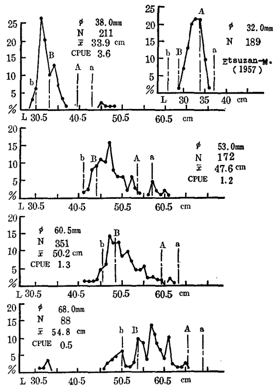
Fig. 5-3. Relation between length composition of the catch and the selective range of the mesh, of chum salmon by mesh " \phi ", size of mesh; N, number of sample; \bar{x} , mean length; CPUE, catch per "tan"; A-B, a-b, selective range of mesh and its limits Catch data by the Oshoro Maru (1957)
