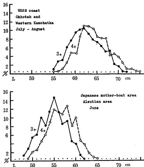
Fig. 5-16. Frequency distribution of fork length of 3+ and 4+ chum salmon in catch, by the area (1961)
