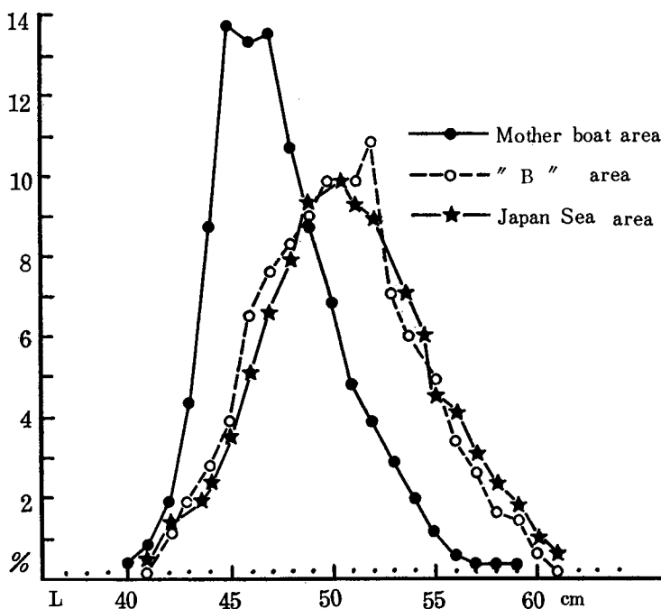
Fig. 5-17. Frequency distribution of fork length of pink salmon caught at USSR coast by the area, correspond to each pelagic distribution
