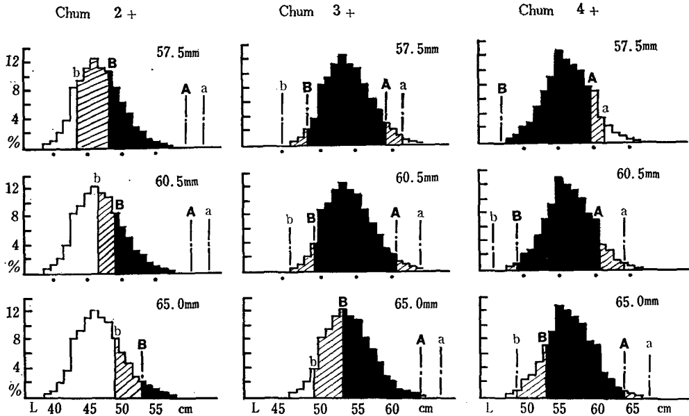
Fig. 5-22. Fishing efficiency by mesh, in each chum salmon age groups
