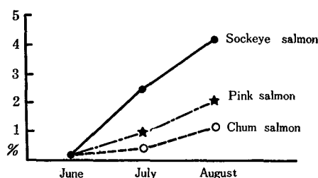
Fig. 2-5. Monthly increase of netmarked fish in the catch
