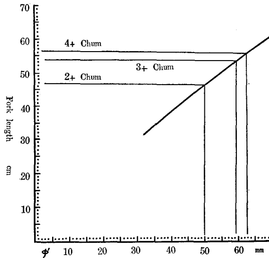
Fig. 5-19. Relationship between fork length and its optimum mesh size ( \phi' ) in chum salmon
