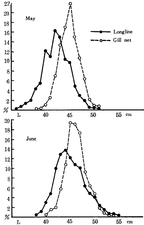
Fig. 5-9. Length composition of pink salmon in "B" area (1962) N, number of sample; \bar{x} , Mean length
