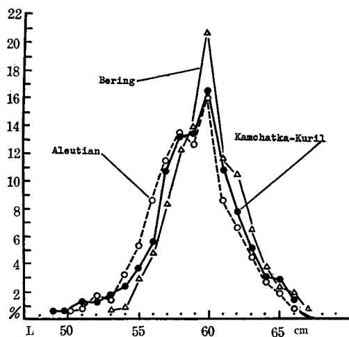
Fig. 5-15. Frequency distribution of fork length of oceanic 3+ group of sockeye salmon by the area (1961)
