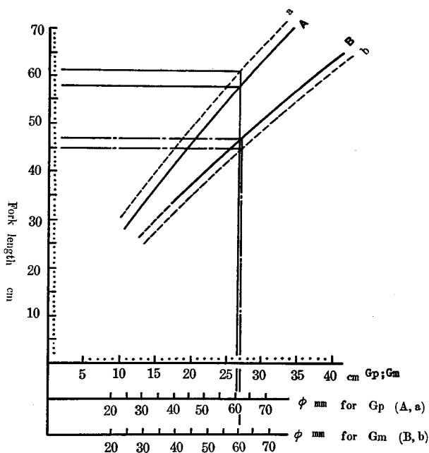
Fig. 4-4. Relationship between “L” and “φ” on sockeye salmon
