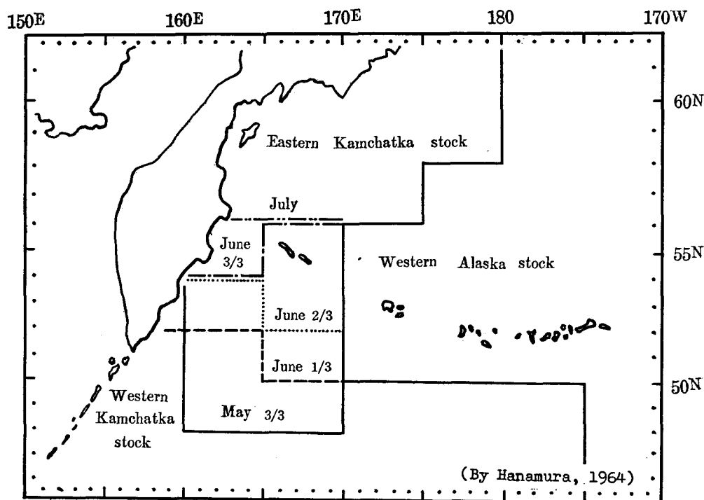
Fig. 3-2. Seasonal variation of sockeye salmon distribution by local stock
