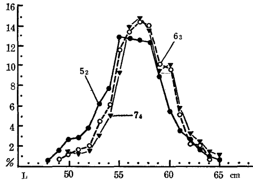
Fig. 5-11. Frequency distribution of fork length of sockeye salmon in catch by age (5 2 , 6 3 , 7 4 , ... Oceanic 3+ group) in the Kamchatka-Kuril area (1959)
