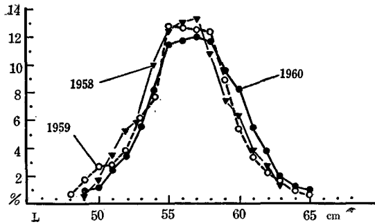
Fig. 5-12. Frequency distribution of fork length of 5 2 sockeye salmon in catch by the year 1958-1960, in the Kamchatka-Kuril area
