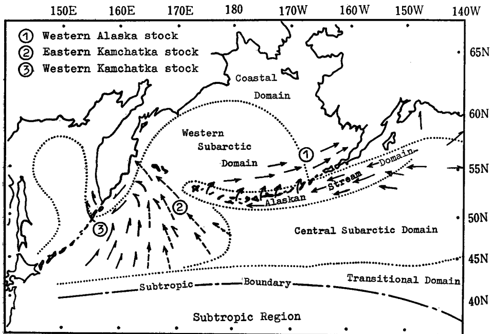
Fig. 2-1. Schematic diagram of distribution and migration of mature sockeye salmon by local stocks
