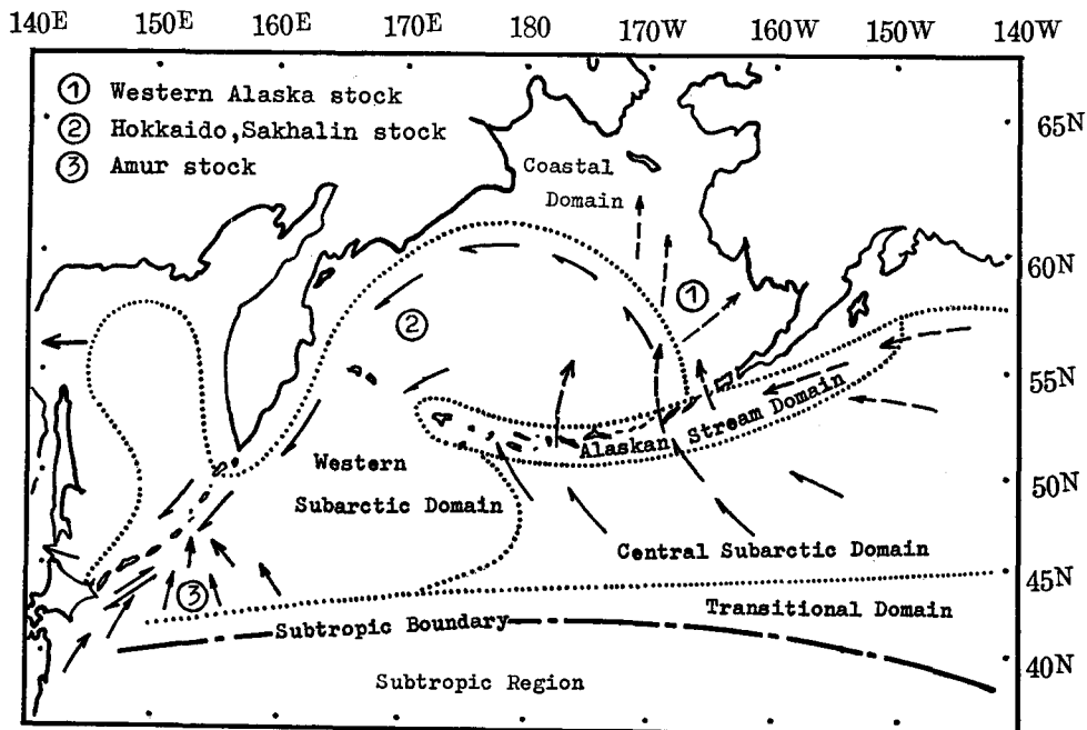
Fig. 2-3. Schematic diagram of distribution and migration of mature chum salmon by local stocks -2
