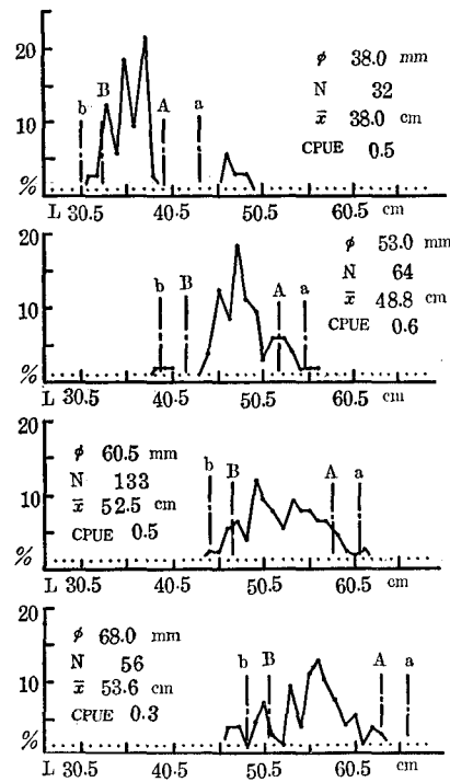
Fig. 5-2. Relation between length composition of the catch and the selective range of the mesh, of sockeye salmon, by mesh " \phi ", size of mesh; N, number of sample; \bar{x} , mean length; CPUE, catch per "tan"; A-B, a-b, selective range of mesh and its limits Catch data by the Oshoro Maru (1957)
