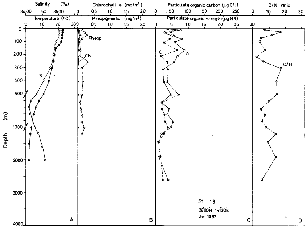
Fig. 17. Profiles of temperature and salinity (A), chlorophyll a and pheopigments (B), P.O.C. and P.O.N. (C), and C/N ratio (D) at St. 19 in the Kuroshio Counter Current, Jan. 1967, Oshoro-Marui Cruise 21.
