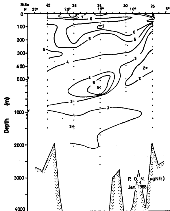
Fig. 10e. Section of particulate organic nitrogen along a 142^{\circ}\text{E} . line from 7^{\circ} to 23^{\circ}\text{N} ., Jan. 1968, Oshoro-Maruru Cruise 26.
