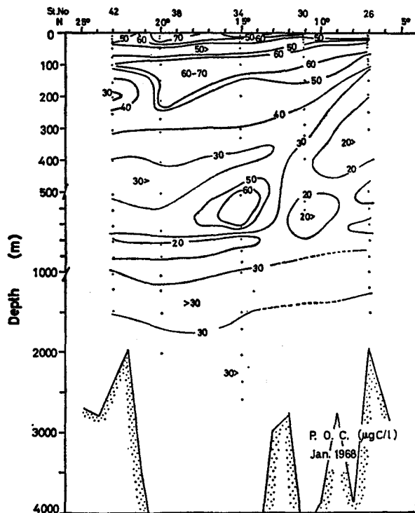
Fig. 10d. Section of particulate organic carbon along a 142^{\circ}\text{E} . line from 7^{\circ} to 23^{\circ}\text{N} ., Jan. 1968, Oshoro-Maruru Cruise 26.
