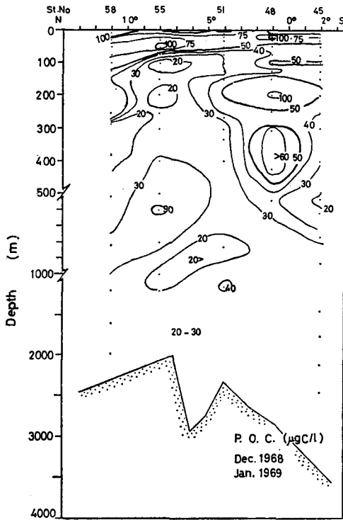
Fig. 11d. Section of particulate organic carbon along a 142°E. line from 2°S. to 11°N., Dec. 1968 to Jan. 1969, Oshoro-Maruru Cruise 30.
