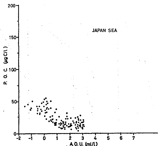
Fig. 34e. Relationship between P.O.C. and A.O.U. observed in the Japan Sea (KH-70-4).
