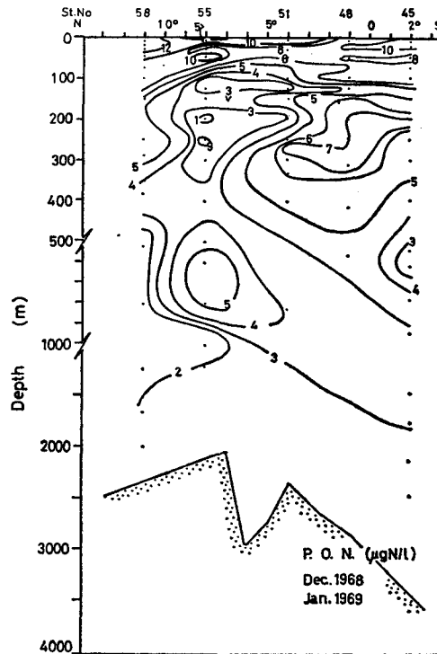
Fig. 11e. Section of particulate organic nitrogen along a 142°E. line from 2°S. to 11°N., Dec. 1968 to Jan. 1969, Oshoro-Maruru Cruise 30.
