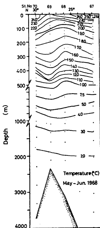
Fig. 12a. Section of temperature along a 132°E. line from 22° to 30°N., May to June 1968, Hakuho-MarU Cruise KH-68-2.
