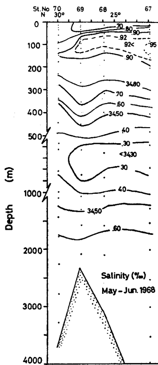
Fig. 12b. Section of salinity along a 132°E. line from 22° to 30°N., May to June, 1968, Hakuho-MarU Cruise KH-68-2.
