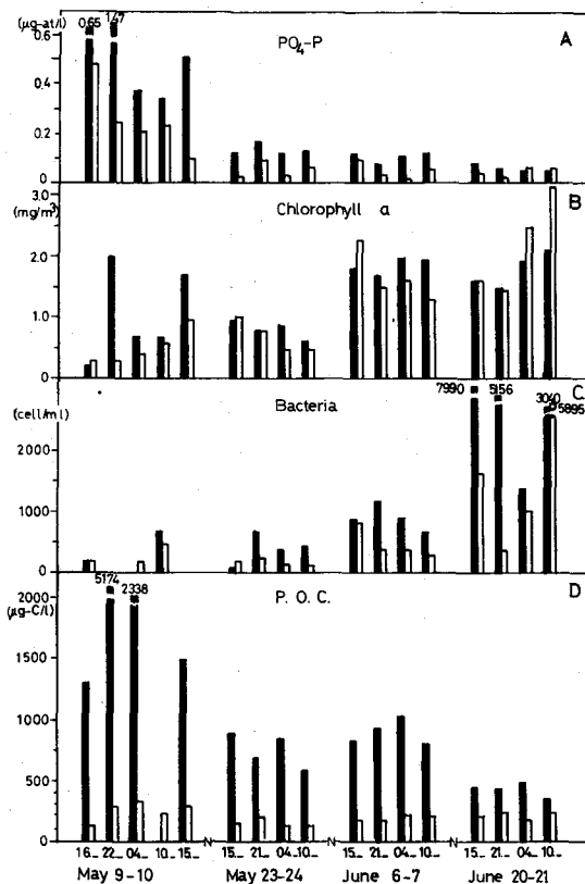
Fig. 32. Monthly variations in concentrations of PO_4 -P (A), chlorophyll a (B), bacterial cell number (C), and P.O.C. (D), in the skin (solid column) and in the subsurface layer (ca. 50 cm. deep, open column) in Oshoro Bay, May to June, 1970.
